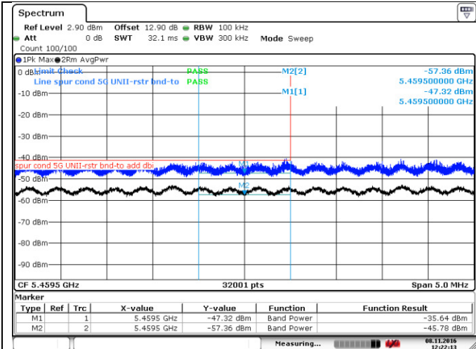
Figure 8.4-50: Lower band edge emission, 802.11ac-VHT80
