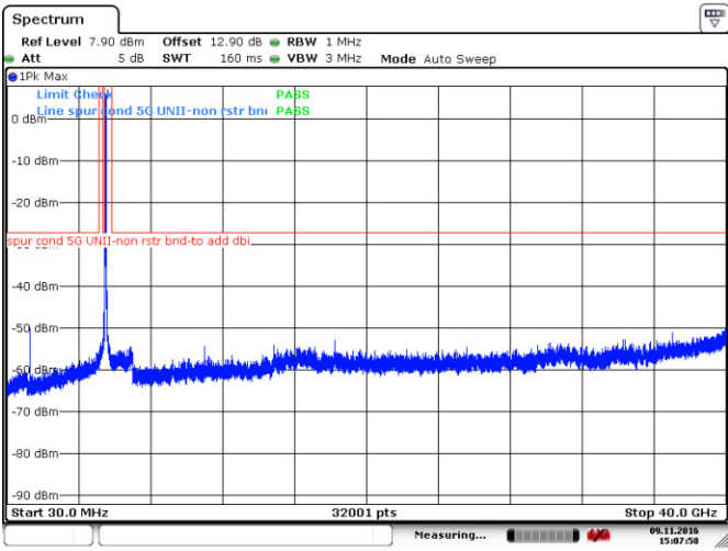
Figure 8.4-24: Peak spurious emissions outside restricted bands at low channel, 802.11n-HT40, ch100
