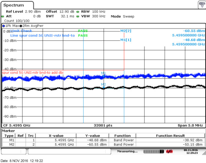
Figure 8.4-43: Lower band edge emission(restricted band), 802.11n-HT40
