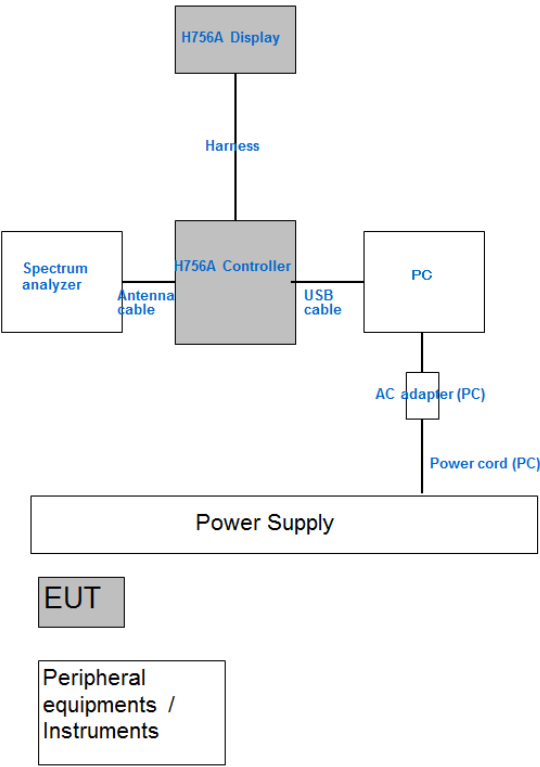
Figure 3.6-1: Setup diagram
