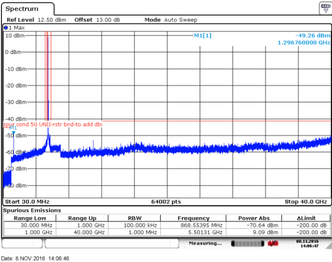
Figure 8.4-10: Peak spurious emissions within restricted bands at low channel, 802.11ac-VHT20, ch100
