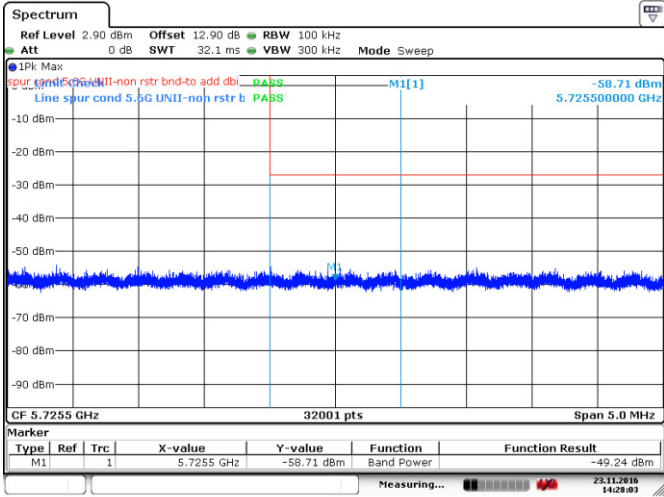
Figure 8.4-51: Upper band edge emission, 802.11ac-VHT80
