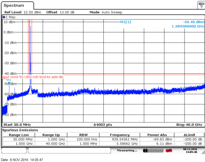
Figure 8.4-8: Peak spurious emissions within restricted bands at mid channel, 802.11n-HT40, ch116
