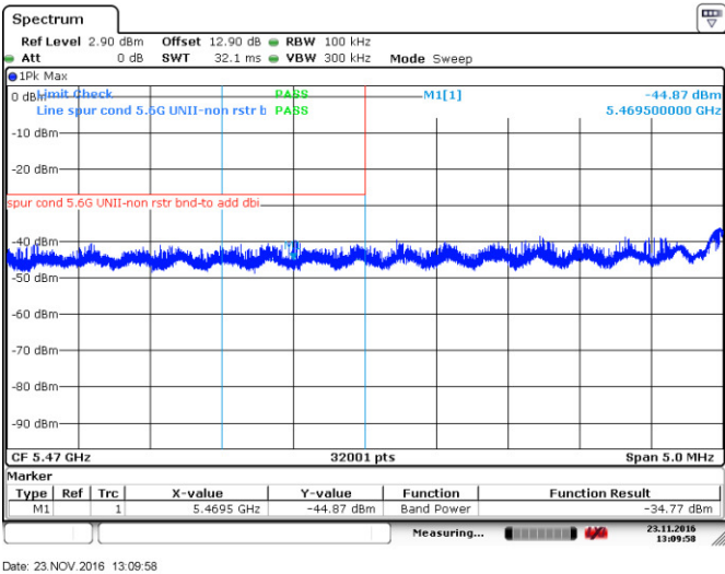
Figure 8.4-41: Lower band edge emission, 802.11n-HT40
