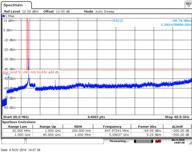
Figure 8.4-11: Peak spurious emissions within restricted bands at mid channel, 802.11ac-VHT20, ch120
