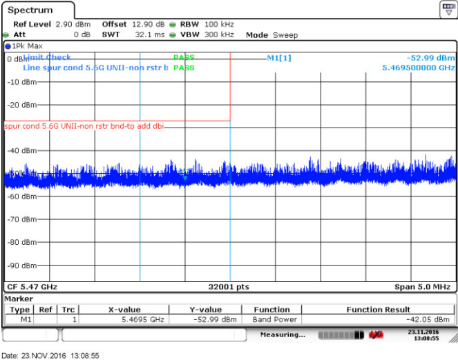
Figure 8.4-38: Lower band edge emission, 802.11n-HT20
