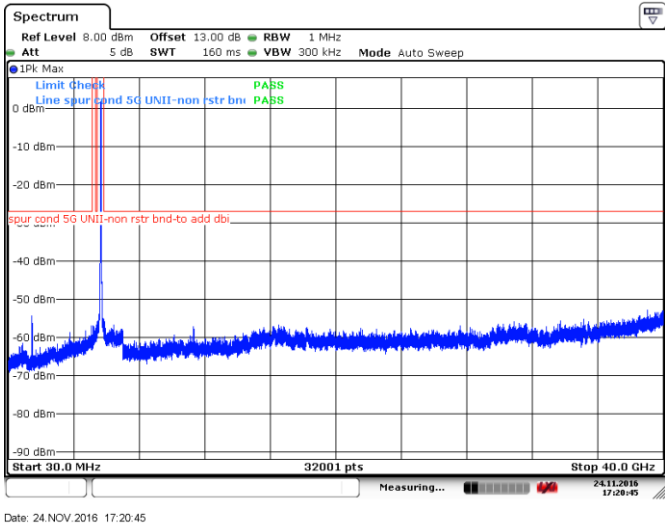
Figure 8.4-32: Peak spurious emissions outside restricted bands at mid channel, 802.11ac-VHT40, ch132
