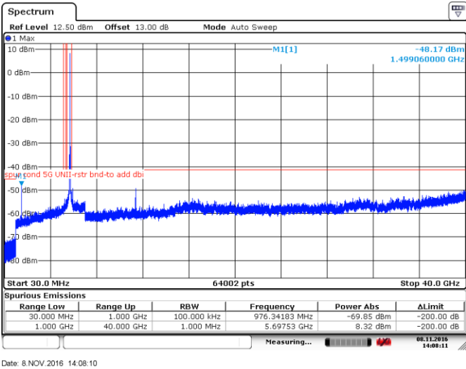
Figure 8.4-12: Peak spurious emissions within restricted bands at high channel, 802.11ac-VHT20, ch140
