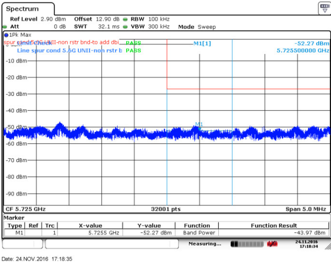
Figure 8.4-42: Upper band edge emission, 802.11n-HT40
