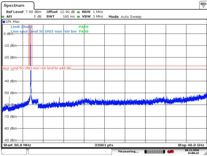
Figure 8.4-25: Peak spurious emissions outside restricted bands at mid channel, 802.11n-HT40, ch116
