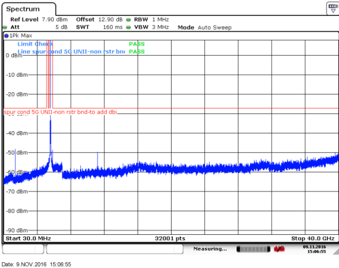
Figure 8.4-22: Peak spurious emissions outside restricted bands at mid channel, 802.11n-HT20, ch120
