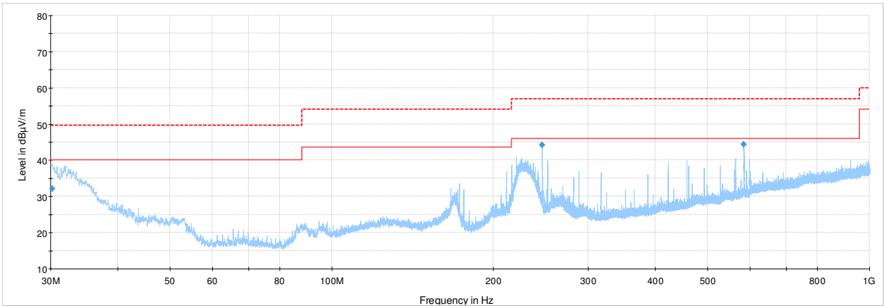
Figure 8.4-56: Radiated spurious emission below 1 GHz sample plot
