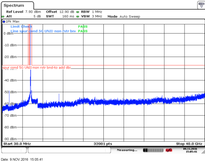
Figure 8.4-19: Peak spurious emissions outside restricted bands at mid channel, 802.11a, ch120
