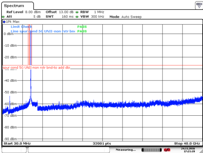
Figure 8.4-26: Peak spurious emissions outside restricted bands at mid channel, 802.11n-HT40, ch132
