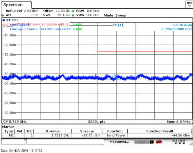
Figure 8.4-48: Upper band edge emission, 802.11ac-VHT40
