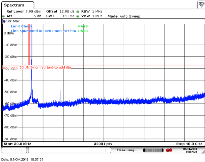
Figure 8.4-23: Peak spurious emissions outside restricted bands at high channel, 802.11n-HT20, ch140
