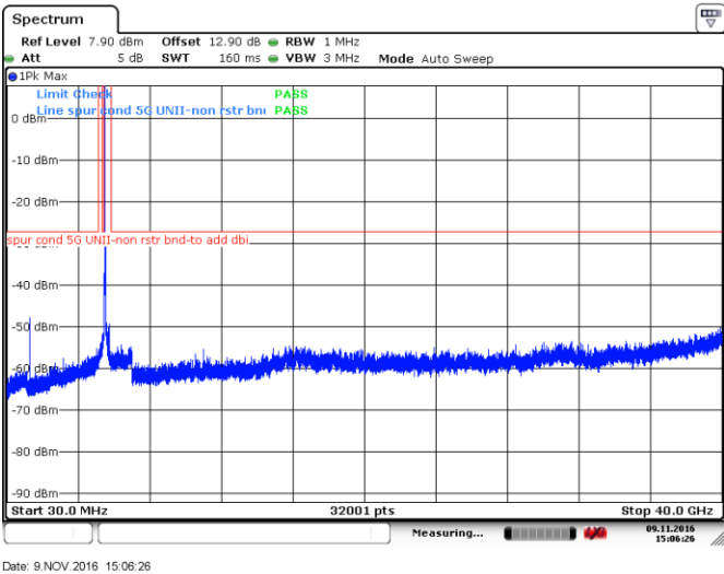
Figure 8.4-21: Peak spurious emissions outside restricted bands at low channel, 802.11n-HT20, ch100
