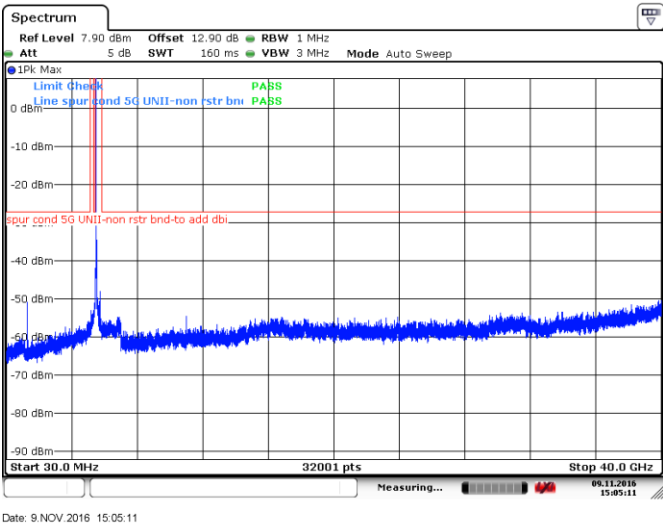
Figure 8.4-18: Peak spurious emissions outside restricted bands at low channel, 802.11a, ch100
