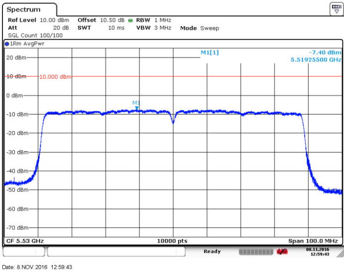
Figure 8.3-6: Sample plot for PSD on 802.11ac VHT80
