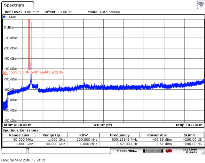
Figure 8.4-15: Peak spurious emissions within restricted bands at mid channel, 802.11ac-VHT40, ch132
