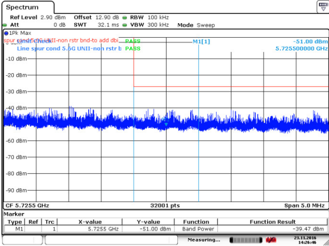
Figure 8.4-45: Upper band edge emission, 802.11ac-VHT20
