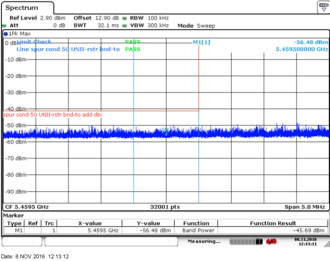
Figure 8.4-40: Lower band edge emission(restricted band), 802.11n-HT20
