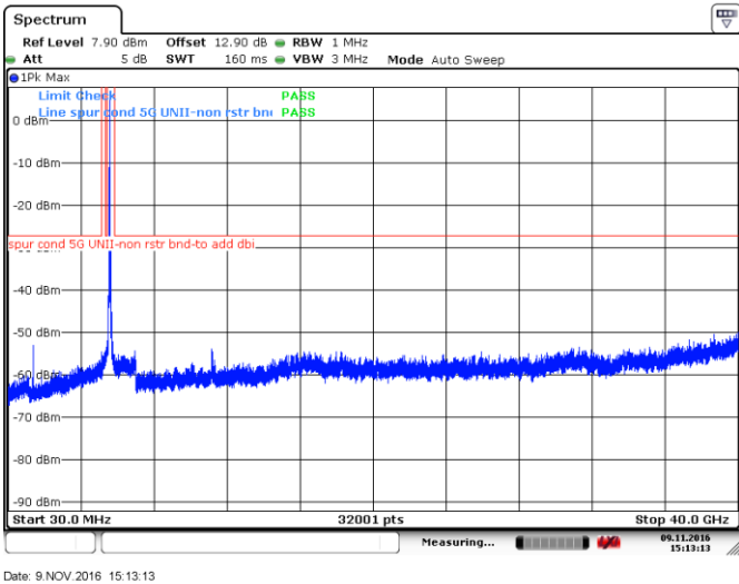
Figure 8.4-31: Peak spurious emissions outside restricted bands at mid channel, 802.11ac-VHT40, ch116
