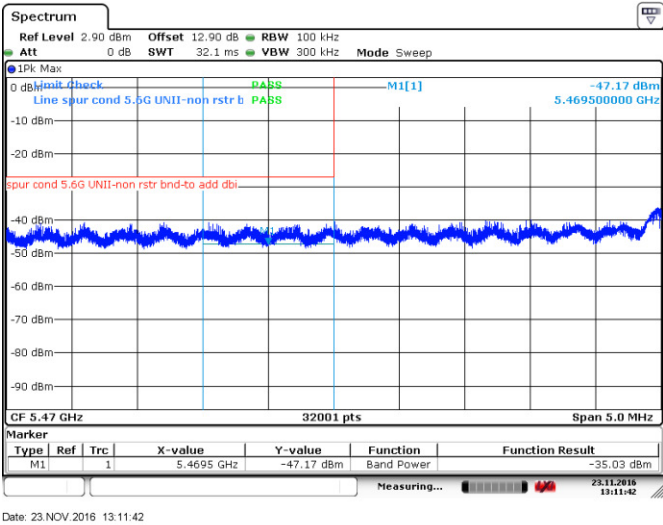
Figure 8.4-47: Lower band edge emission, 802.11ac-VHT40
