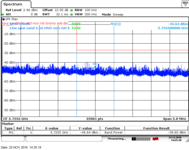
Figure 8.4-39: Upper band edge emission, 802.11n-HT20
