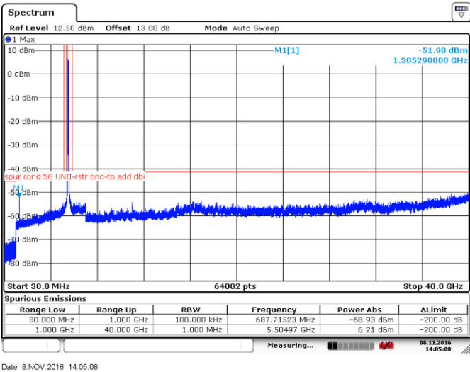
Figure 8.4-7: Peak spurious emissions within restricted bands at low channel, 802.11n-HT40, ch100
