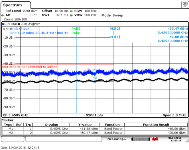
Figure 8.4-49: Lower band edge emission(restricted band), 802.11ac-VHT40
