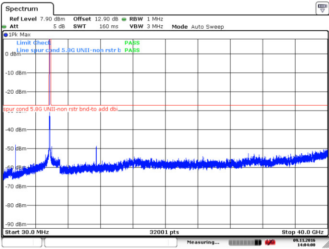
Figure 8.5-18: Peak spurious emissions outside restricted bands at low channel, 802.11n-HT20, ch149
