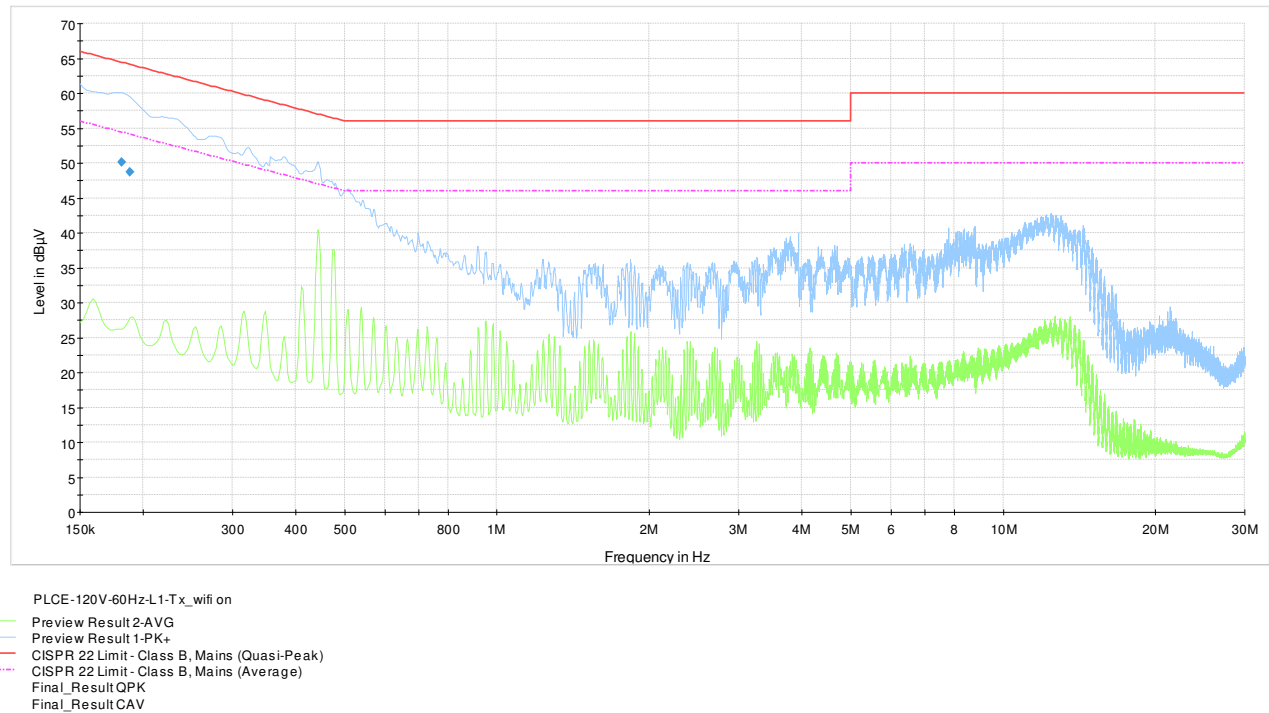
Plot 8.6-1: Conducted emissions on phase line
