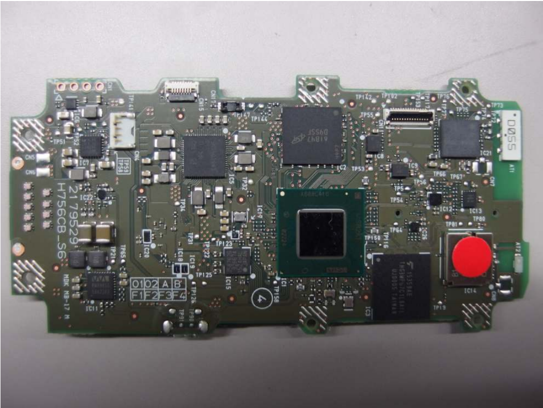
06. CB Board (surface)
