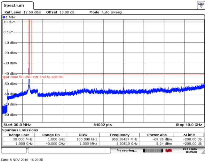
Figure 8.4-13: Peak spurious emissions within restricted bands at high channel, 802.11ac-VHT40, ch60
