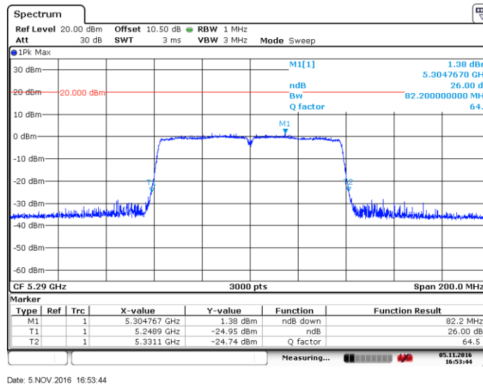
Figure 8.1-3: 26 dB bandwidth on 802.11ac HT80, sample plot
