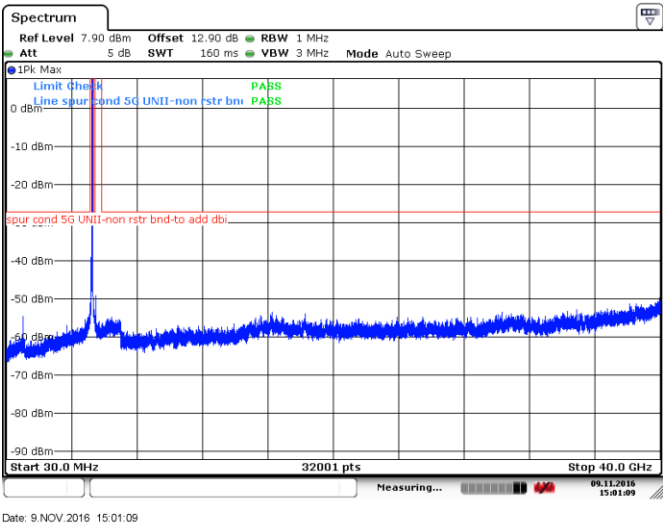
Figure 8.4-23: Peak spurious emissions outside restricted bands at low channel, 802.11ac-VHT20, ch52
