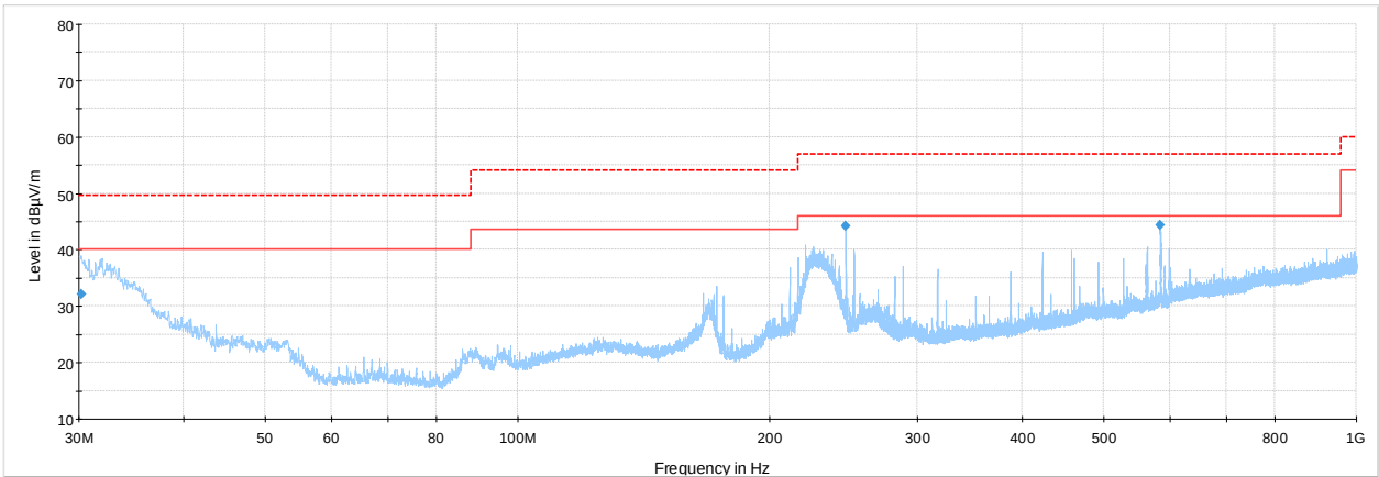
Figure 8.4-44: Radiated spurious emission below 1 GHz sample plot
