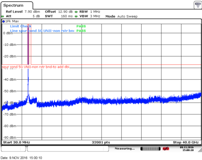
Figure 8.4-21: Peak spurious emissions outside restricted bands at low channel, 802.11n-HT40, ch52
