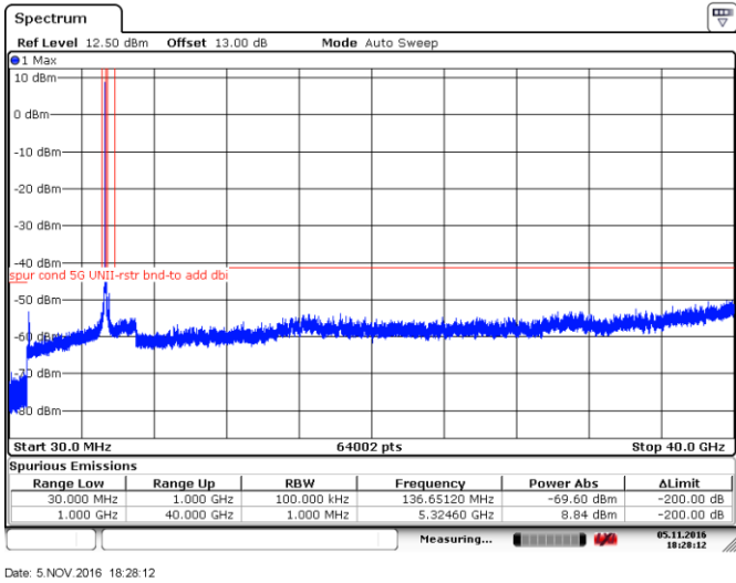
Figure 8.4-11: Peak spurious emissions within restricted bands at high channel, 802.11ac-VHT20, ch64
