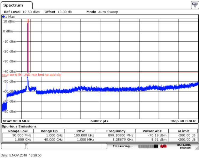
Figure 8.4-9: Peak spurious emissions within restricted bands at low channel, 802.11ac-VHT20, ch52
