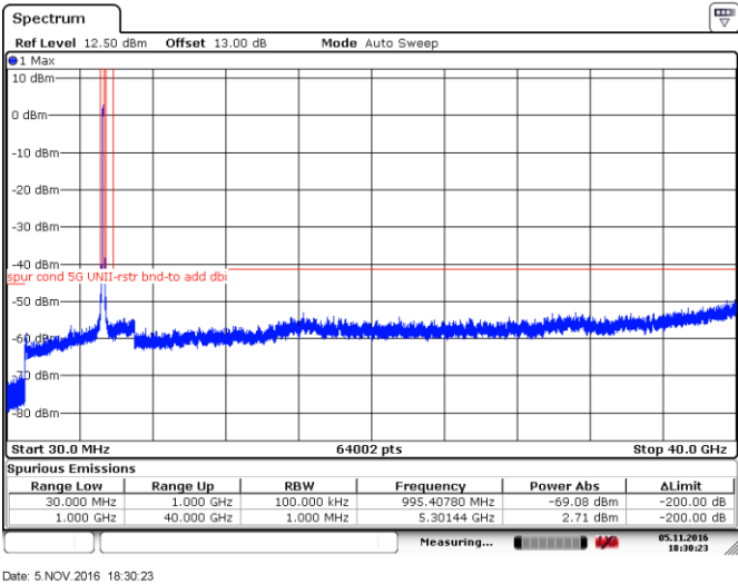
Figure 8.4-14: Peak spurious emissions within restricted bands, 802.11ac-VHT80, ch52
