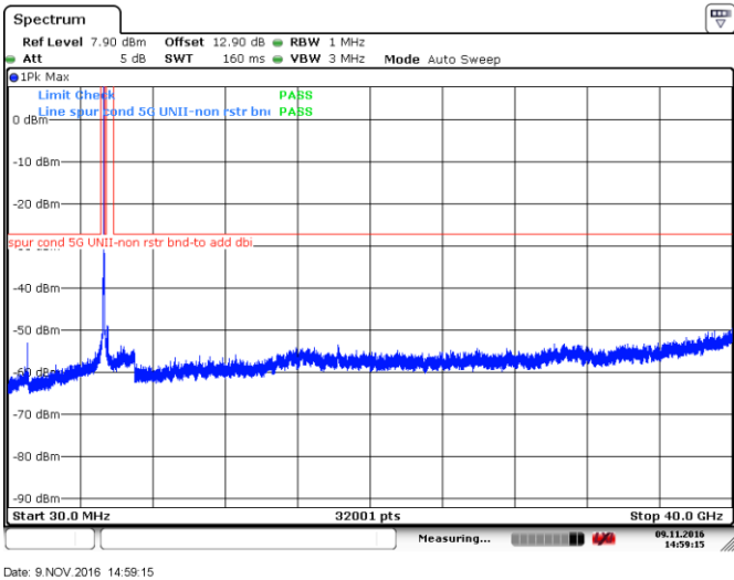
Figure 8.4-19: Peak spurious emissions outside restricted bands at mid channel, 802.11n-HT20, ch60
