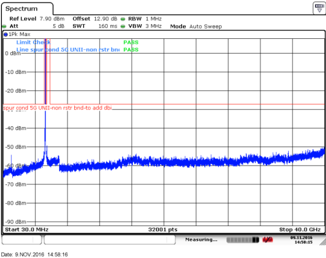
Figure 8.4-18: Peak spurious emissions outside restricted bands at low channel, 802.11n-HT20, ch52
