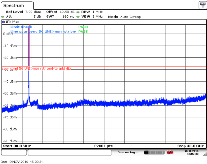
Figure 8.4-26: Peak spurious emissions outside restricted bands at low channel, 802.11ac-VHT40, ch52
