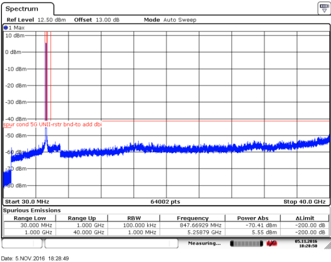
Figure 8.4-12: Peak spurious emissions within restricted bands at low channel, 802.11ac-VHT40, ch52
