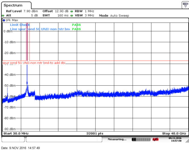
Figure 8.4-17: Peak spurious emissions outside restricted bands at high channel, 802.11a, ch64
