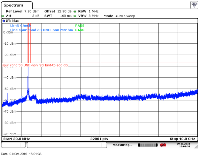
Figure 8.4-24: Peak spurious emissions outside restricted bands at mid channel, 802.11ac-VHT20, ch60
