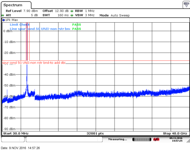
Figure 8.4-16: Peak spurious emissions outside restricted bands at mid channel, 802.11a, ch60
