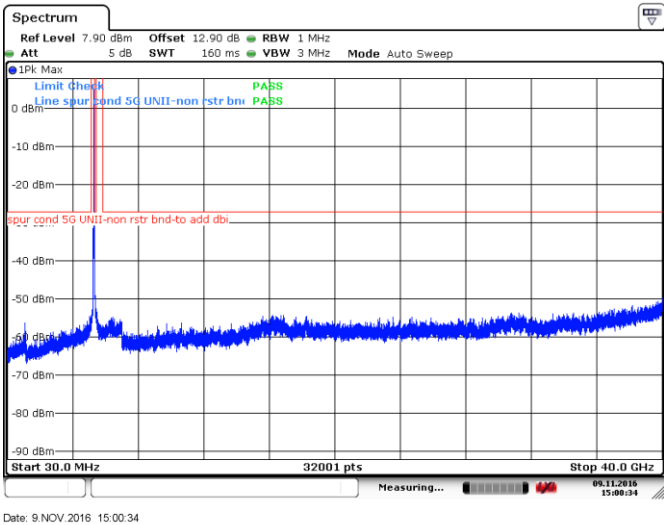
Figure 8.4-22: Peak spurious emissions outside restricted bands at high channel, 802.11n-HT40, ch60
