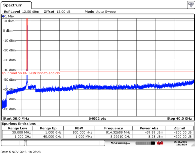
Figure 8.4-7: Peak spurious emissions within restricted bands at low channel, 802.11n-HT40, ch52
