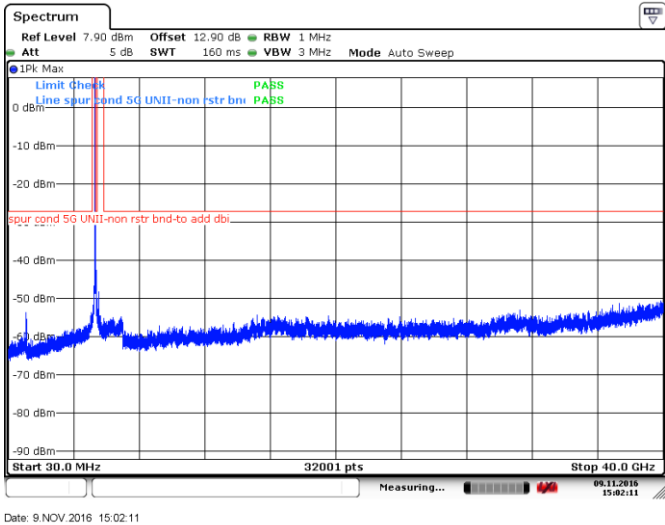
Figure 8.4-25: Peak spurious emissions outside restricted bands at high channel, 802.11ac-VHT20, ch64
