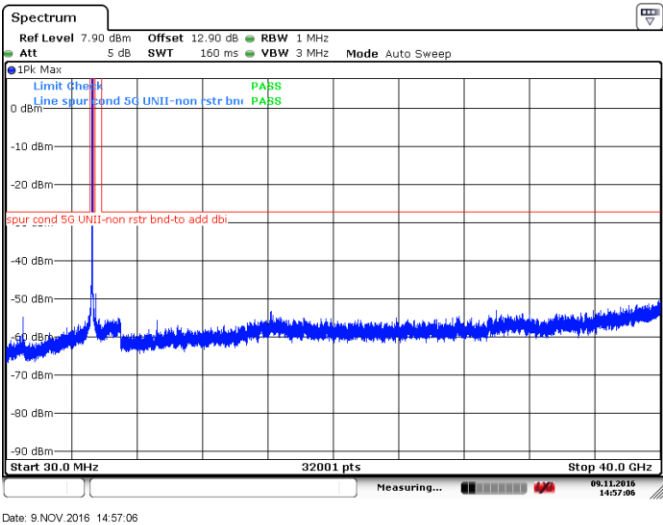
Figure 8.4-15: Peak spurious emissions outside restricted bands at low channel, 802.11a, ch52
