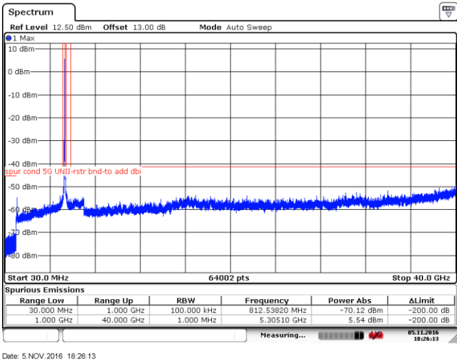
Figure 8.4-8: Peak spurious emissions within restricted bands at high channel, 802.11n-HT40, ch60
