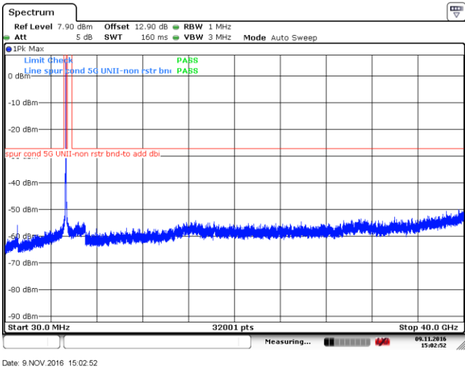
Figure 8.4-27: Peak spurious emissions outside restricted bands at high channel, 802.11ac-VHT40, ch60
