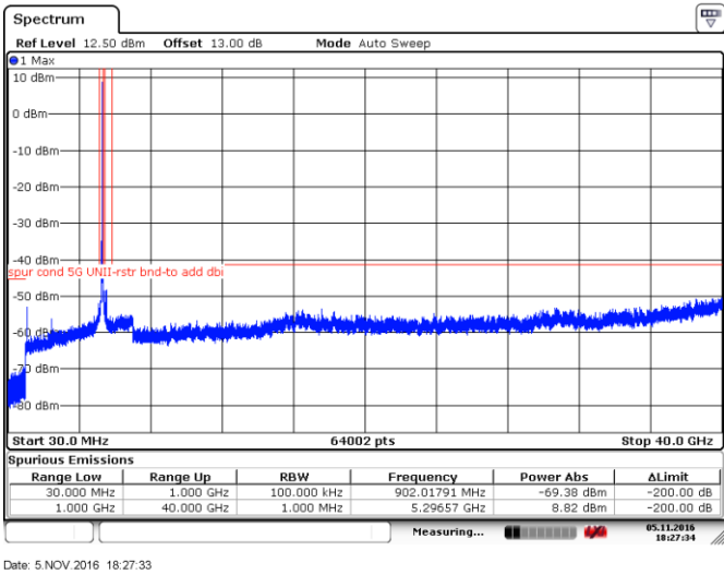
Figure 8.4-10: Peak spurious emissions within restricted bands at mid channel, 802.11ac-VHT20, ch60
