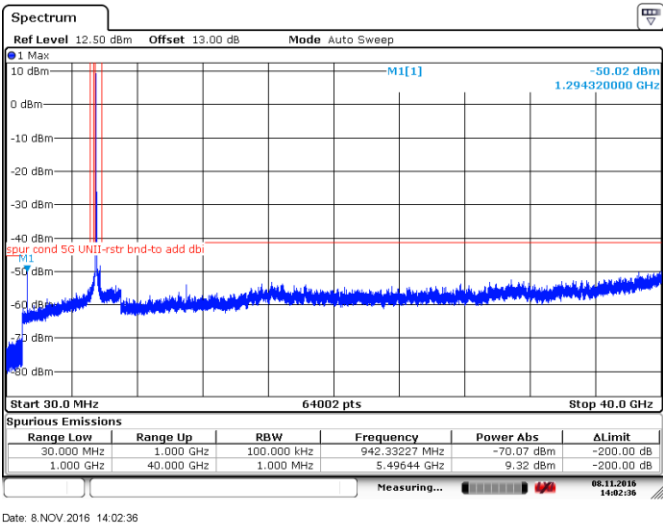
Figure 8.4-4: Peak spurious emissions within restricted bands at low channel, 802.11n-HT20, ch100
