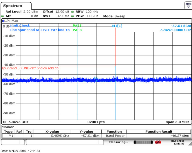
Figure 8.4-37: Lower band edge emission(restricted band), 802.11a
