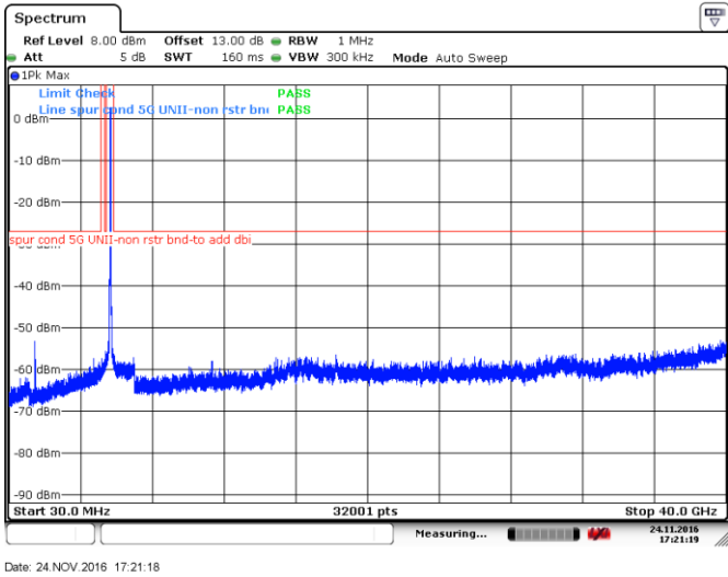
Figure 8.4-26: Peak spurious emissions outside restricted bands at mid channel, 802.11n-HT40, ch132
