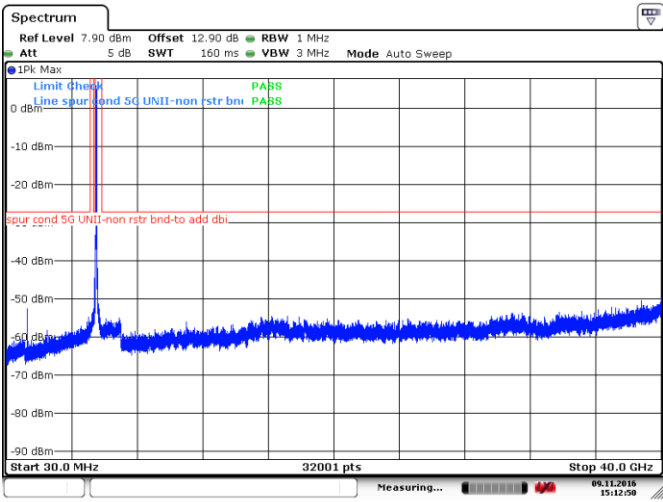
Figure 8.4-30: Peak spurious emissions outside restricted bands at low channel, 802.11ac-VHT40, ch100
