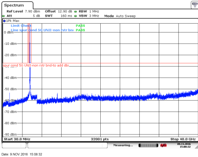
Figure 8.4-25: Peak spurious emissions outside restricted bands at mid channel, 802.11n-HT40, ch116
