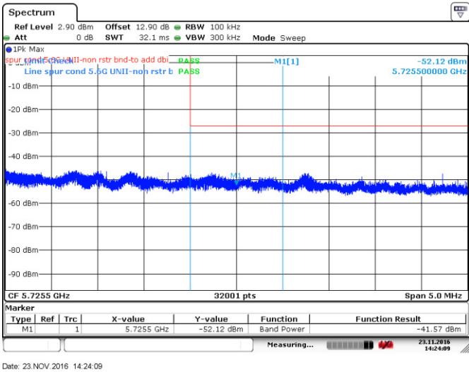
Figure 8.4-36: Upper band edge emission, 802.11a
