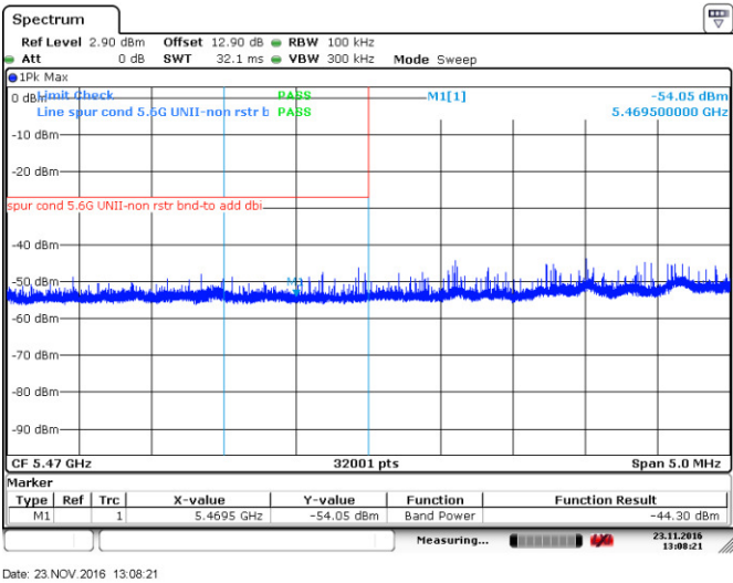
Figure 8.4-35: Lower band edge emission, 802.11a
