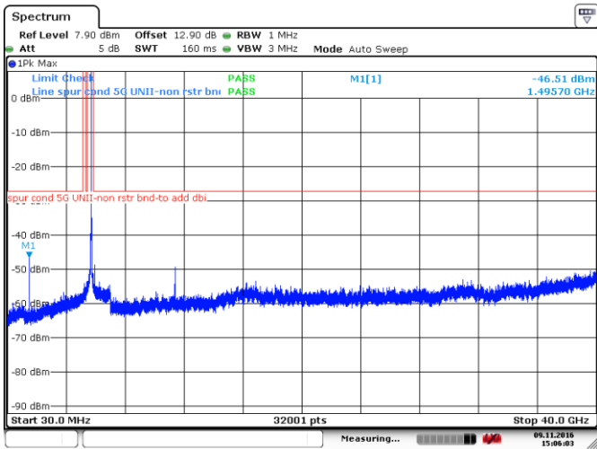
Figure 8.4-20: Peak spurious emissions outside restricted bands at high channel, 802.11a, ch140
