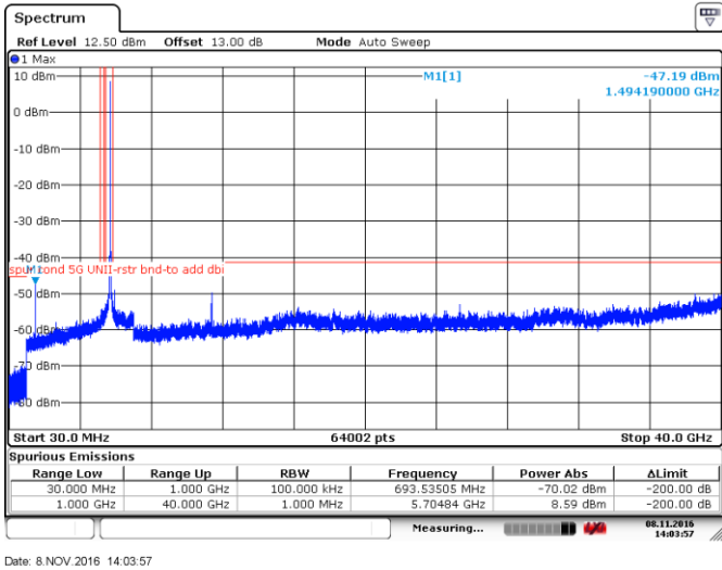
Figure 8.4-6: Peak spurious emissions within restricted bands at high channel, 802.11n-HT20, ch140
