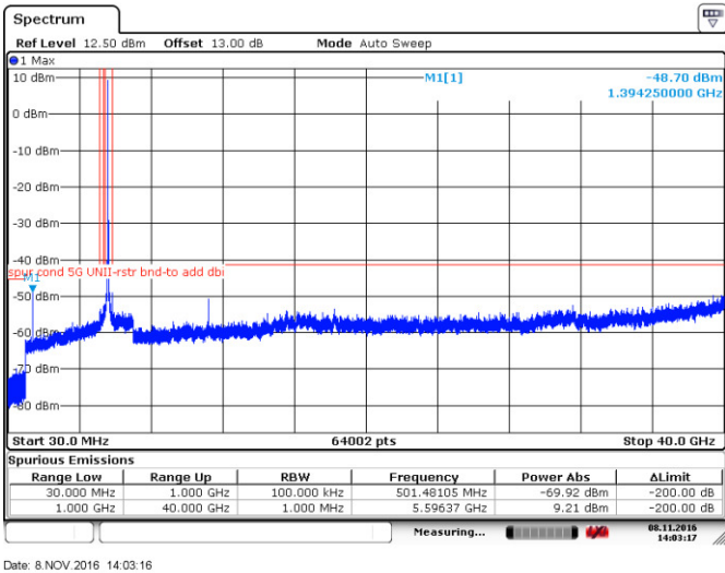
Figure 8.4-5: Peak spurious emissions within restricted bands at mid channel, 802.11n-HT20, ch120
