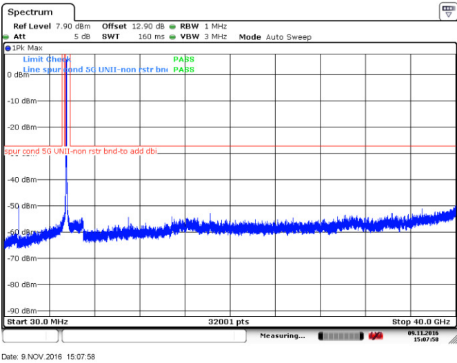
Figure 8.4-24: Peak spurious emissions outside restricted bands at low channel, 802.11n-HT40, ch100
