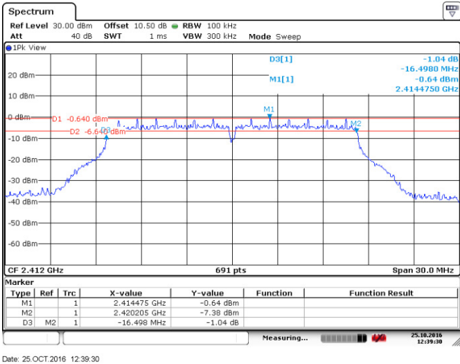
Figure 8.2-2: 6 dB bandwidth on 802.11g, sample plot
