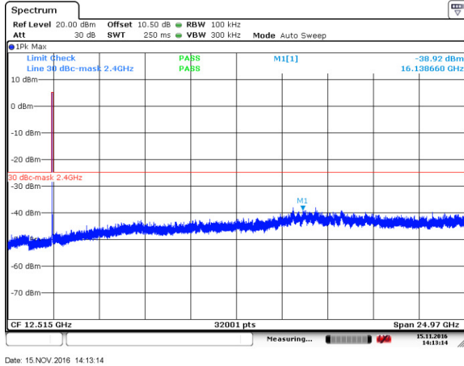
Figure 8.4-4: Conducted spurious emissions for 802.11b (TX 2437 MHz)
