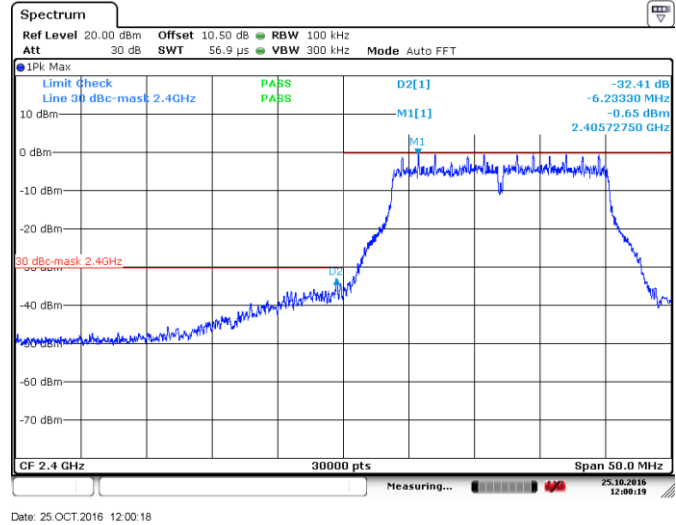
Figure 8.4-11: Conducted spurious emissions Lower band edge for 802.11g, (TX 2412 MHz)
