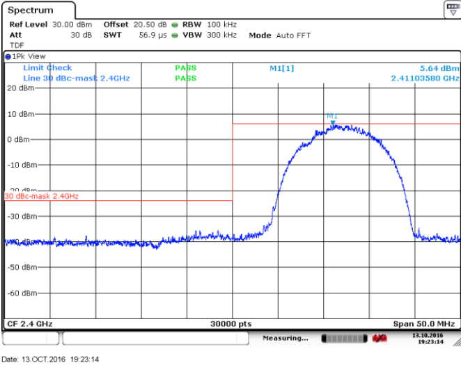
Figure 8.4-10: Conducted spurious emissions Lower band edge for 802.11b, (TX 2412 MHz)
