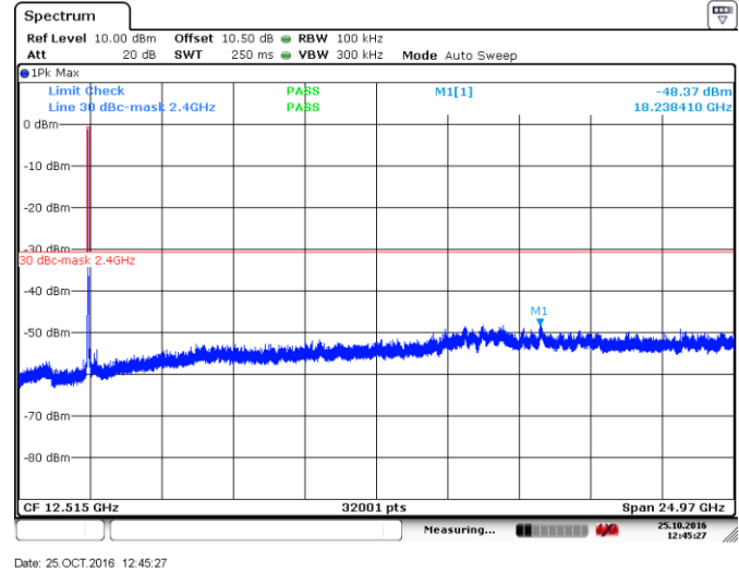
Figure 8.4-5: Conducted spurious emissions for 802.11g (TX 2437 MHz)
