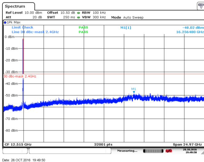
Figure 8.4-6: Conducted spurious emissions for 802.11n HT20 (TX 2437 MHz)
