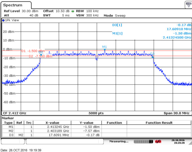
Figure 8.2-3: 6 dB bandwidth on 802.11n, sample plot
