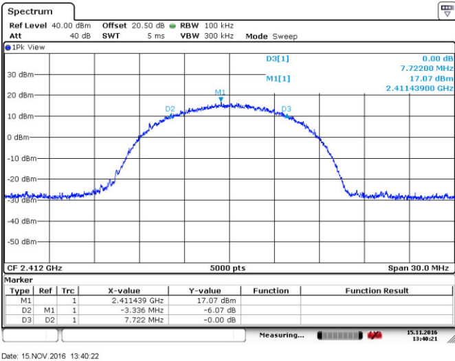
Figure 8.2-1: 6 dB bandwidth on 802.11b, sample plot
