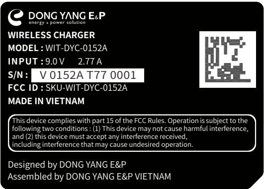
<Label print spec> Scale 2:1
