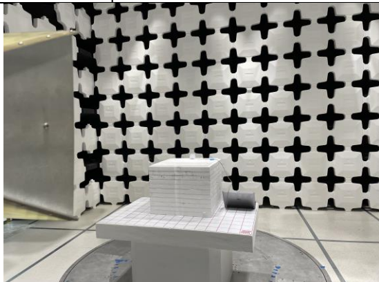
Radiated Spurious Emission- 1GHz to 18GHz-Front
