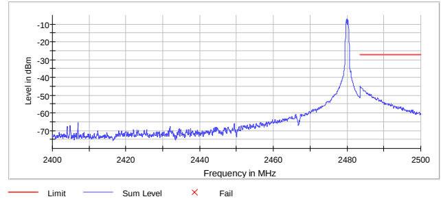
Figure 7.5.1.2-5: Upper Band-edge
