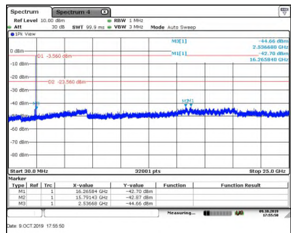
Figure 7.5.1.2-2: MCH – 30MHz–25GHz
