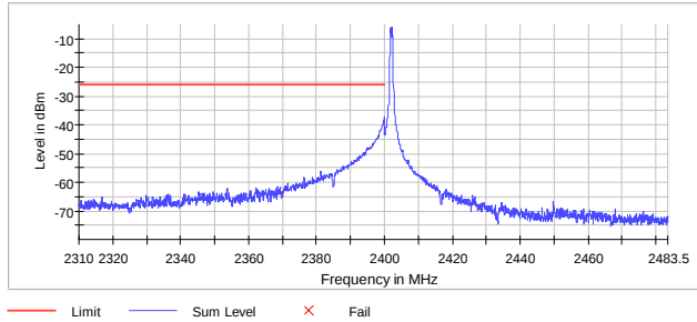
Figure 7.5.1.2-4: Lower Band-edge
