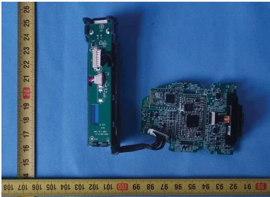
Figure 4. Internal view
