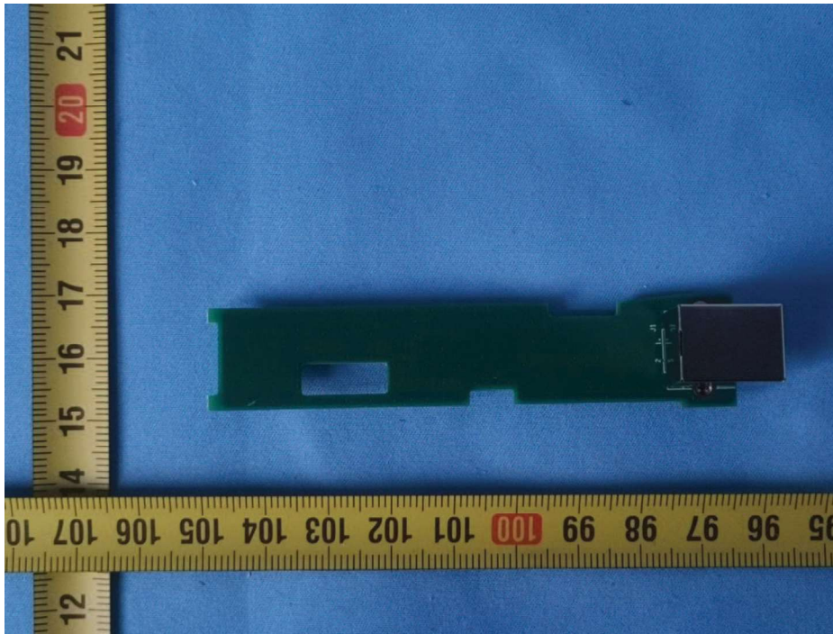
Figure 9. PCB view
