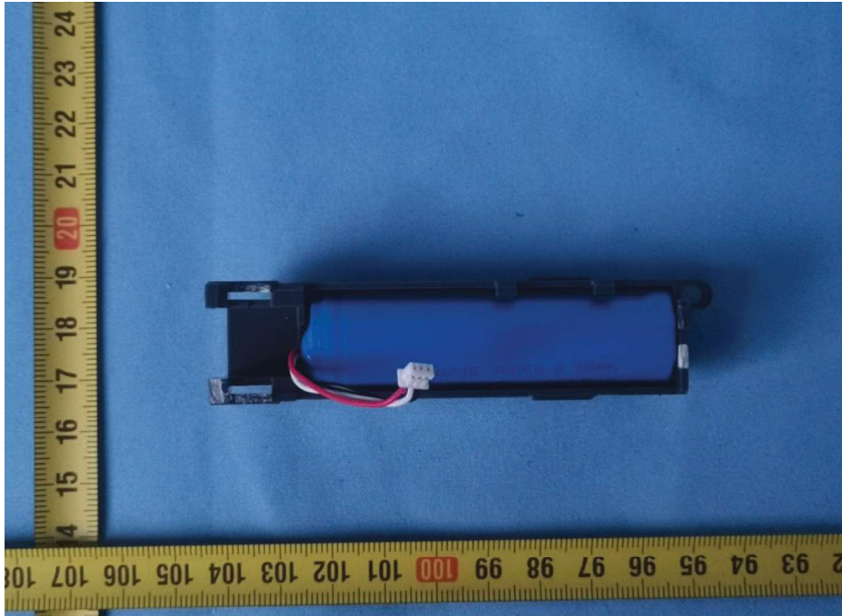
Figure 5. Internal view
