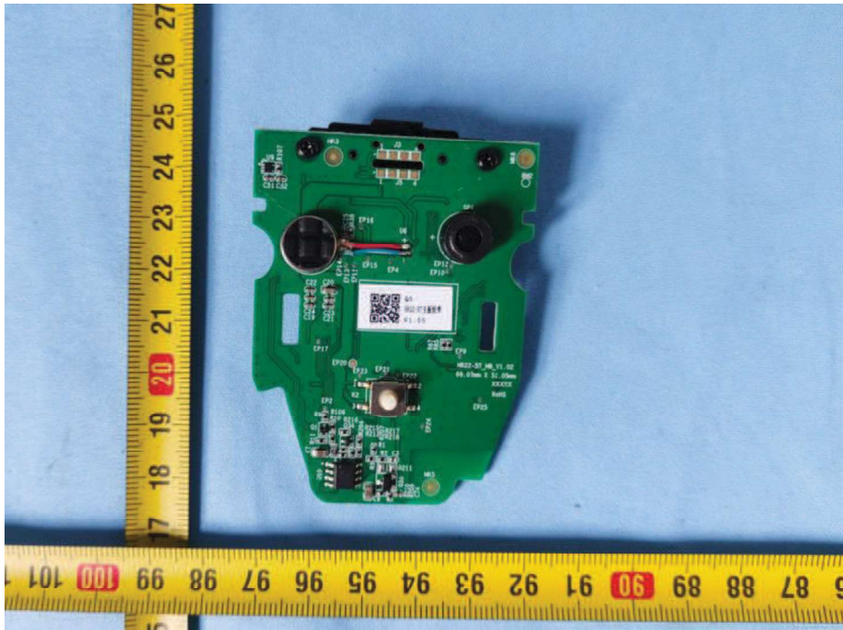
Figure 7. PCB view
