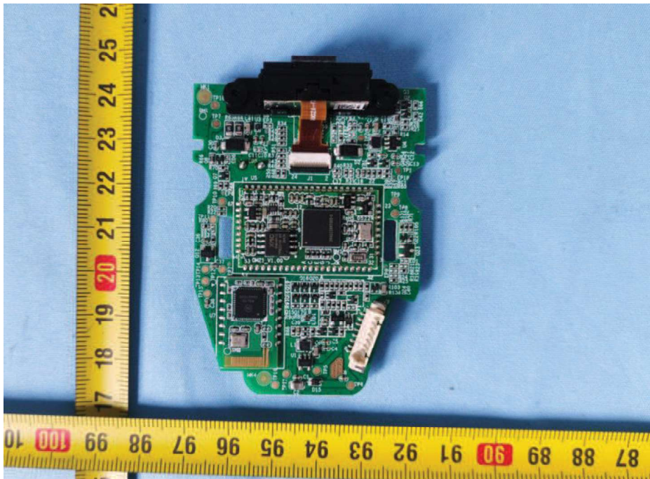
Figure 6. PCB view
