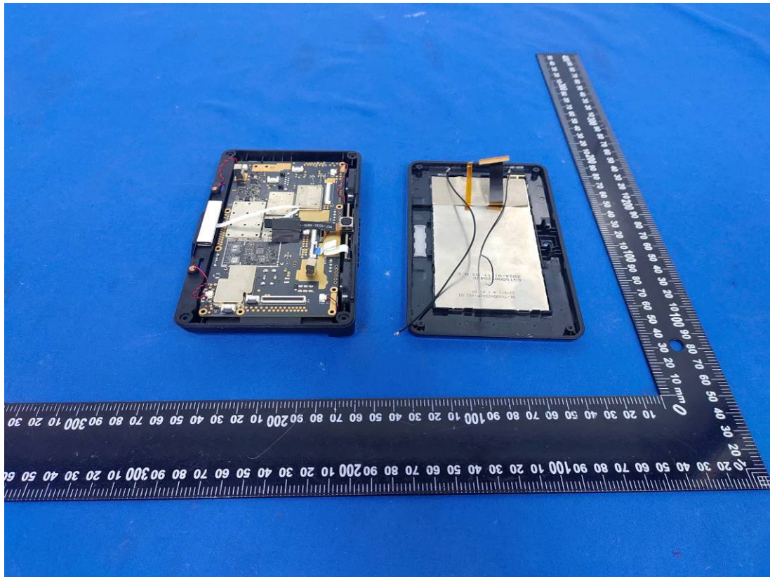
2.4G WIFI & BT Antenna
