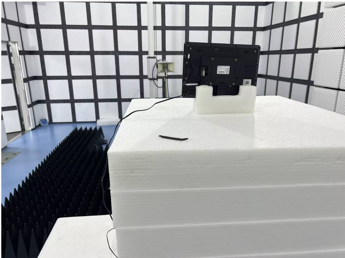
RE-Back View_NLS-NQuire1000 (6GHz – 18GHz )
