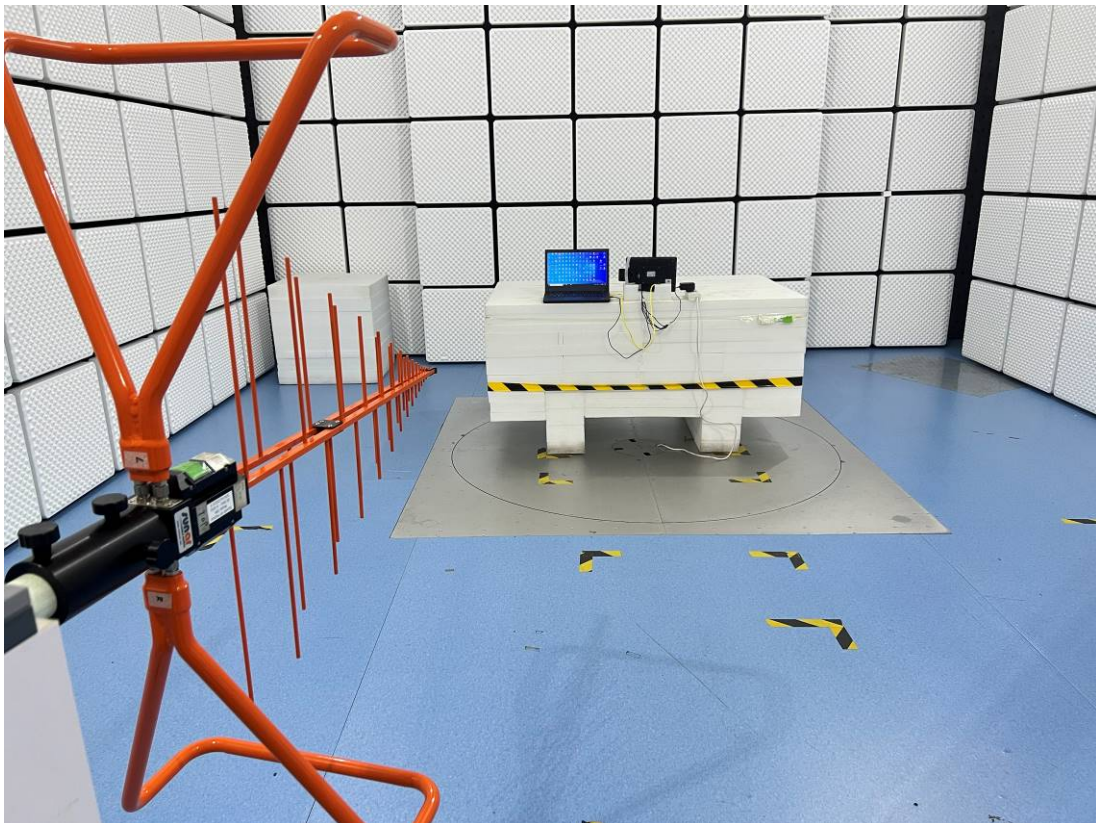
RE-Back View_NLS-NQuire1000 (30MHz~1GHz)
