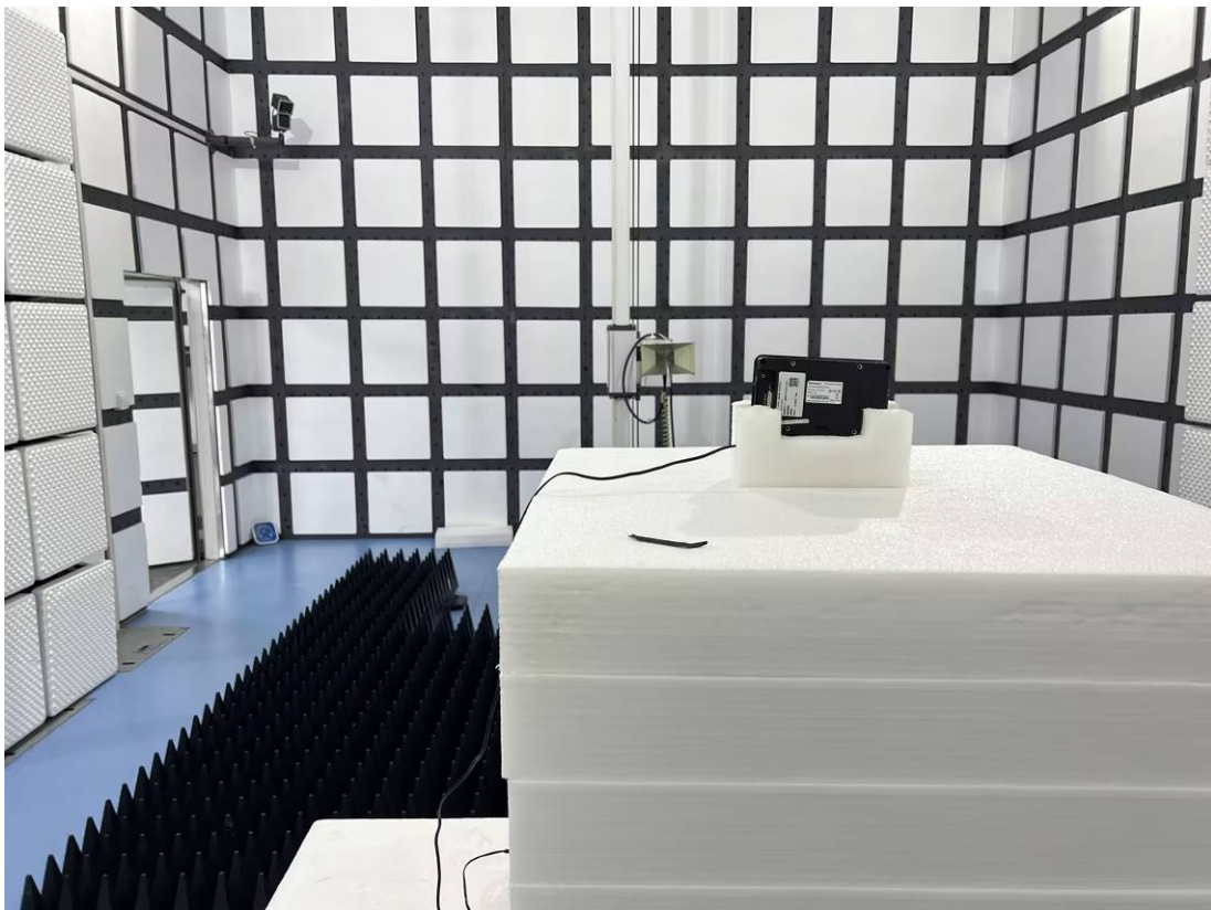
RE-Back View_NLS-NQuire500 (3GHz – 18GHz )
