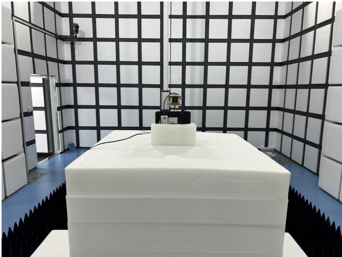
RE-Back View_NLS-NQuire500 (1GHz – 3GHz )
