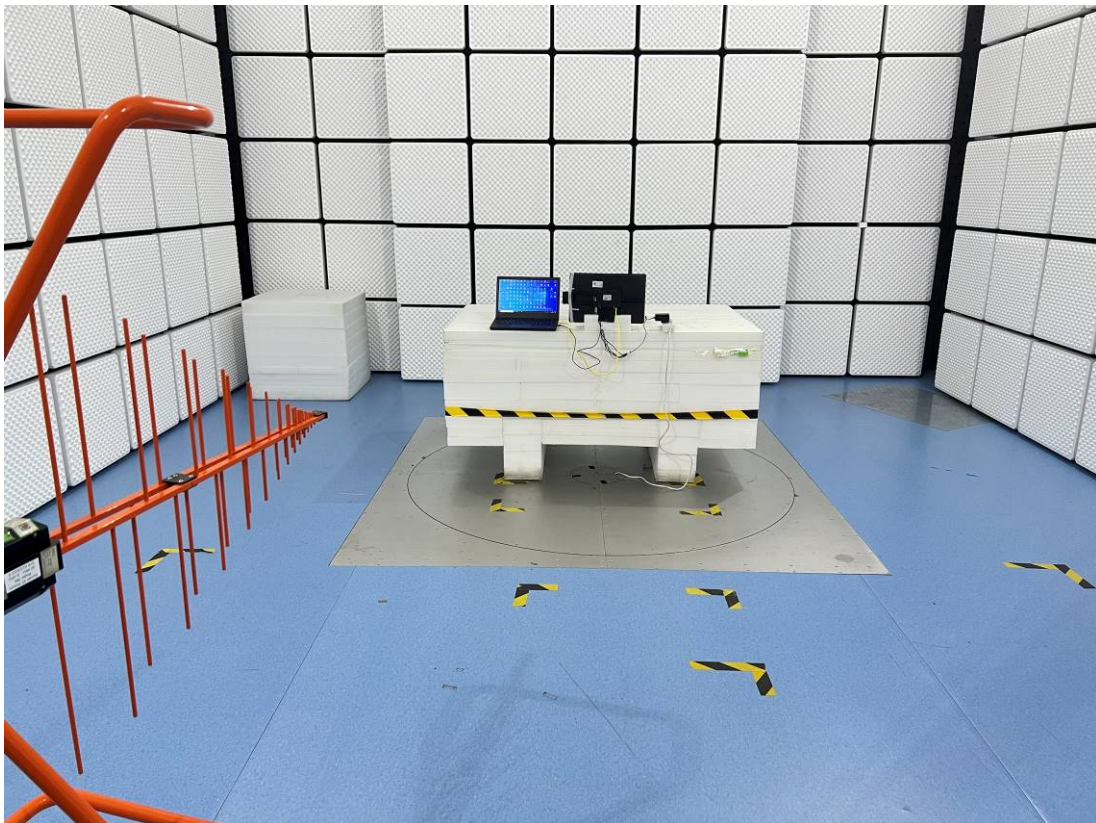
RE-Back View_NLS-NQuire1500 (30MHz~1GHz)
