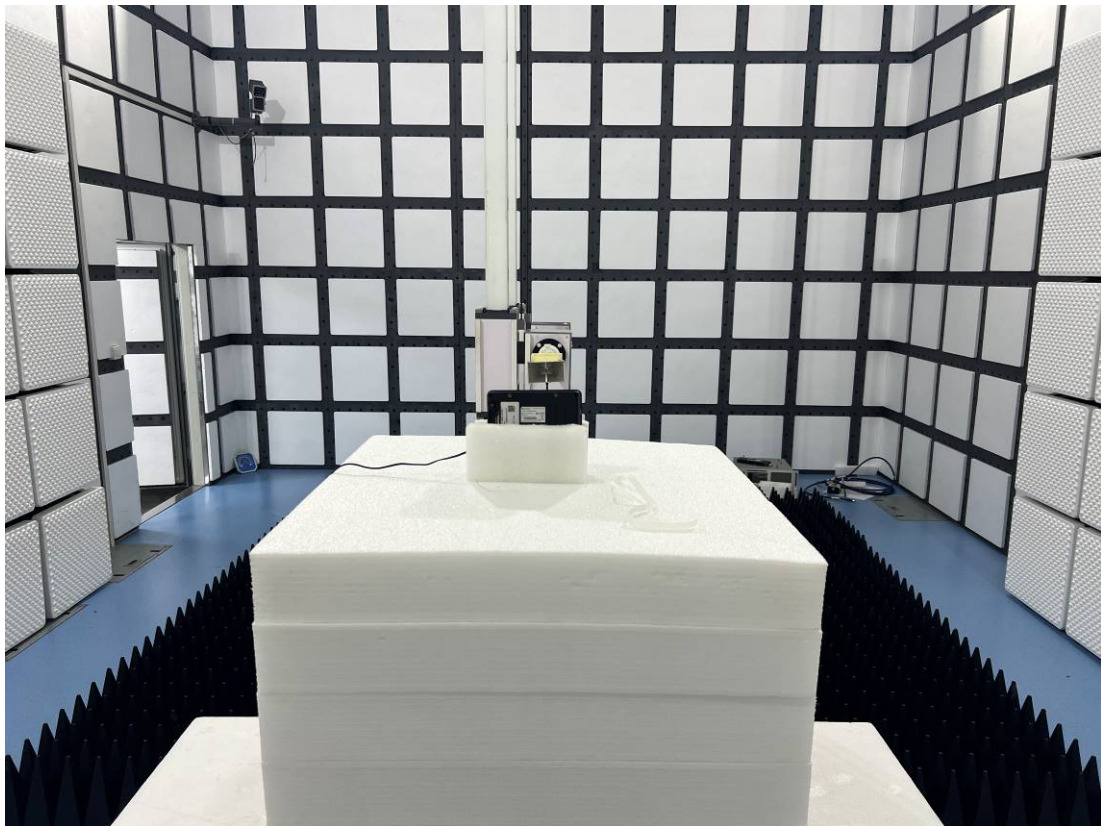
RE-Back View_NLS-NQuire500 (Above 18GHz )
