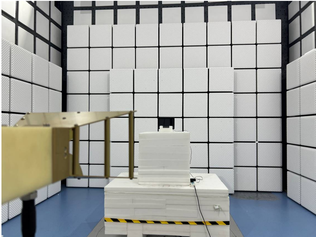
RE-Back View_NLS-NQuire1000(1GHz – 3GHz )
