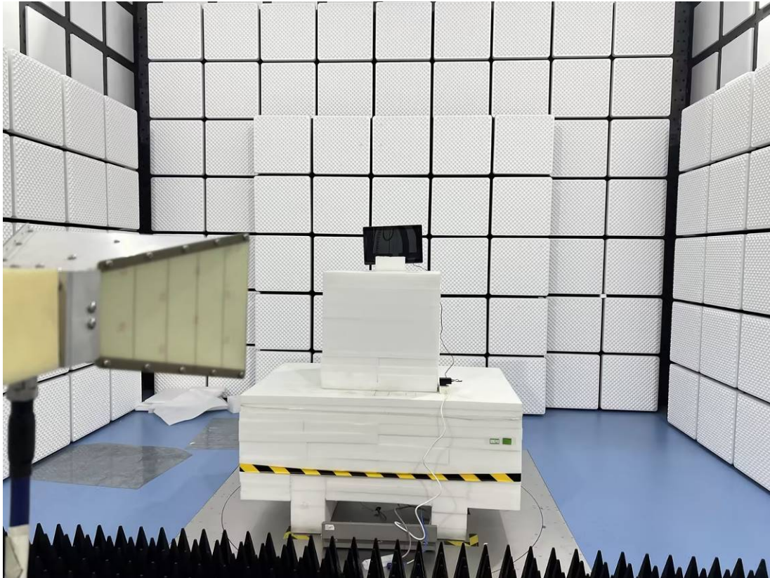
RE-Back View_NLS-NQuire1500 (3GHz – 18GHz )
