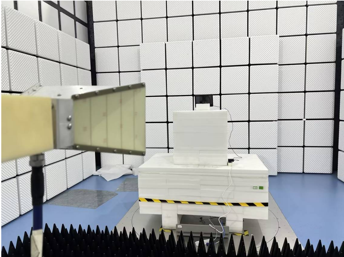
RE-Back View_NLS-NQuire1000 (3GHz – 18GHz )
