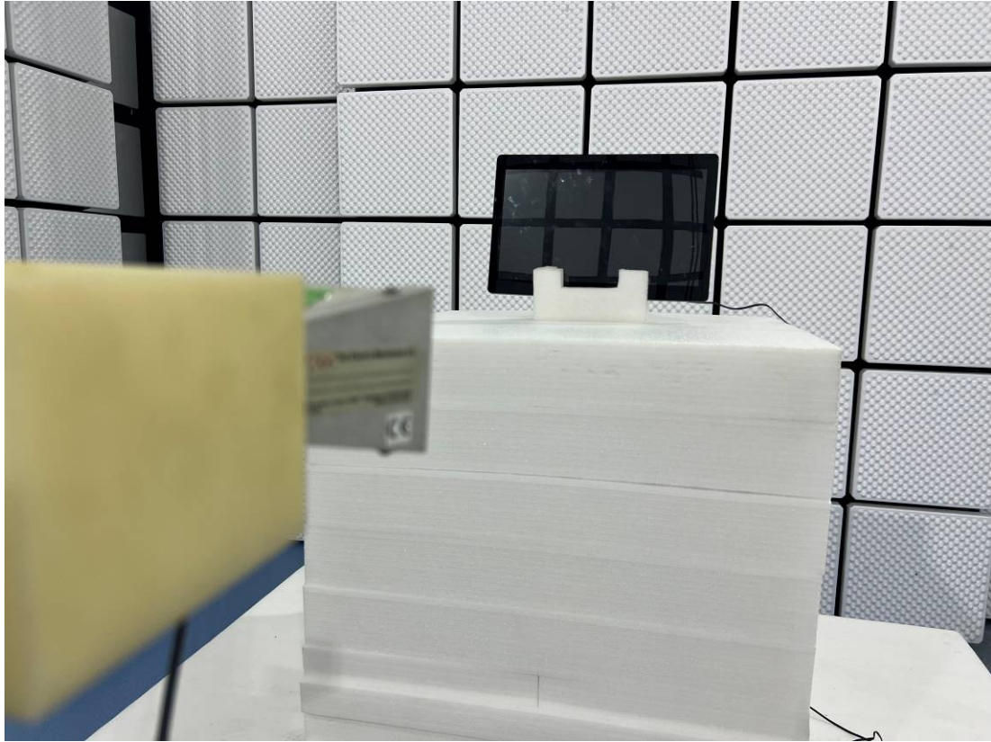
RE-Back View_NLS-NQuire1500 (Above 18GHz )
