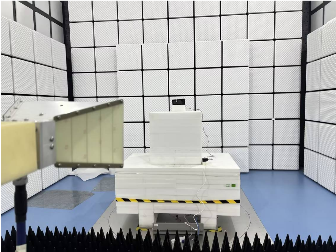
RE-Back View_NLS-NQuire700 (3GHz – 18GHz )
