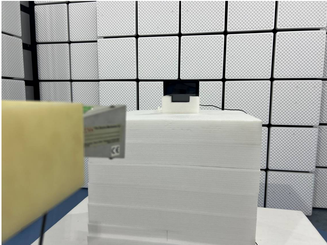
RE-Back View_NLS-NQuire700(Above 18GHz )
