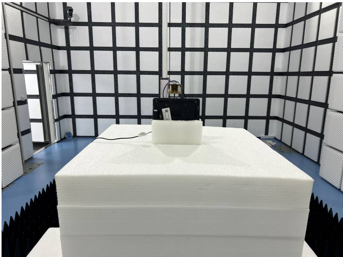
RE-Back View_NLS-NQuire700(1GHz – 3GHz )
