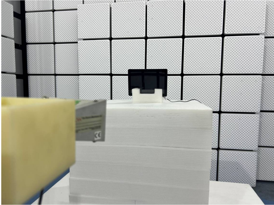
RE-Back View_NLS-NQuire1000 (Above 18GHz )
