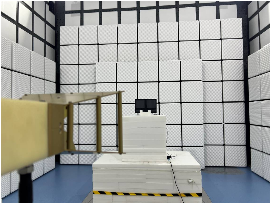
RE-Back View_NLS-NQuire1500 (1GHz – 3GHz )
