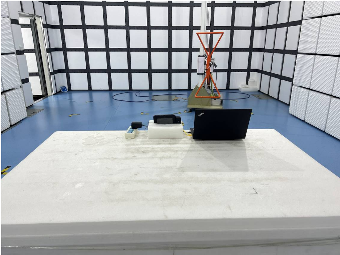
RE-Back View_NLS-NQuire500 (30MHz~1GHz)
