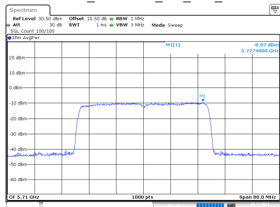
802.11ax40_5710MHz_RU_Full_Chain 1
