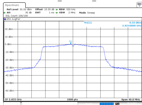
802.11n20_5825MHz_Chain 1
