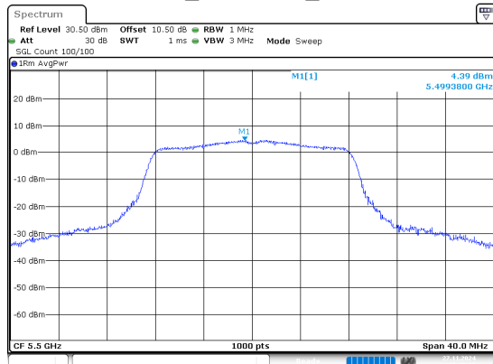
802.11a_5500MHz_Chain 0
