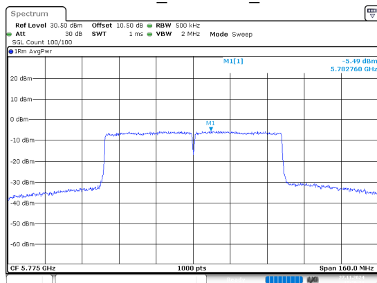
802.11ac80_5775MHz_Chain 0
