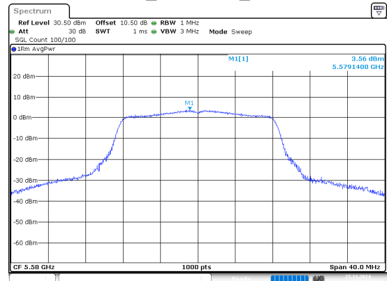
802.11a_5580MHz_Chain 0
