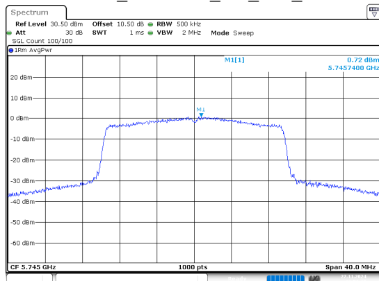
802.11ax20_5745MHz_RU_Full_Chain 0
