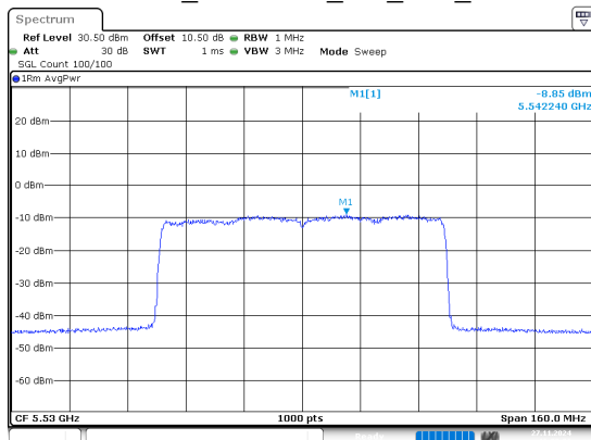
802.11ax80_5530MHz_RU_Full_Chain 0
