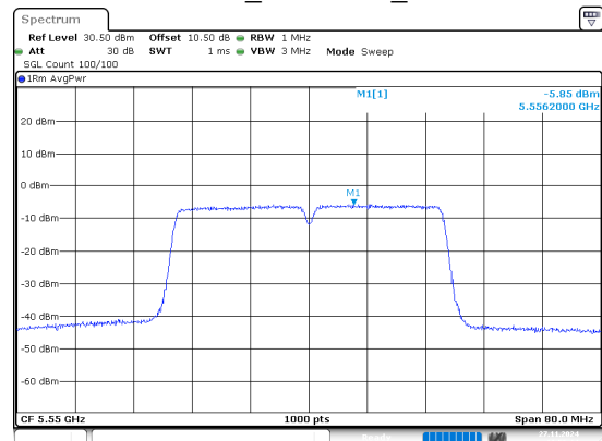
802.11n40_5550MHz_Chain 0
