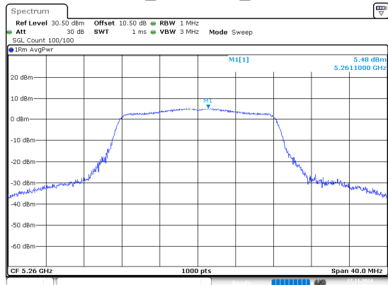
802.11a_5260MHz_Chain 0
