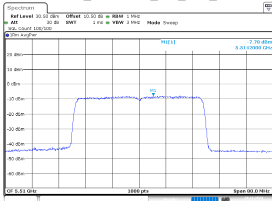
802.11ax40_5510MHz_RU_Full_Chain 1
