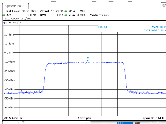
802.11ax40_5670MHz_RU_Full_Chain 1
