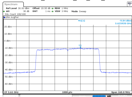
802.11ax80_5610MHz_RU_Full_Chain 0
