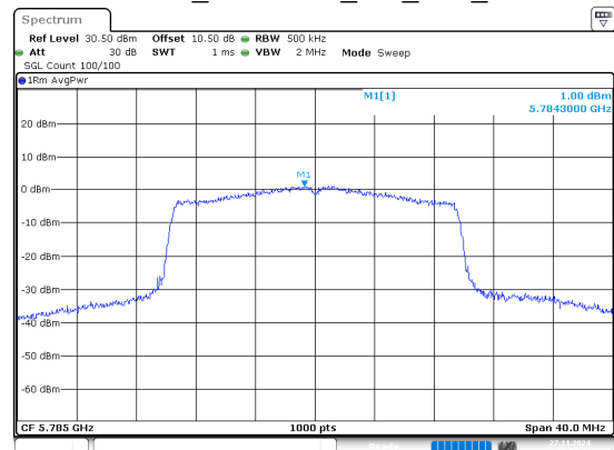
802.11ax20_5785MHz_RU_Full_Chain 0
