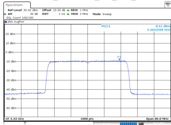
802.11ax40_5550MHz_RU_Full_Chain 1
