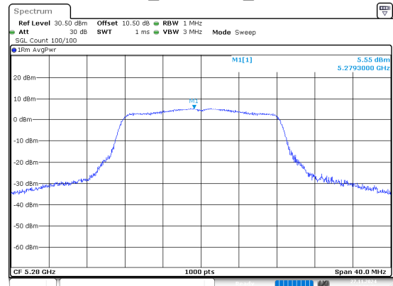
802.11a_5280MHz_Chain 0
