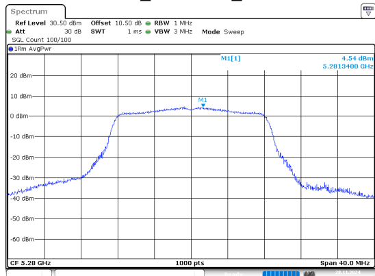
802.11a_5280MHz_Chain 1
