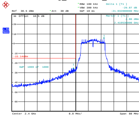
802.11g_2412MHz_Chain 0
