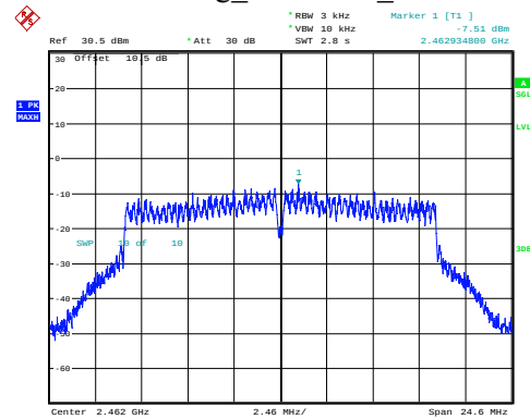
802.11g_2462MHz_Chain 1
