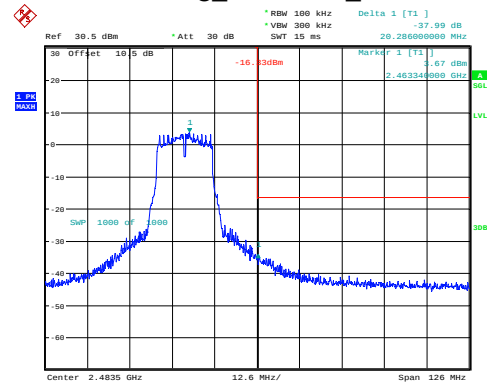
802.11g_2462MHz_Chain 0
