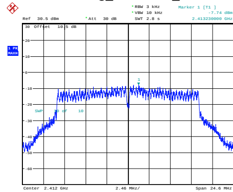
802.11g_2412MHz_Chain 1
