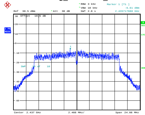
802.11g_2437MHz_Chain 0
