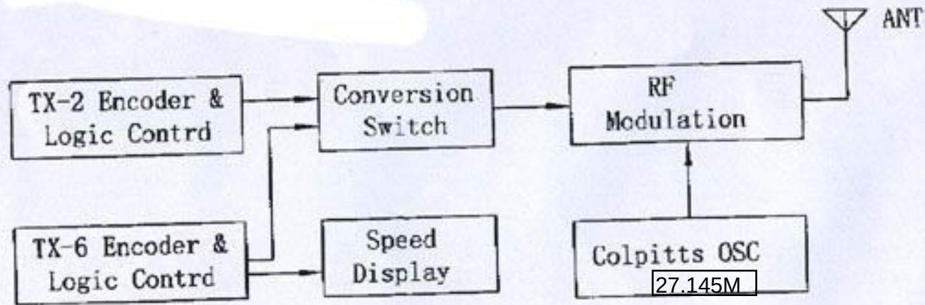
Figure 1. Block Diagram of Transmitter Part
