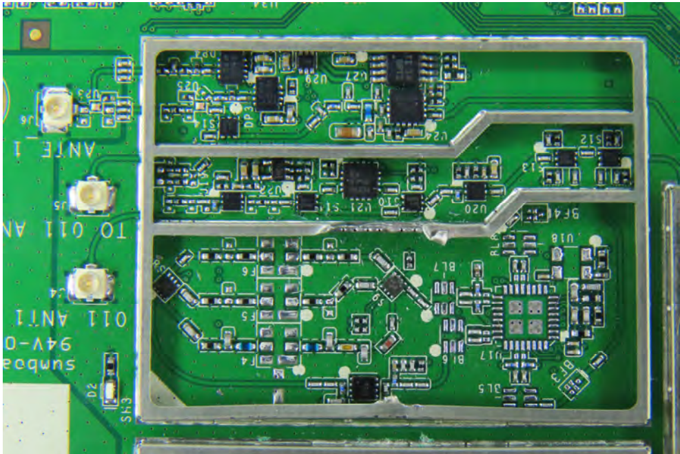
(23) EUT Photo
