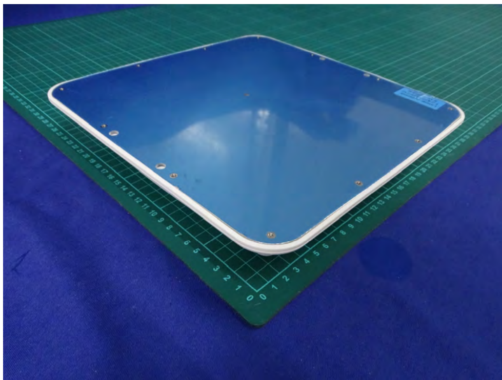
(43) EUT Photo
