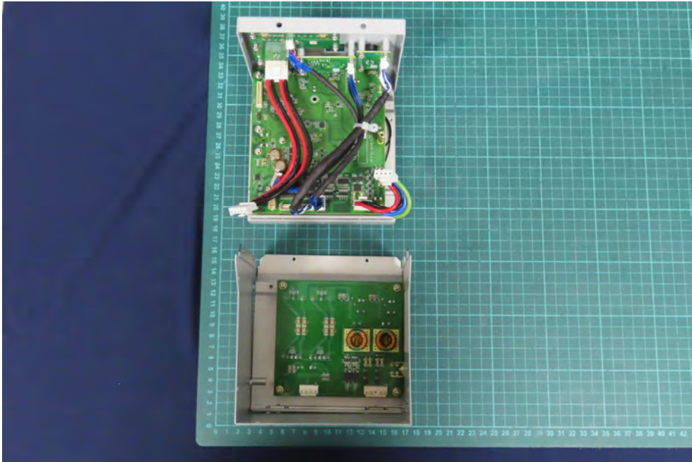
(7) EUT Photo
