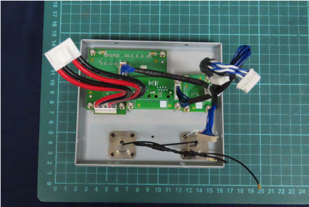
(25) EUT Photo
