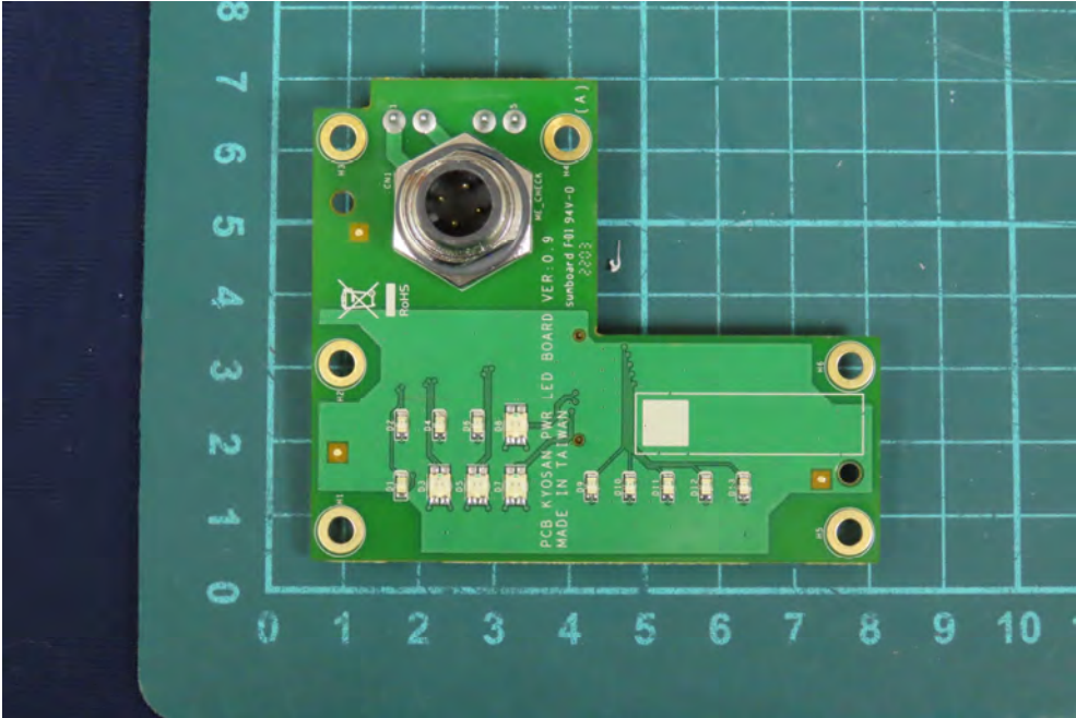
(32) EUT Photo
