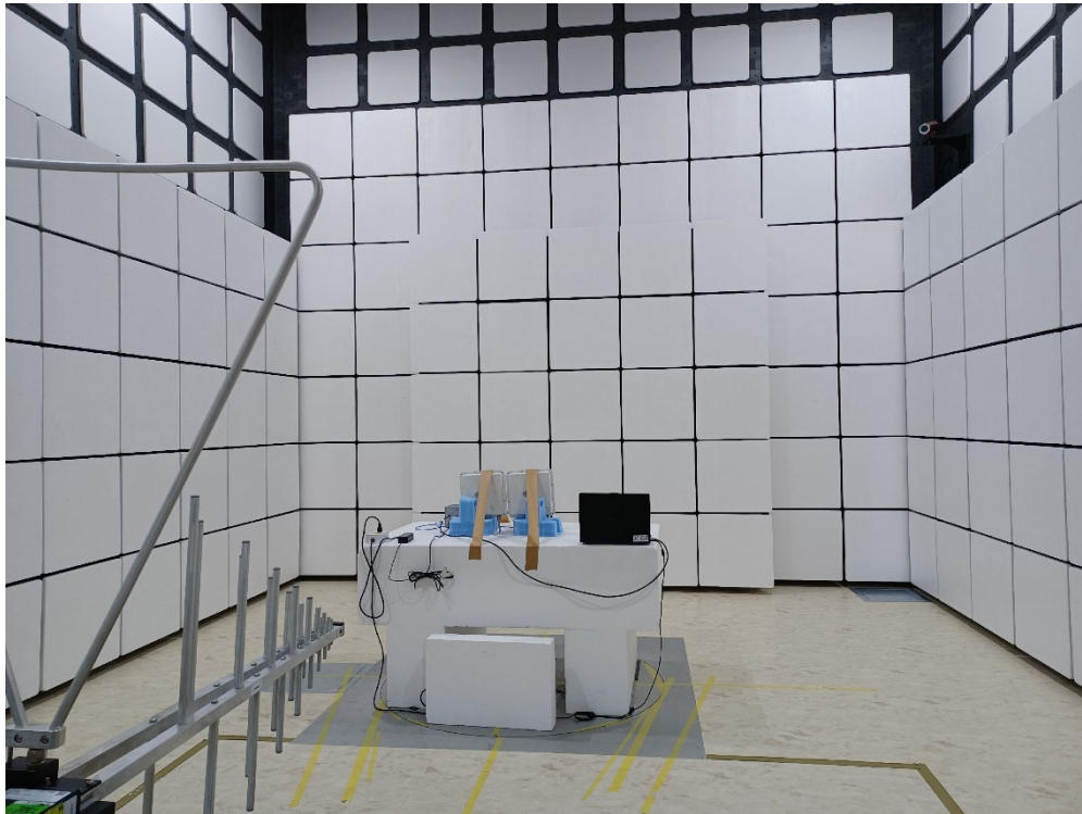
Radiated Test - Panel
