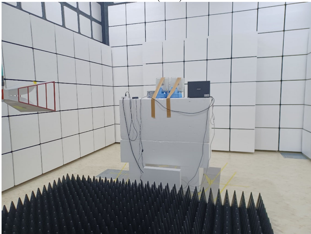
Radiated Test (Horn) - Panel
