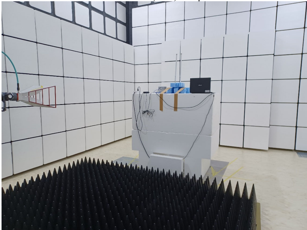
Radiated Test (Horn) - Diople
