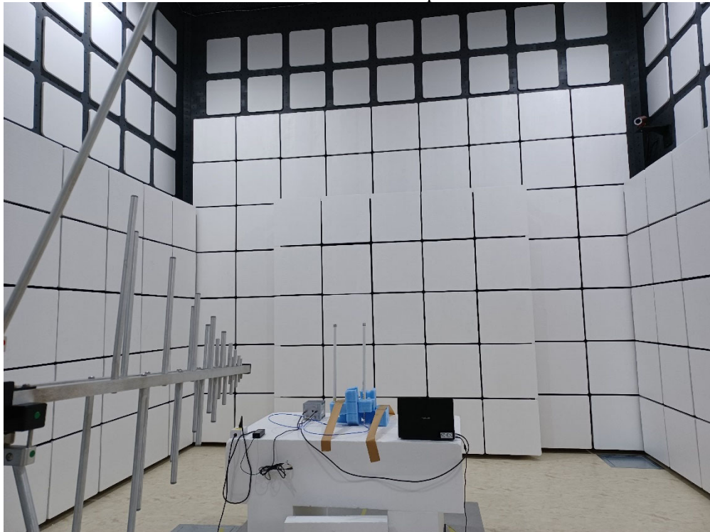
Radiated Test - Diople
