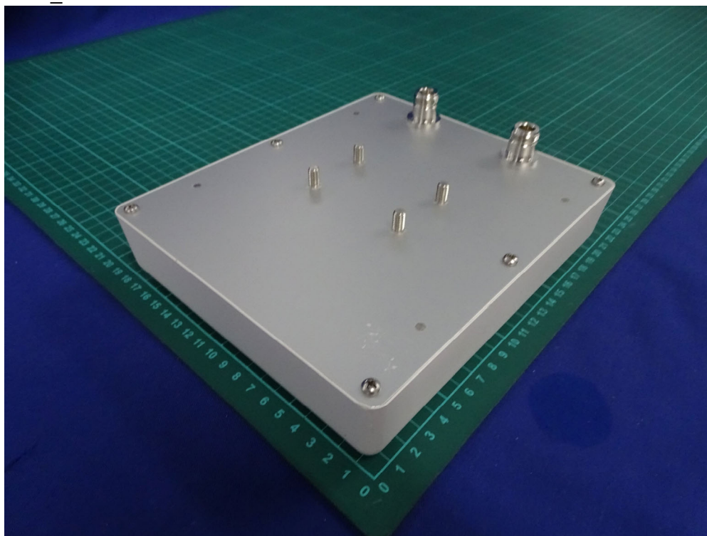
(29) EUT Photo_ Antenna: MOXA / MAT-WDB-PA-NF-2-0708
