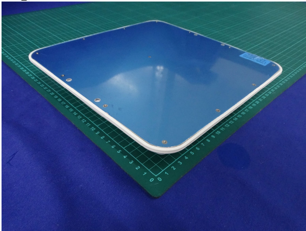
(32) EUT Photo_ Antenna: MOXA / ANT-WDB-PNF-1011
