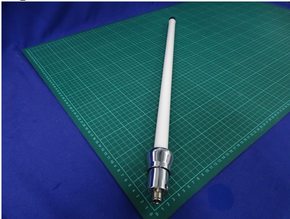
(38) EUT Photo_ Antenna: MOXA / ANT-WDB-ONF-0709
