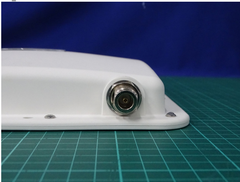
(36) EUT Photo_ Antenna: MOXA / ANT-WSB-PNF-12-02
