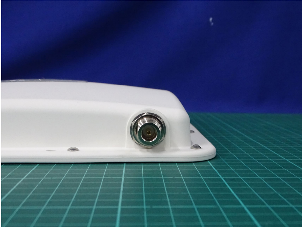
(33) EUT Photo_ Antenna: MOXA / ANT-WSB5-PNF-16
