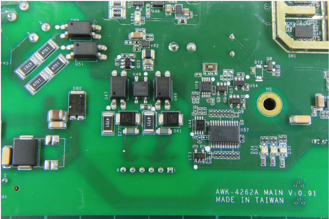
(55) EUT Photo
