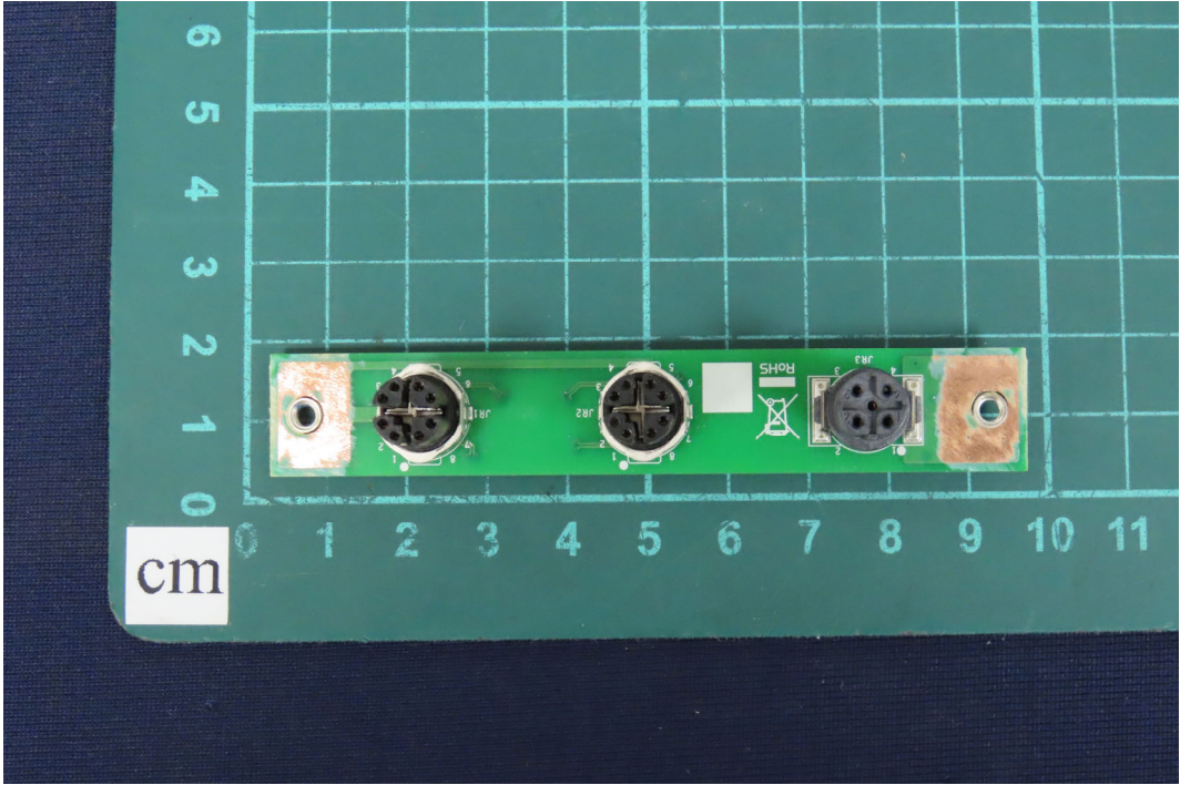
(68) EUT Photo
