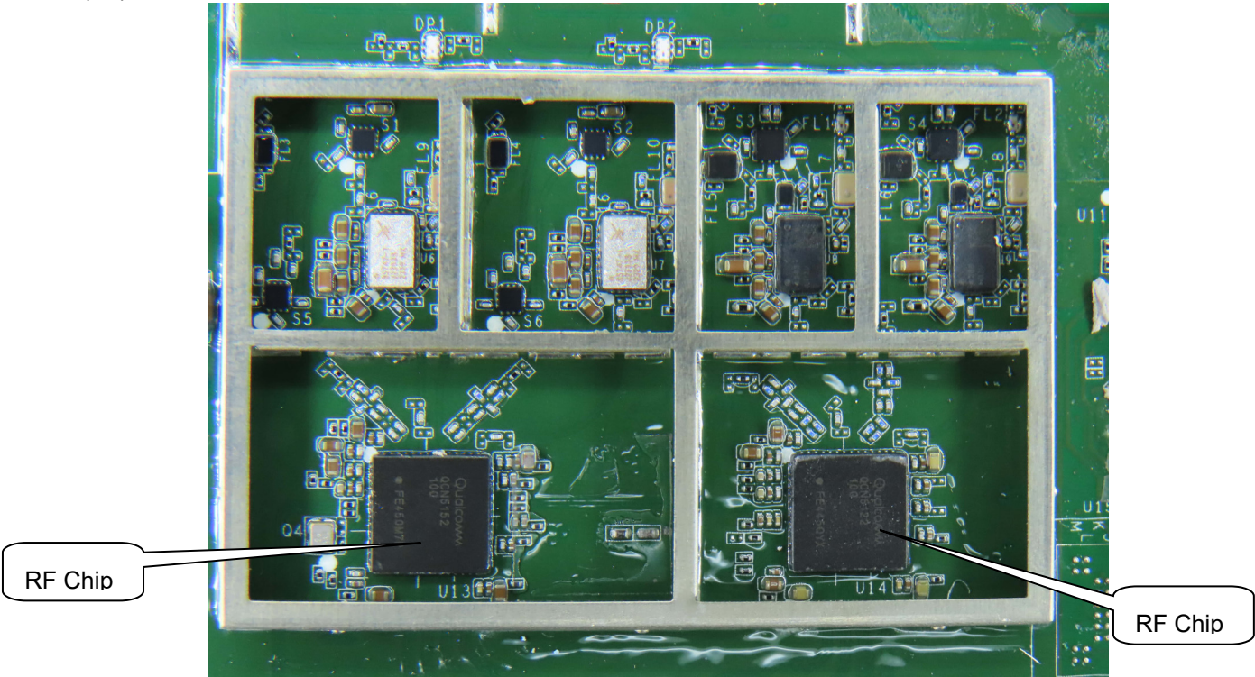
(39) EUT Photo
