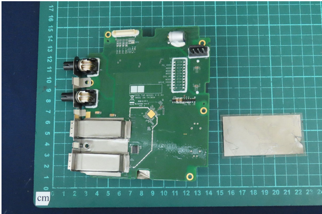
(80) EUT Photo
