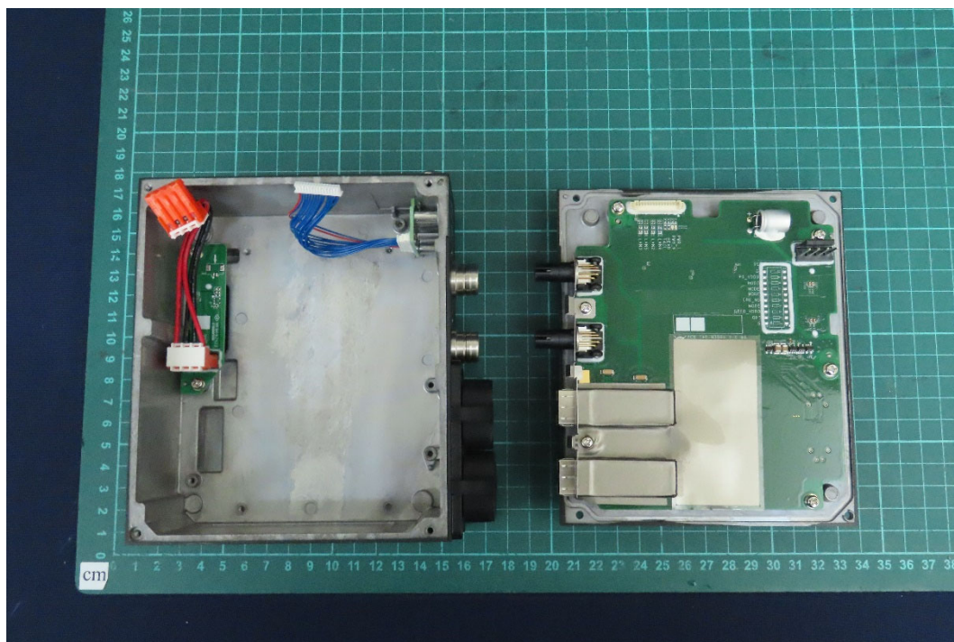
(76) EUT Photo
