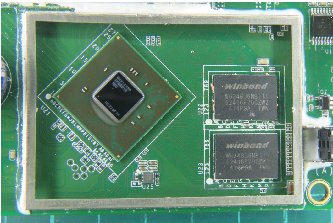
(73) EUT Photo
