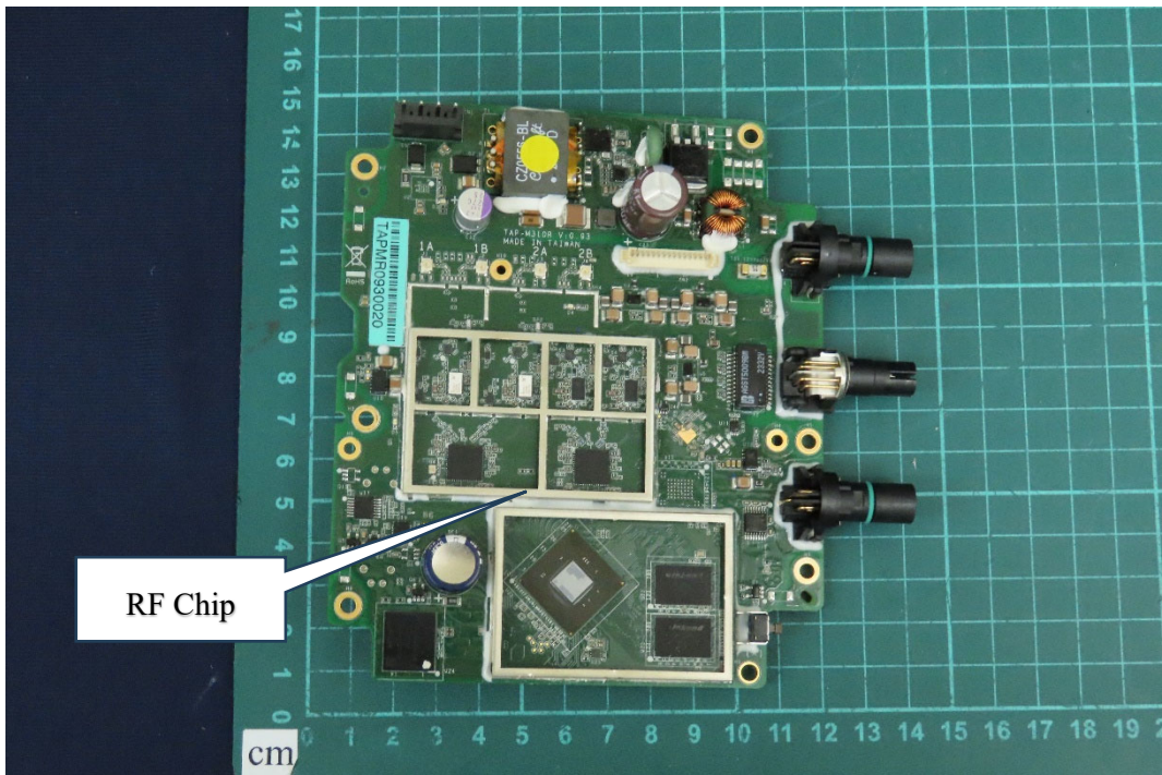
(103) EUT Photo
