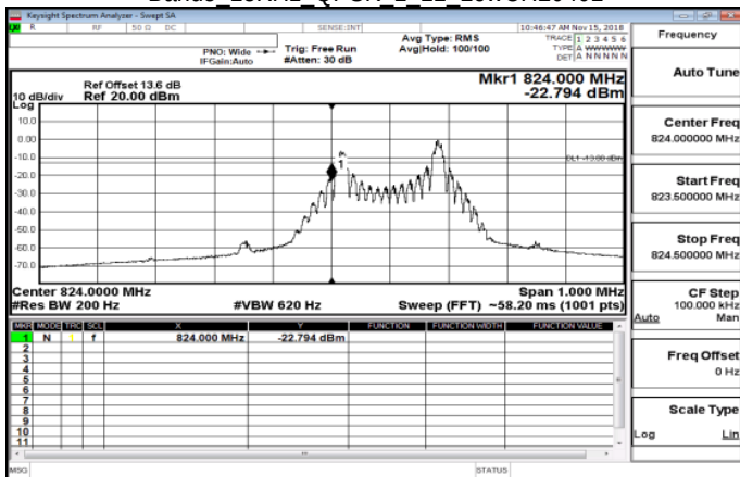
Band5 15KHz QPSK 1 11 LowCH20401
