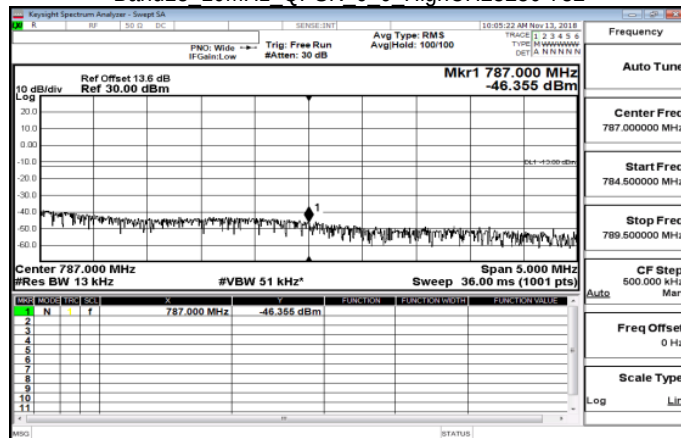
Band13 10MHz QPSK 6 0 HighCH23230-782
