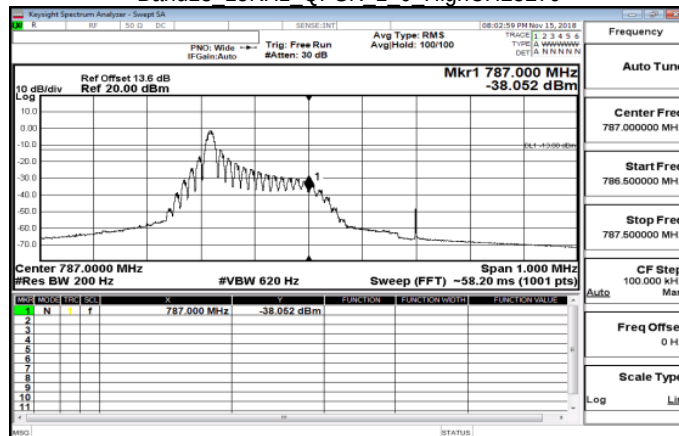
Band13 15KHz QPSK 1 0 HighCH23279
