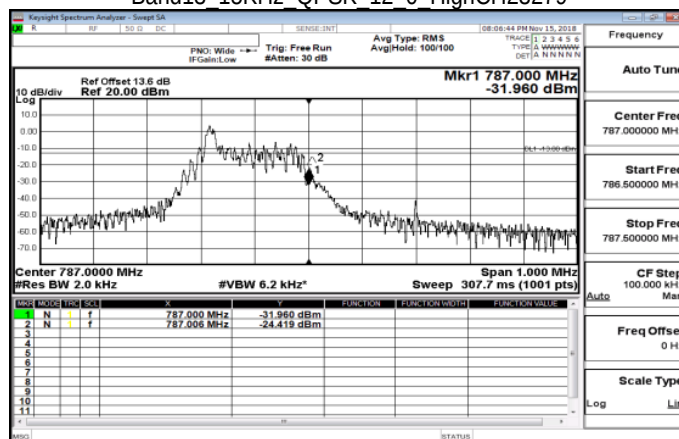
Band13 15KHz QPSK 12 0 HighCH23279
