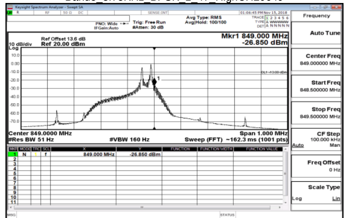
Band5 3.75KHz BPSK 1 47 HighCH20649
