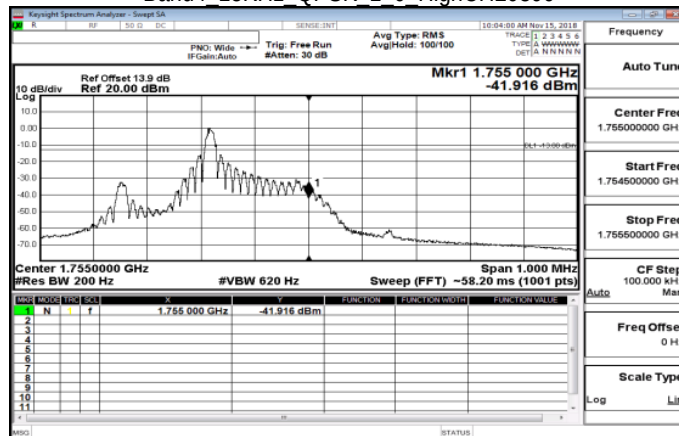
Band4 15KHz QPSK 1 0 HighCH20399
