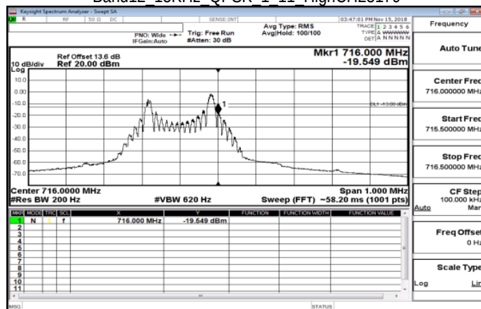
Band12 15KHz QPSK 1 11 HighCH23179
