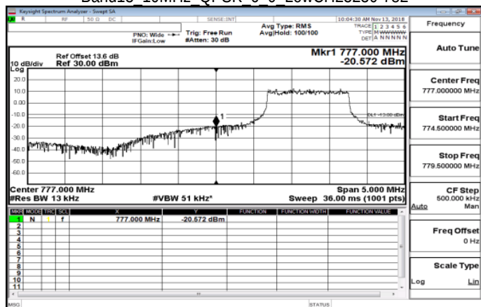
Band13 10MHz QPSK 6 0 LowCH23230-782
