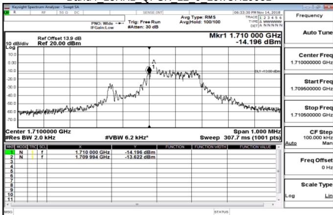
Band4 15KHz QPSK 12 0 LowCH19951
