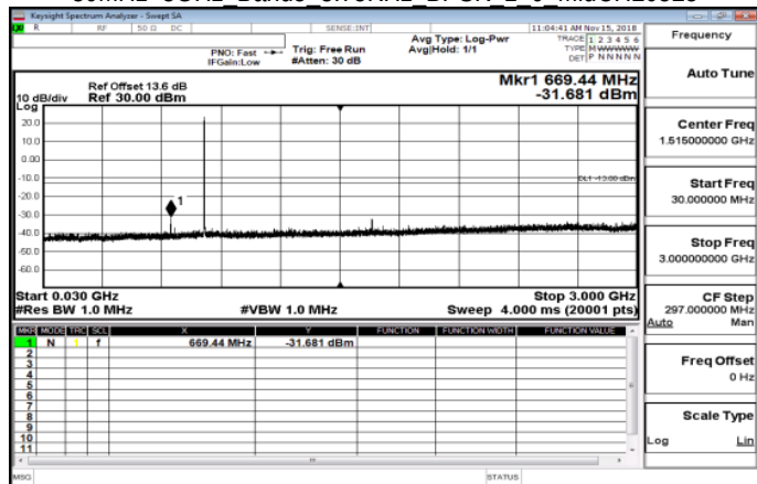
30MHz~3GHz Band5 3.75KHz BPSK 1 0 MidCH20525
