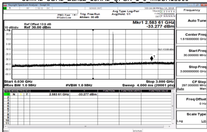
30MHz~3GHz Band2 15KHz QPSK 1 0 MidCH18900
