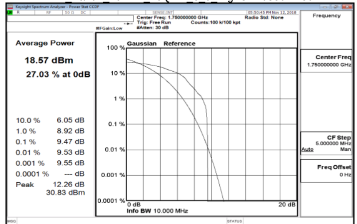
LTE Band4 10MHz 16QAM 6 0 HighCH20350-1750
