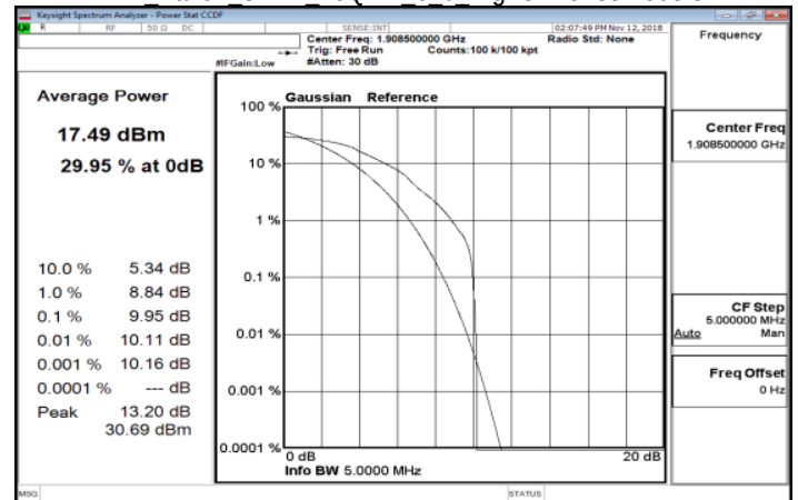
LTE Band2 3MHz 16QAM 6 0 HighCH19185-1908.5
