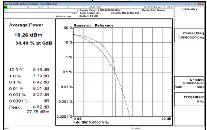
LTE Band4 3MHz 16QAM 6 0 HighCH20385-1753.5
