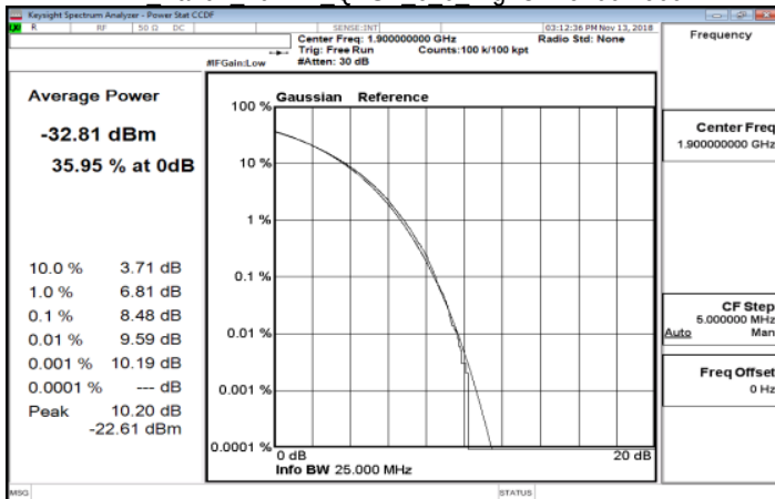
LTE Band2 20MHz QPSK 6 0 HighCH19100-1900
