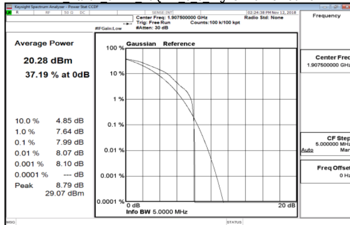
LTE Band2 5MHz 16QAM 6 0 HighCH19175-1907.5
