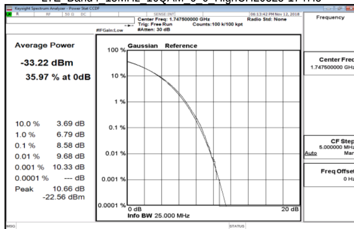
LTE Band4 15MHz 16QAM 6 0 HighCH20325-1747.5
