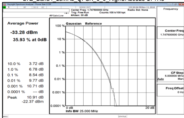
LTE Band4 15MHz QPSK 6 0 HighCH20325-1747.5
