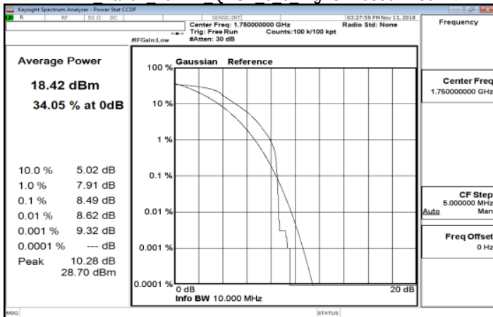
LTE Band4 10MHz QPSK 6 0 HighCH20350-1750
