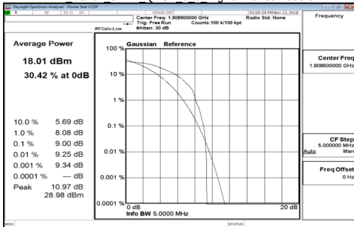
LTE Band2 3MHz QPSK 6 0 HighCH19185-1908.5
