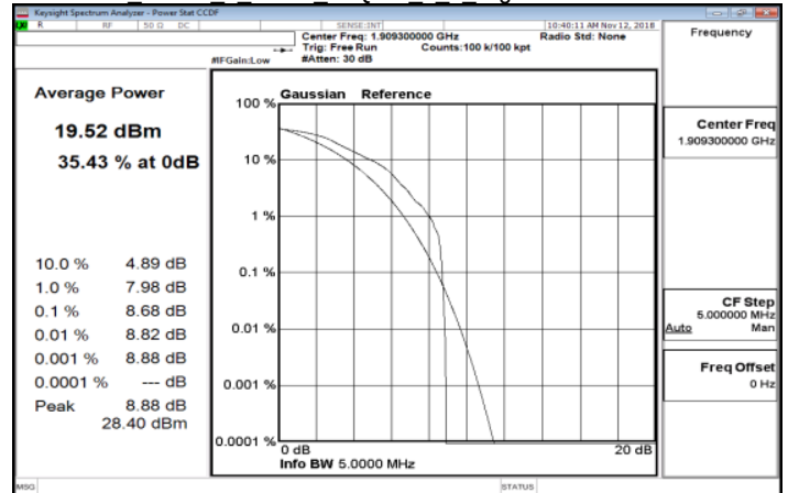
LTE Band2 1 4MHz 16QAM 6 0 HighCH19193-1909.3
