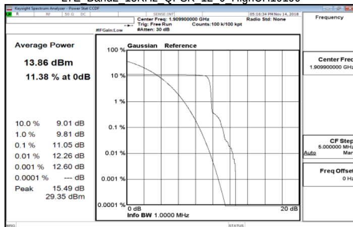
LTE Band2 15KHz QPSK 12 0 HighCH19199
