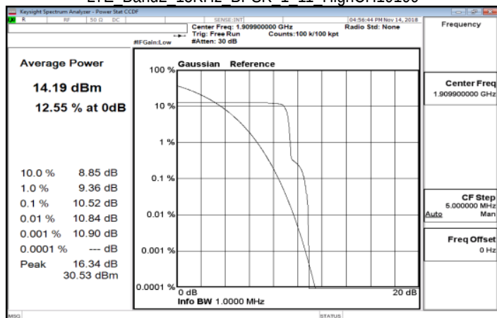
LTE Band2 15KHz BPSK 1 11 HighCH19199
