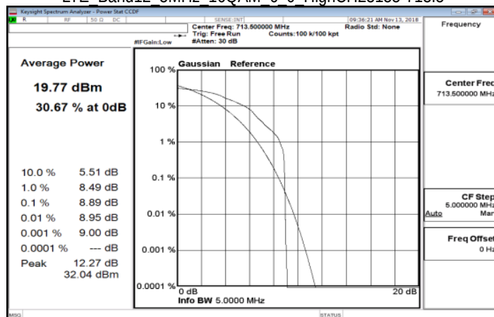
LTE Band12 5MHz 16QAM 6 0 HighCH23155-713.5
