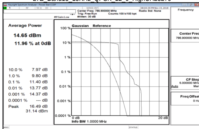
LTE Band13 15KHz QPSK 12 0 HighCH23279
