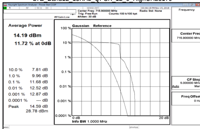
LTE Band12 15KHz QPSK 12 0 HighCH23179
