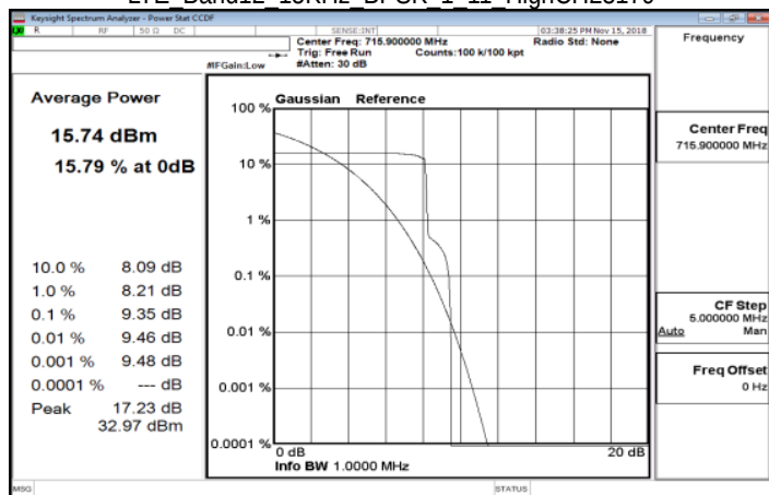
LTE Band12 15KHz BPSK 1 11 HighCH23179
