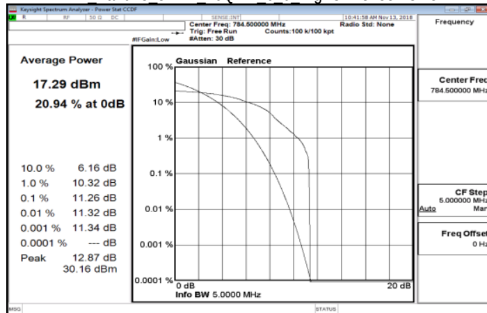
LTE Band13 5MHz 16QAM 6 0 HighCH23255-784.5
