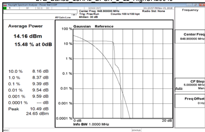
LTE Band5 15KHz BPSK 1 11 HighCH20649
