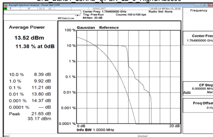
LTE Band4 15KHz QPSK 12 0 HighCH20399
