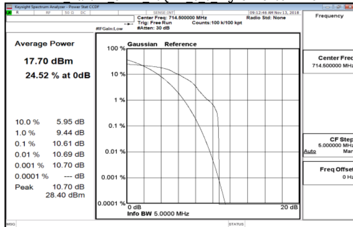
LTE Band12 3MHz 16QAM 6 0 HighCH23165-714.5
