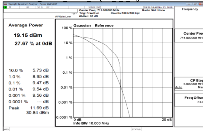
LTE Band12 10MHz 16QAM 6 0 HighCH23130-711
