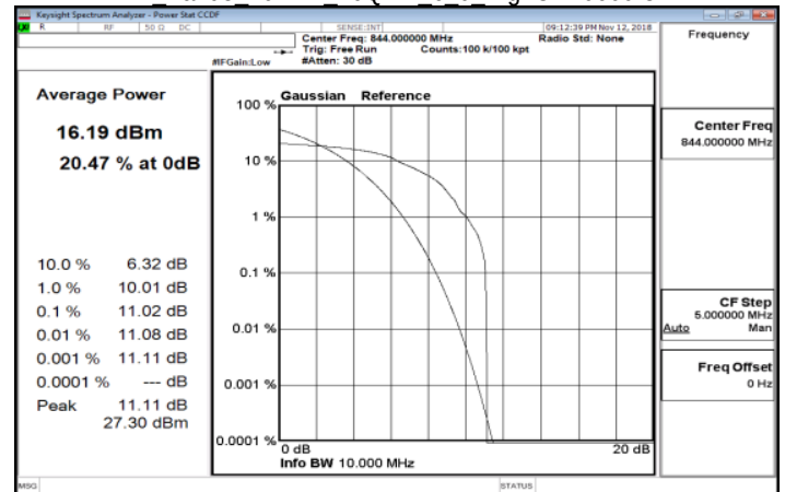
LTE Band5 10MHz 16QAM 6 0 HighCH20600-844
