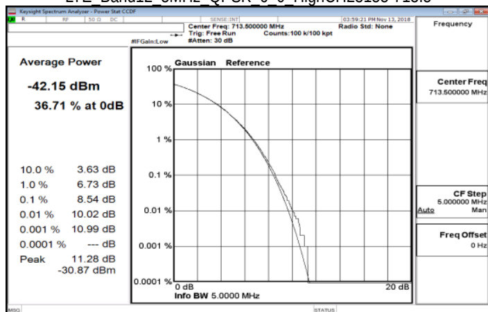
LTE Band12 5MHz QPSK 6 0 HighCH23155-713.5
