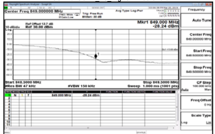
HSUPA\HSUPA B5 HighCH4233-846.6
