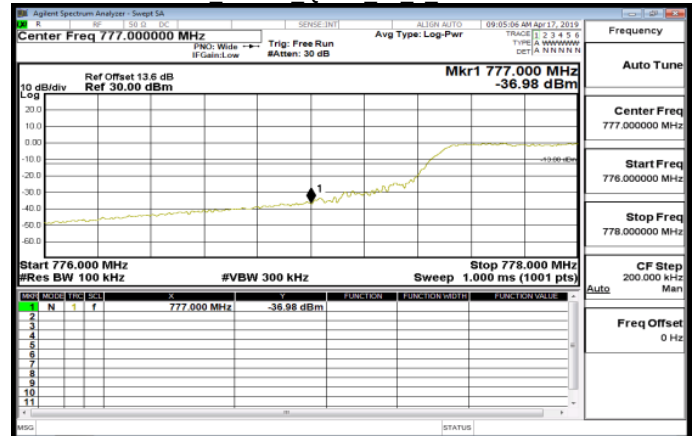
LTE\Band13 10MHz QPSK 50 0 LowCH23230-782
