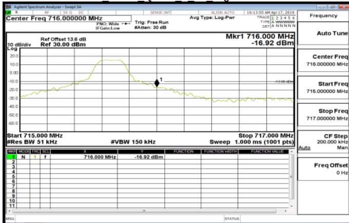
LTE\Band17 5MHz QPSK 1 24 HighCH23825-713.5
