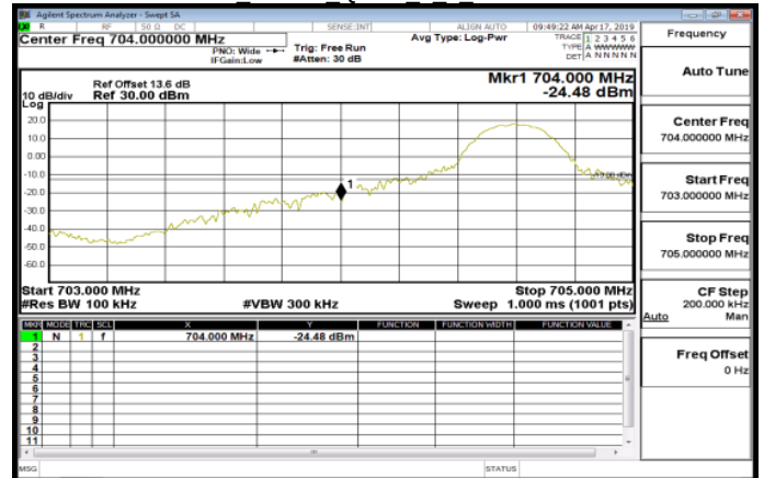
LTE\Band17 10MHz QPSK 1 0 LowCH23780-709
