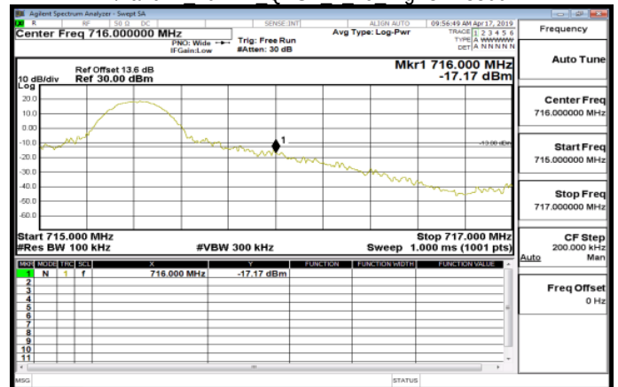
LTE\Band17 10MHz QPSK 1 49 HighCH23800-711
