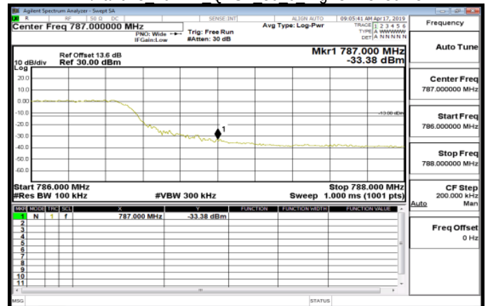
LTE\Band13 10MHz QPSK 50 0 HighCH23230-782
