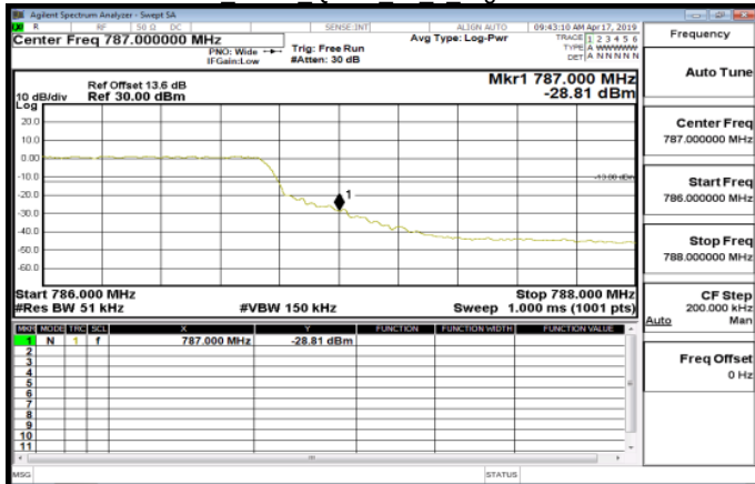
LTE\Band13 5MHz QPSK 25 0 HighCH23255-784.5
