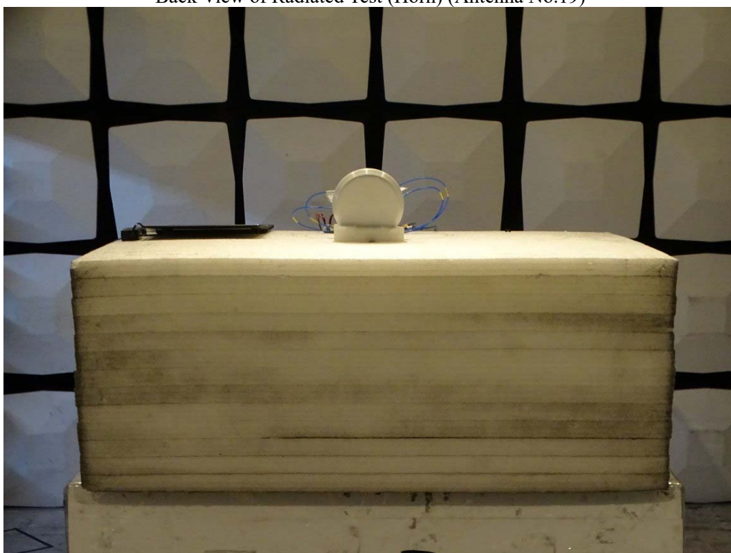
Back View of Radiated Test (Horn) (Antenna No.19)
