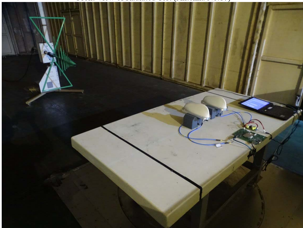
Front View of Radiated Test (Antenna No.17)
