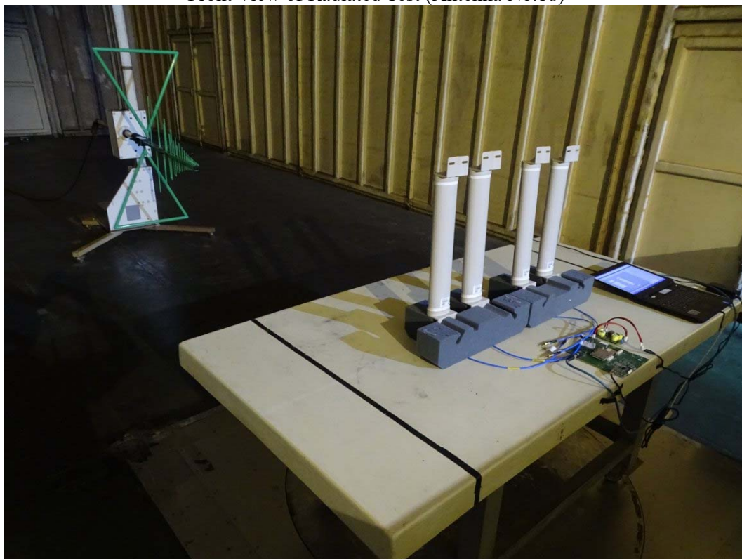
Front View of Radiated Test (Antenna No.18)
