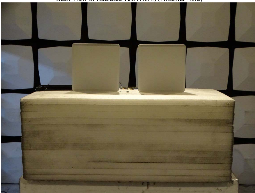
Back View of Radiated Test (Horn) (Antenna No.2)
