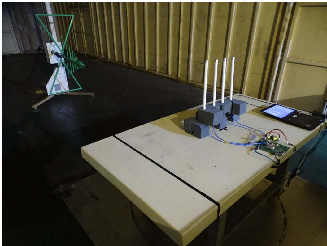
Front View of Radiated Test (Antenna No.7)
