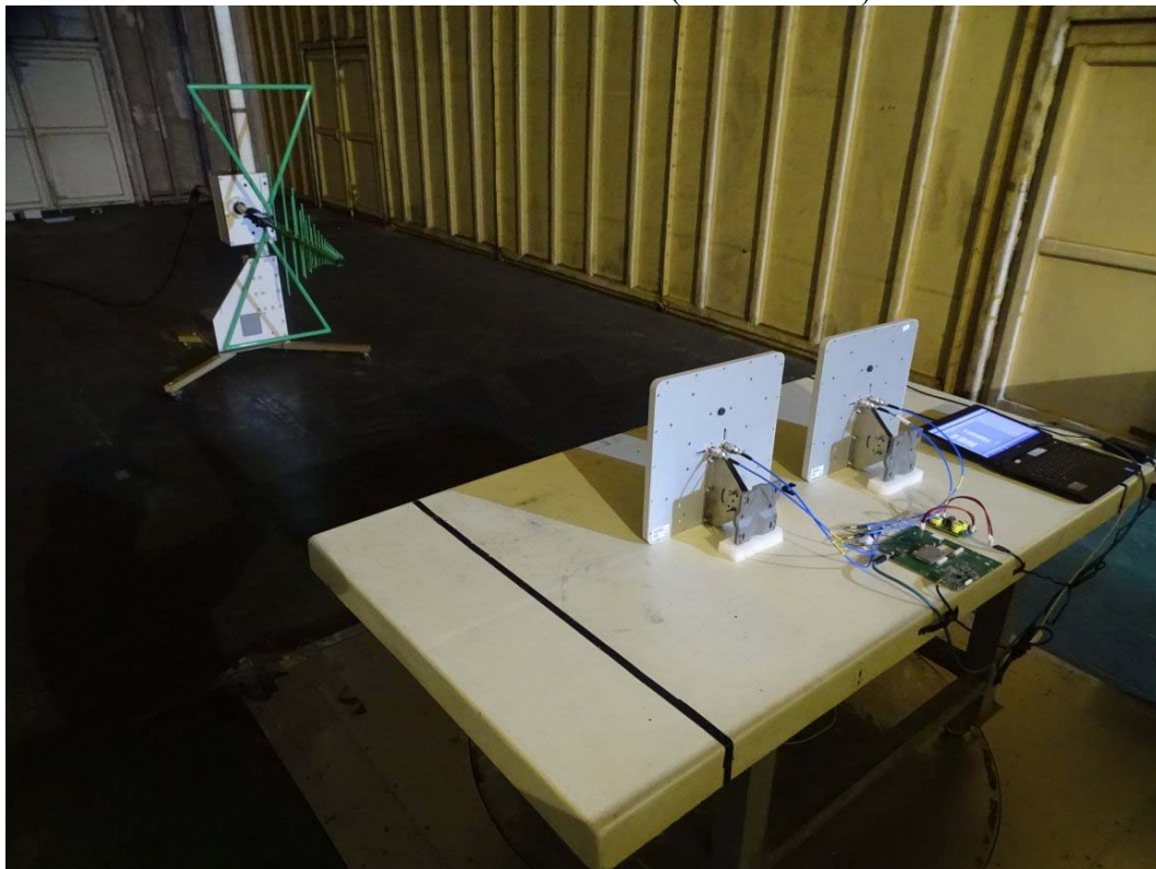
Front View of Radiated Test (Antenna No.2)
