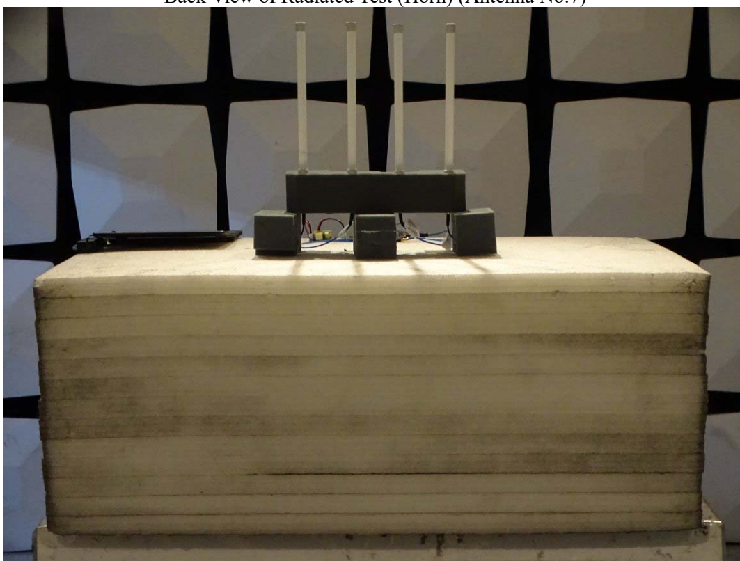
Back View of Radiated Test (Horn) (Antenna No.7)
