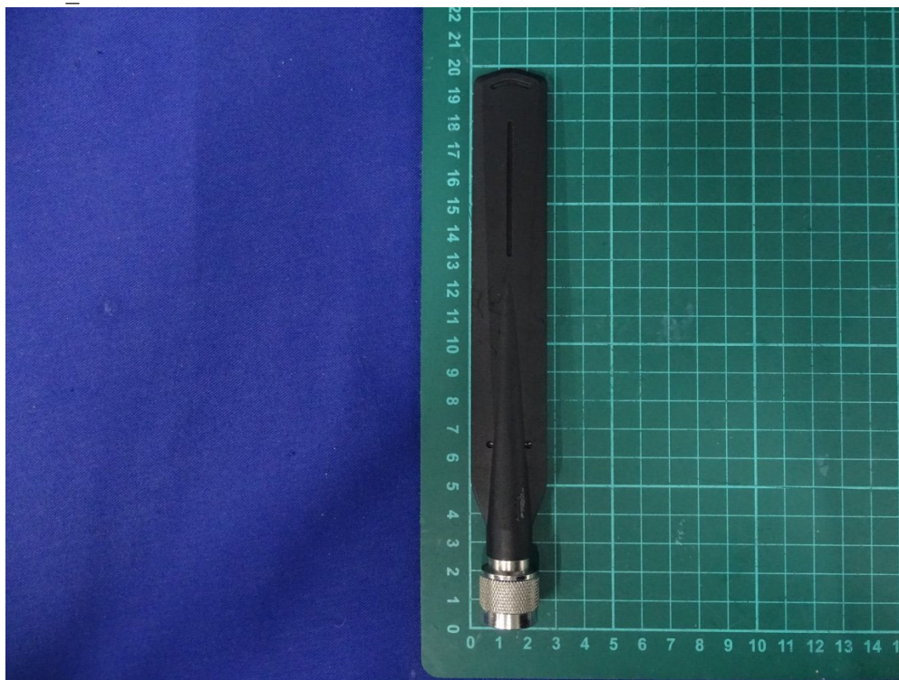
(10) EUT Photo_ Antenna: MOXA / ANT-WDB-ANM-0502
