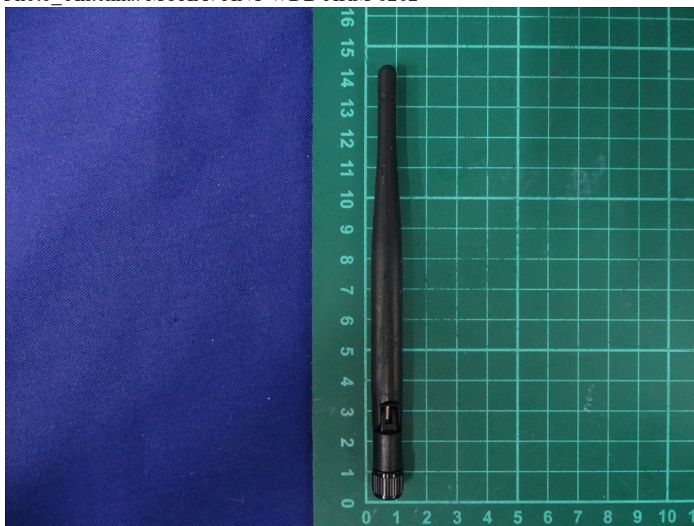
(17) EUT Photo_ Antenna: MOXA / ANT-WDB-ARM-0202
