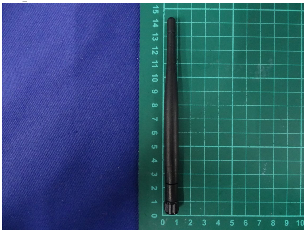
(16) EUT Photo_ Antenna: MOXA / ANT-WDB-ARM-0202
