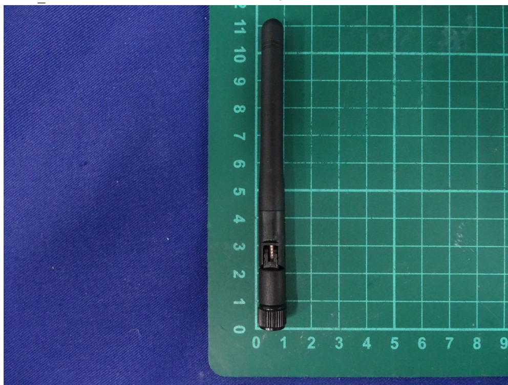
(14) EUT Photo_ Antenna: MOXA / ANT-WDB-ARM-02
