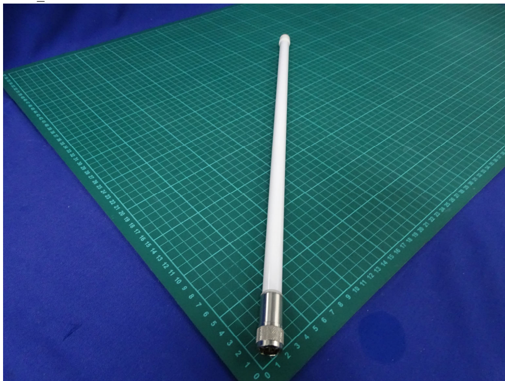
(31) EUT Photo_ Antenna: MOXA / ANT-WDB-ONM-0707
