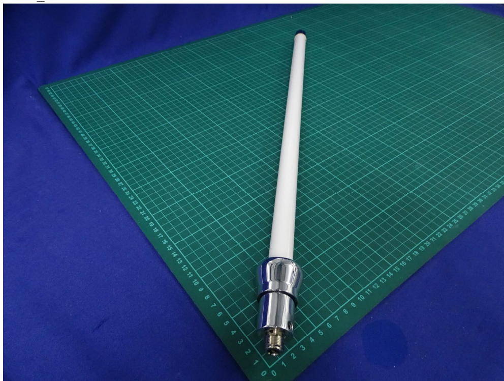
(35) EUT Photo_ Antenna: MOXA / ANT-WDB-ONF-0709
