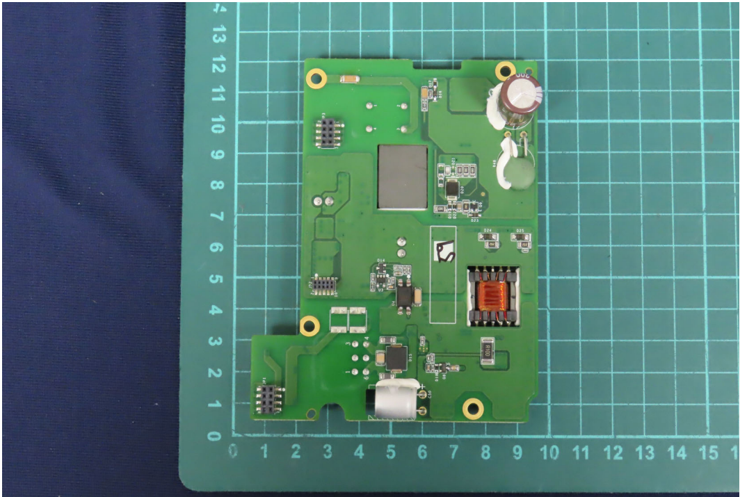
(7) EUT Photo
