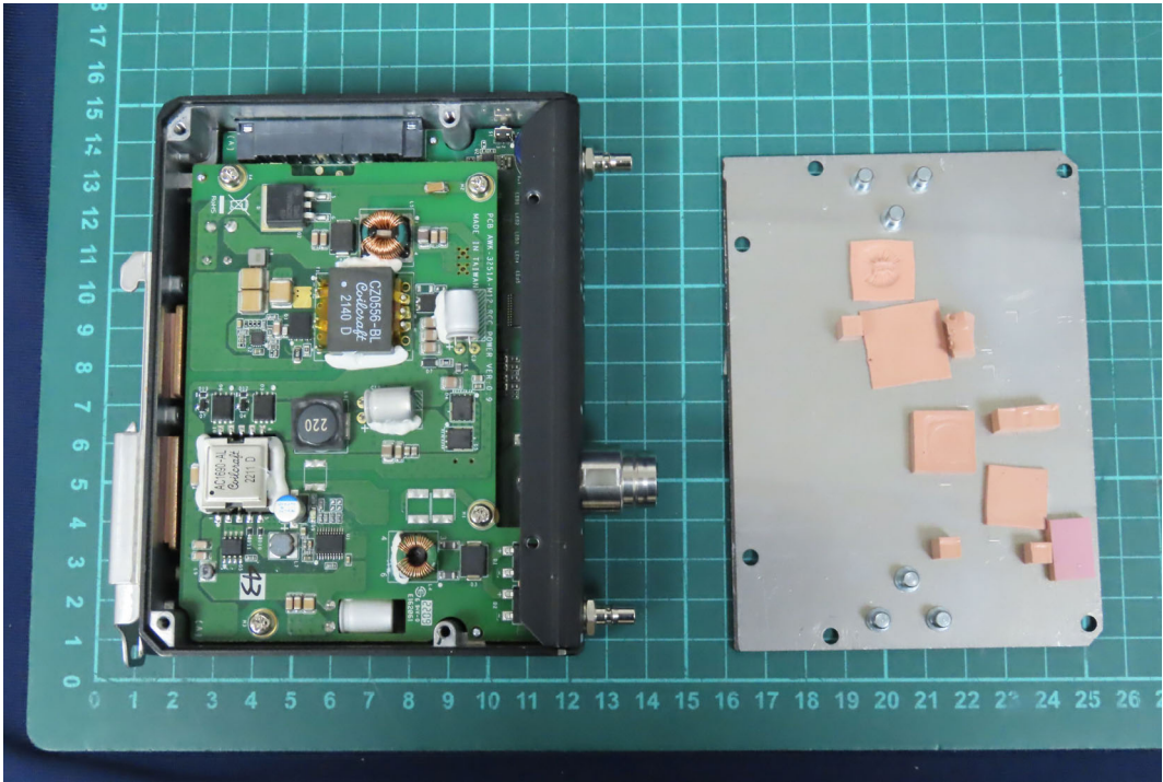
(1) EUT Photo
