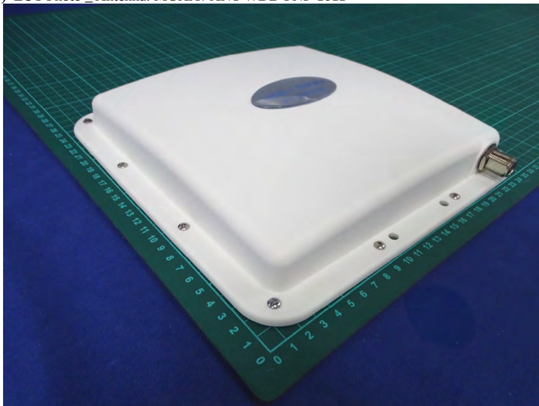
(38) EUT Photo _ Antenna: MOXA / ANT-WDB-PNF-1011
