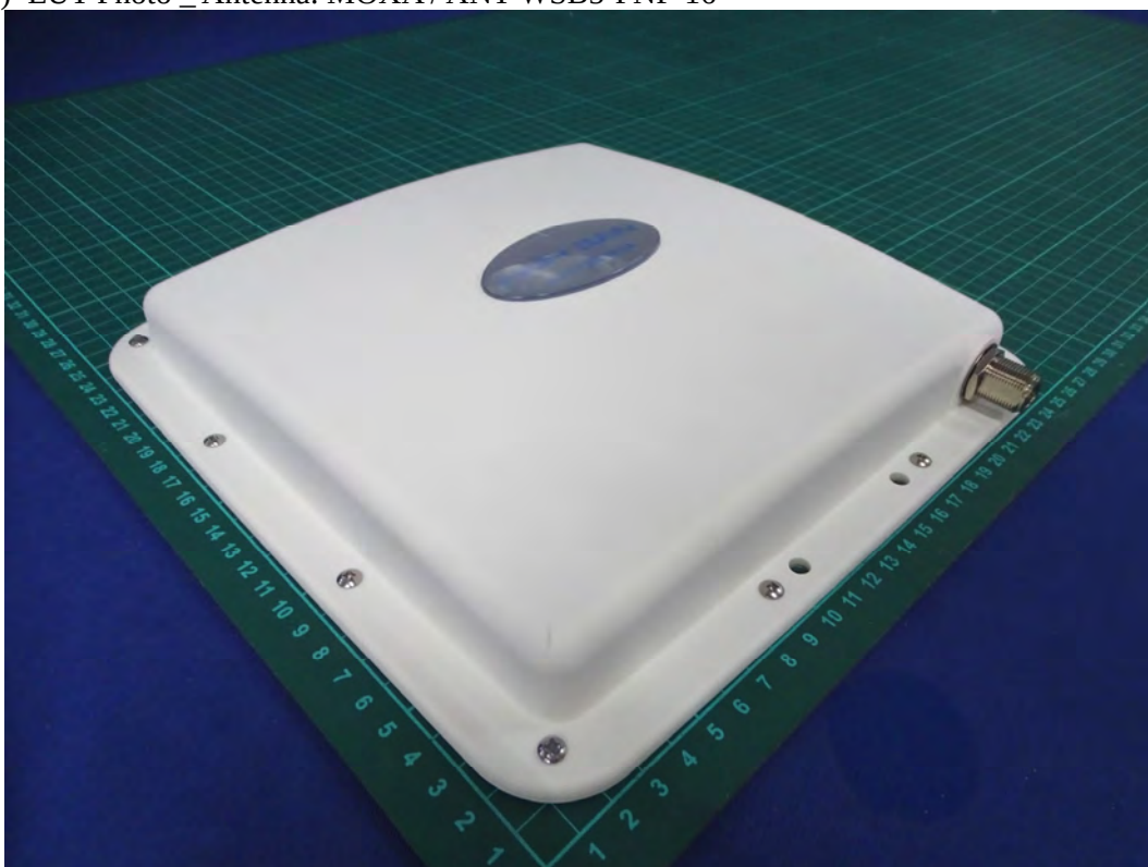
(46) EUT Photo _ Antenna: MOXA / ANT-WSB5-PNF-16
