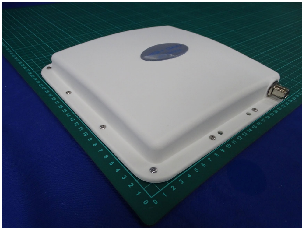
(37) EUT Photo_ Antenna: MOXA / ANT-WDB-PNF-1011
