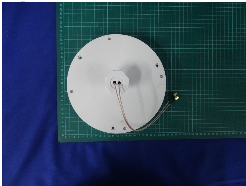
(29) EUT Photo_ Antenna: MOXA / MAT-WDB-CA-RM-2-0205
