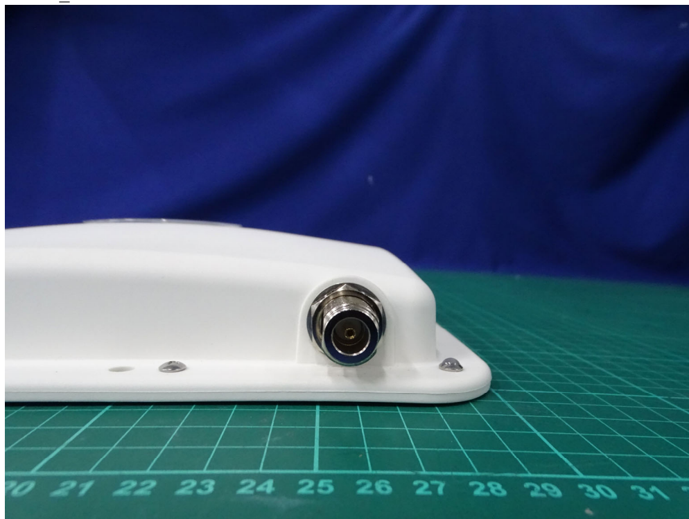
(39) EUT Photo_ Antenna: MOXA / ANT-WDB-PNF-1011
