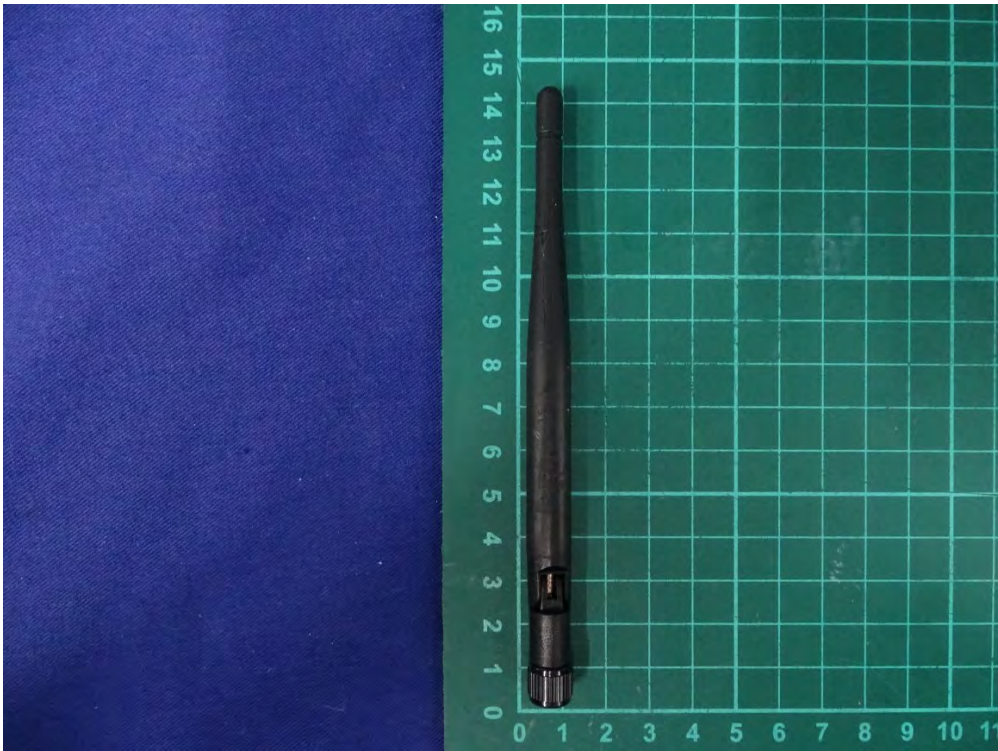
(38) EUT Photo_ Antenna: MOXA / ANT-WDB-ARM-0202
