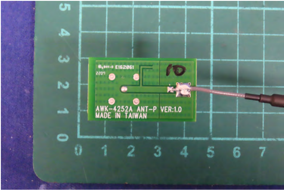
(27) EUT Photo
