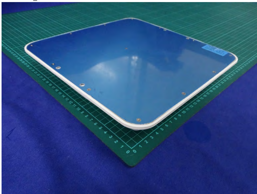
(53) EUT Photo_ Antenna: MOXA / ANT-WDB-PNF-1011
