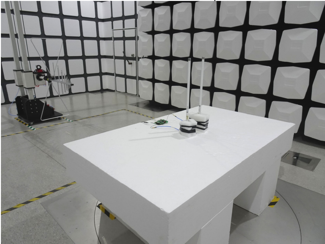
Front View of Radiated Test - Dipole
