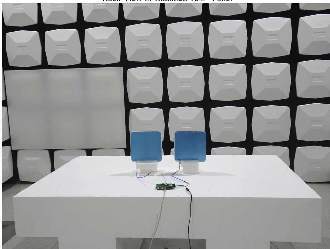
Back View of Radiated Test - Panel
