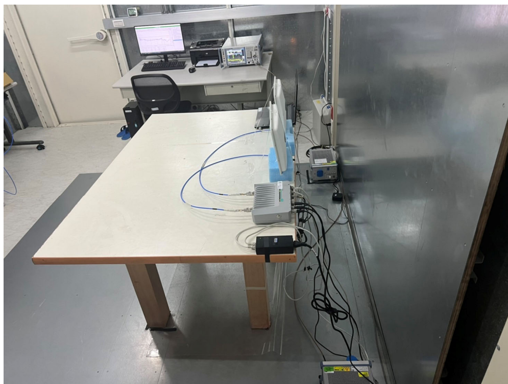
Front View of Conducted Test - Panel
