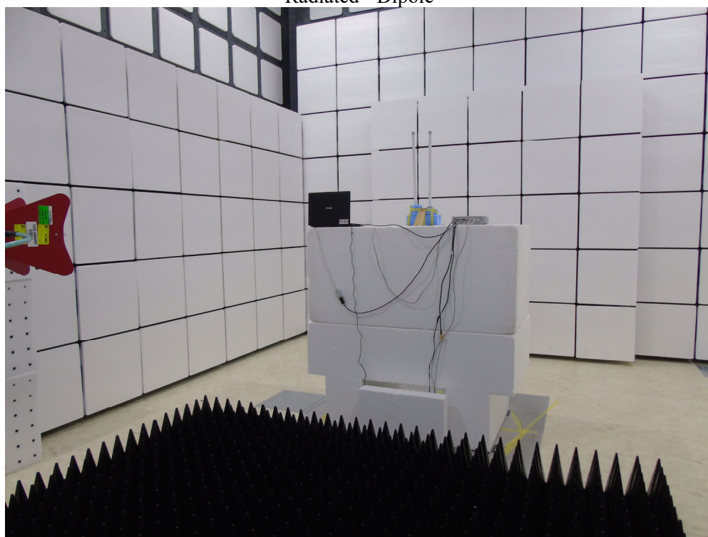
Radiated - Dipole
