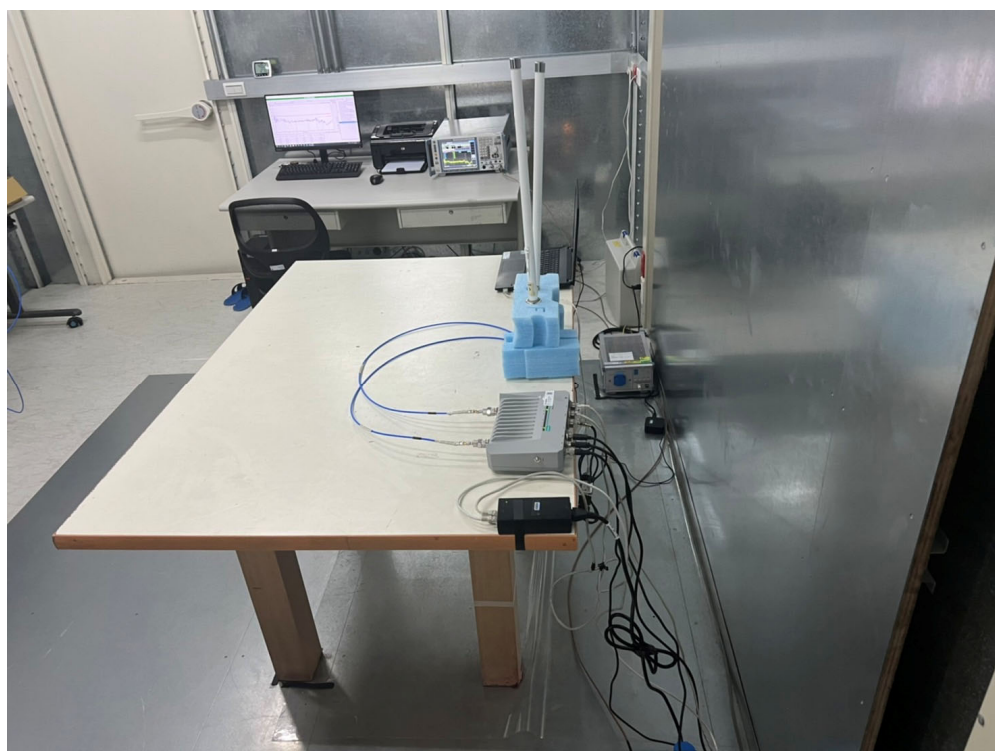
Front View of Conducted Test - Dipole
