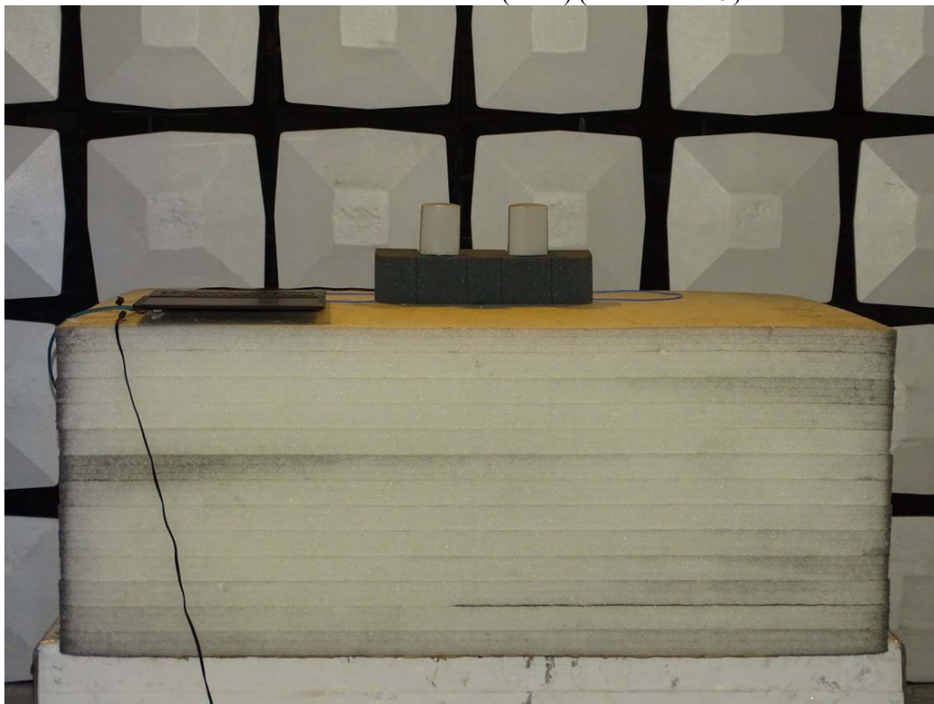
Back View of Radiated Test (Horn) (Antenna No.9)
