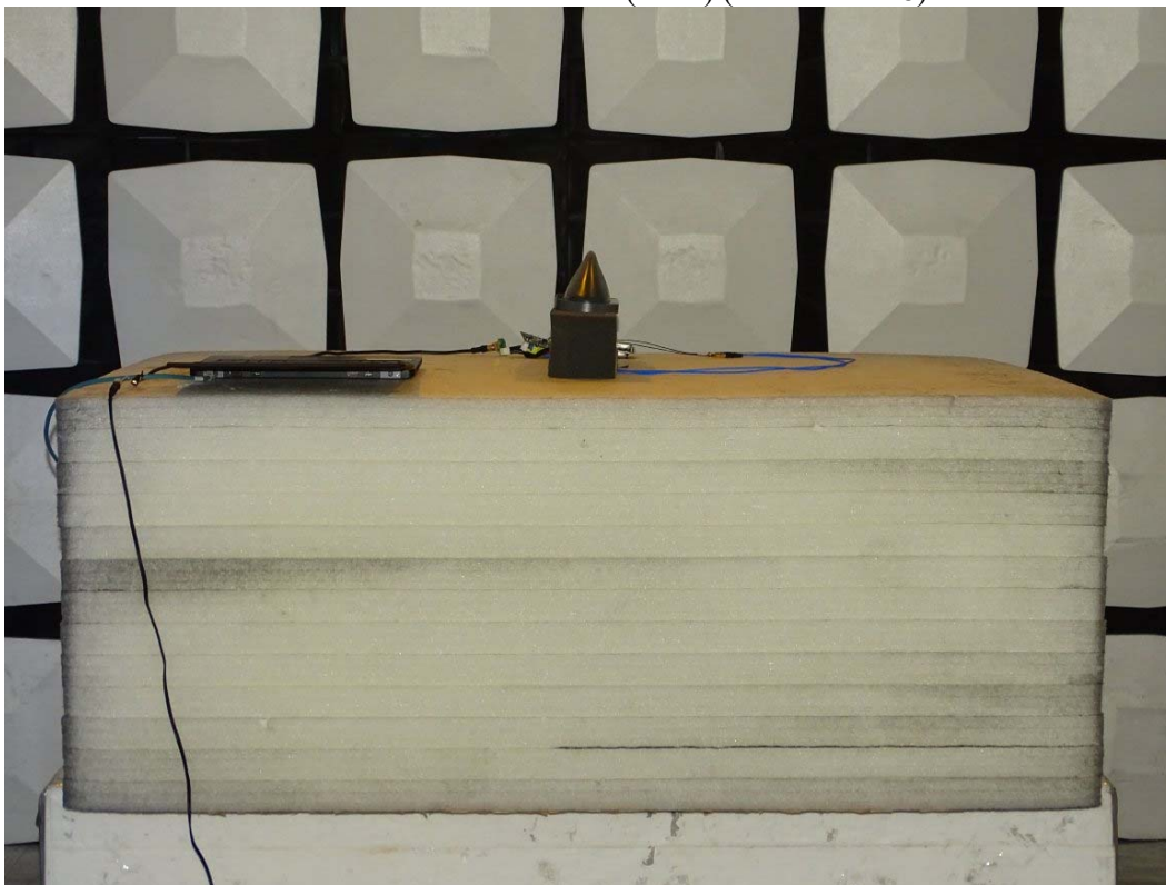
Back View of Radiated Test (Horn) (Antenna No.8)
