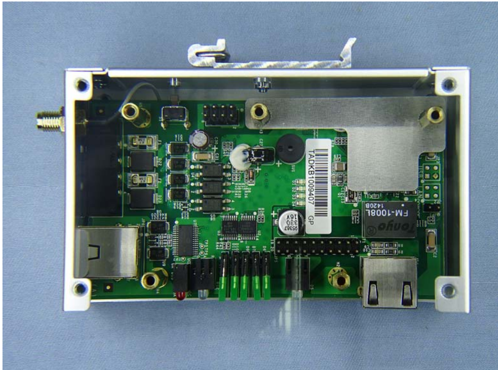
(11) EUT Photo
