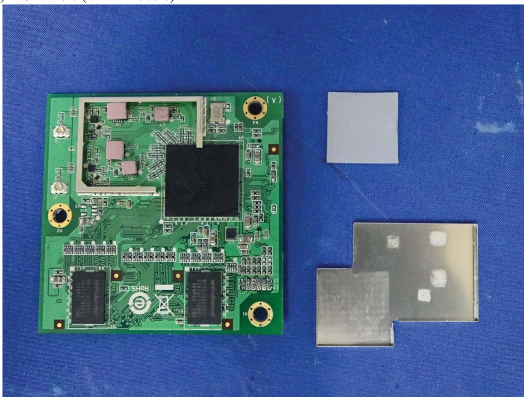
(28) EUT Photo (Wi-Fi Module)
