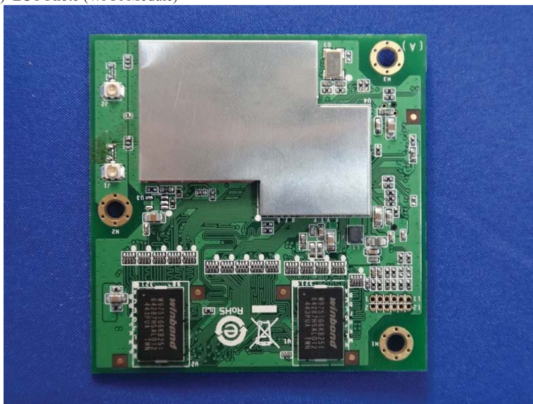
(24) EUT Photo (Wi-Fi Module)
