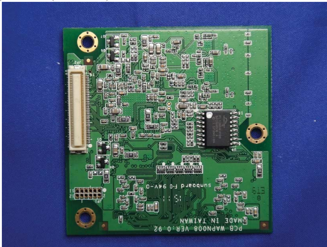
(25) EUT Photo (Wi-Fi Module)
