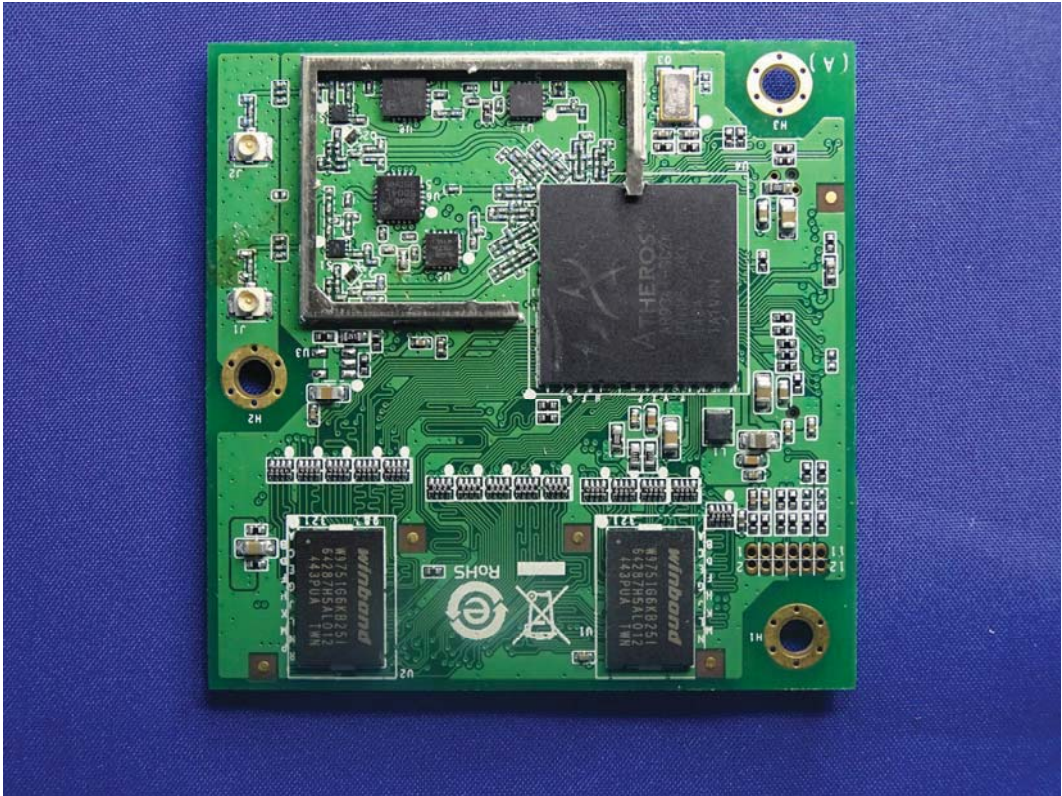
(29) EUT Photo (Wi-Fi Module)
