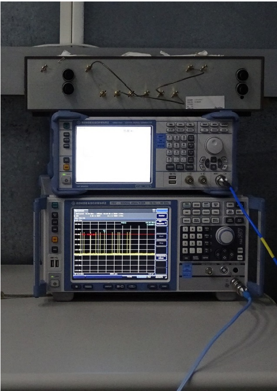
DFS Set-up Photo: Spectrum Analyzer and Radar Generator
