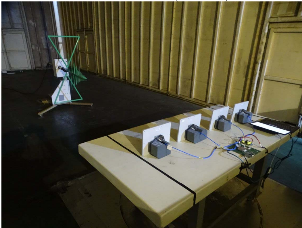
Back View of Radiated Test (Antenna No.1)
