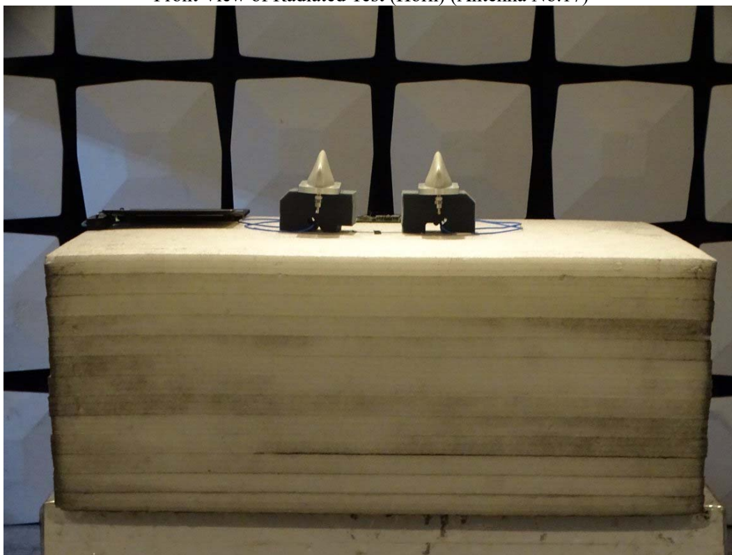
Front View of Radiated Test (Horn) (Antenna No.17)
