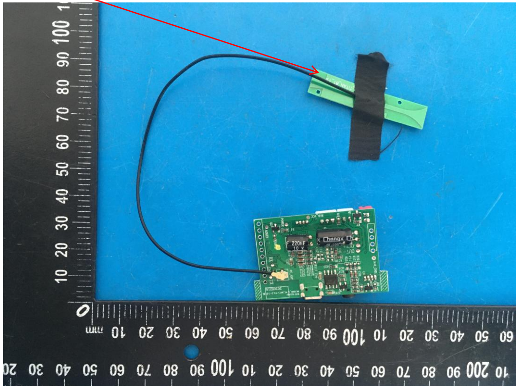
BT antenna
