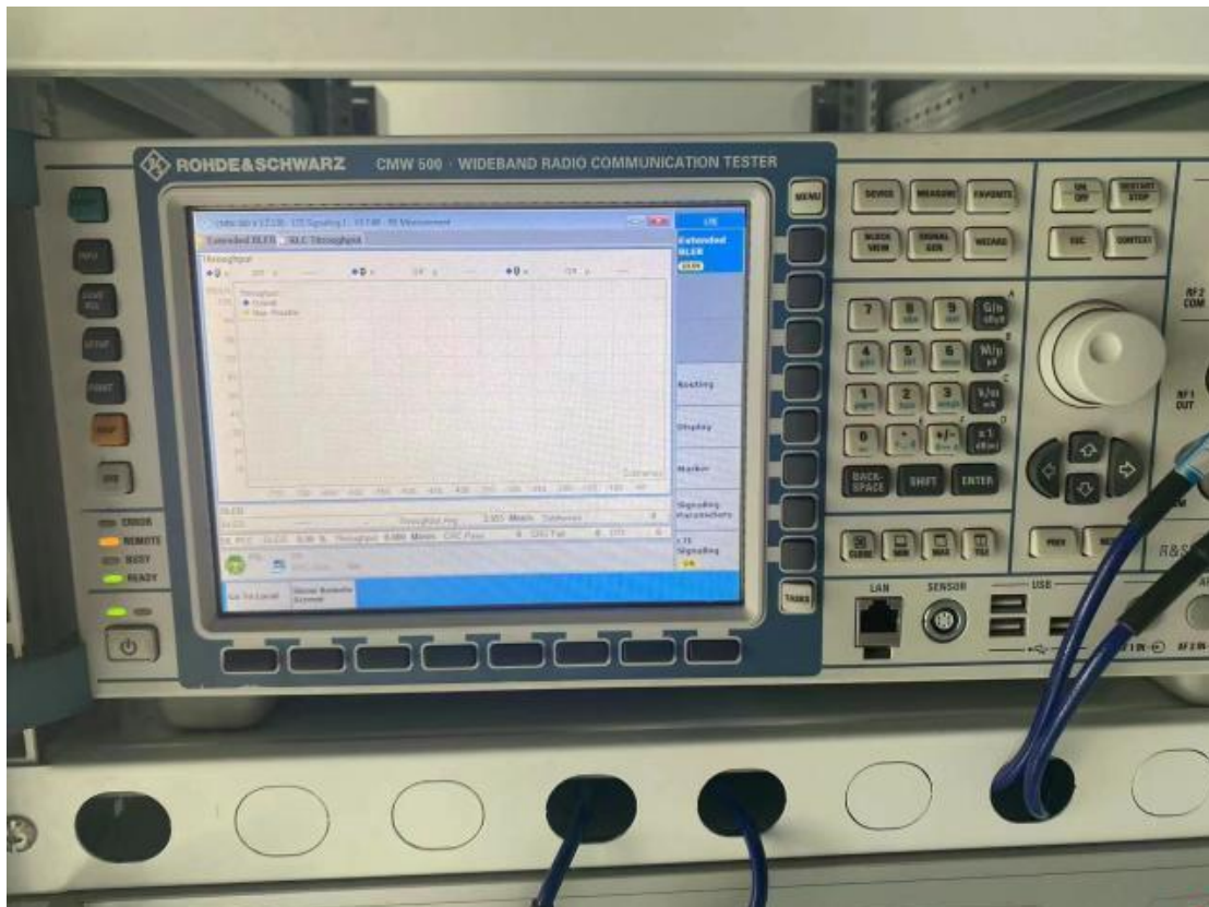
Test instrumentation
