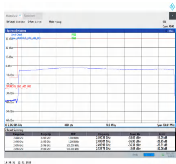
1-N41-PC3-30-100-L-6-CP-QPSK-Outer_Full-273@0-Ant1-1--PASS-see graph
