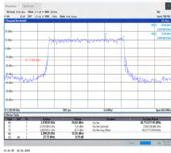
1-N41-PC3-30-30-M-2-DFT-PI2BPSK-Outer_Full-75 @0-Ant1-26.713-27.720-≤30-PASS
