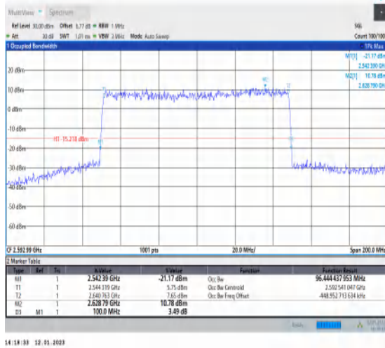
1-N41-PC3-30-100-M-3-DFT-16QAM-Outet_Full-270 @0-Ant1-96.444-100.000-≤100-PASS
