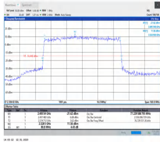
1-N41-PC3-30-80-L-7-CP-16QAM-Outer_Full-217@0-Ant1-77.23-80.800-≤80-PASS
