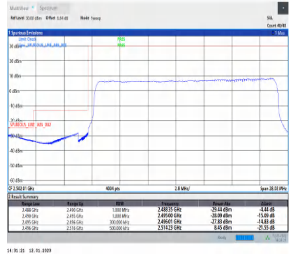
1-N41-PC3-30-20-L-3-DFT-PI2BPSK-Outer_Full-50@0-Ant1-1--PASS-see graph
