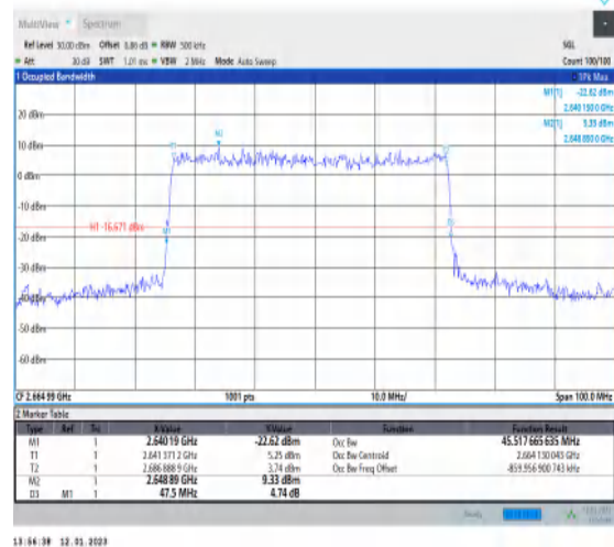
1-N41-PC3-30-50-H-5-DFT-256QAM-Outer_Full-128 @0-Ant1-45.518-47.500-≤50-PASS
