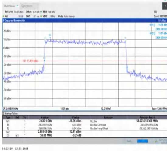
1-N41-PC3-30-60-H-3-DFT-16QAM-Outer_Full-162 @0-Ant1-58.023-59.880-≤60-PASS
