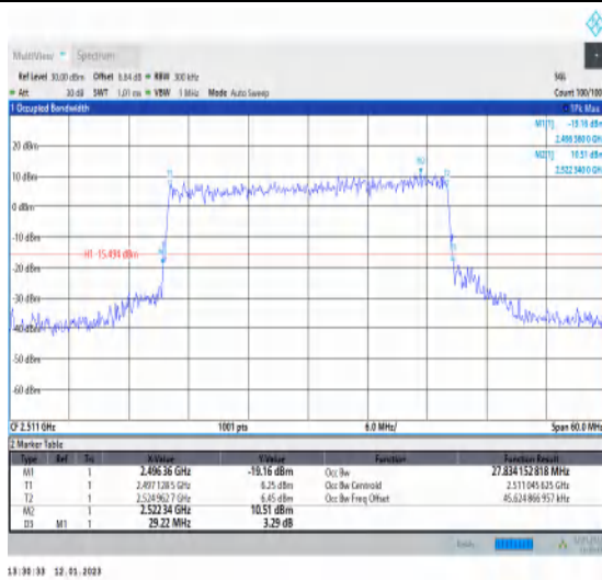
1-N41-PC3-30-30-L-6-CP-QPSK-Outer_Full-78@0-A Ant1-27.834-29.220-≤30-PASS
