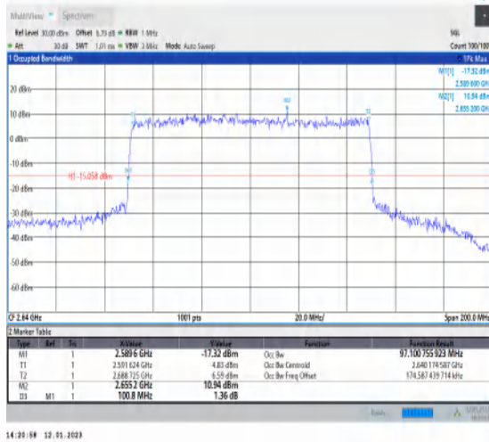
1-N41-PC3-30-100-H-6-CP-QPSK-Outer_Full-273@ 0-Ant1-97.101-100.800≤100-PASS
