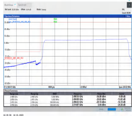
1-N41-PC3-30-20-L-6-CP-QPSK-Outer_Full-51@0-Ant1-1--PASS-see graph
