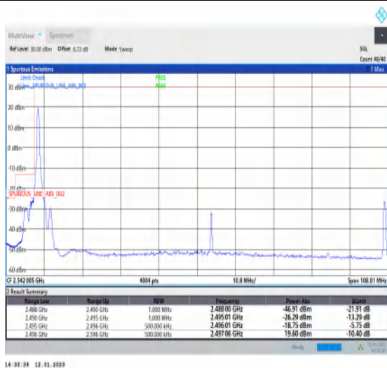
1-N41-PC3-30-100-L-4-CP-QPSK-Edge_1RB_Left-1@0-Ant1-1--PASS-see graph
