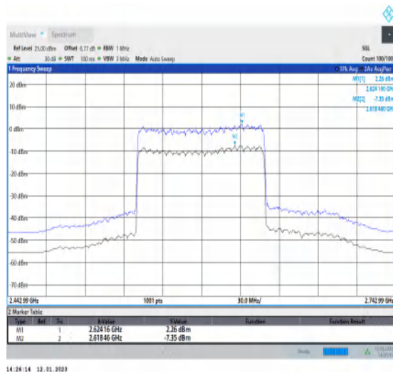
1-N41-PC3-30-100-M-1-DFT-256QAM-Outer_Full-27 0@0-Ant1-9.61-100%-0.00-9.61-PASS-≤13
