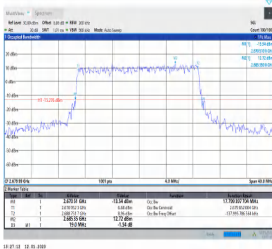
1-N41-PC3-30-20-H-1-DFT-QPSK-Outer_Full-50@0- Ant1-17.799-19.000-≤20-PASS
