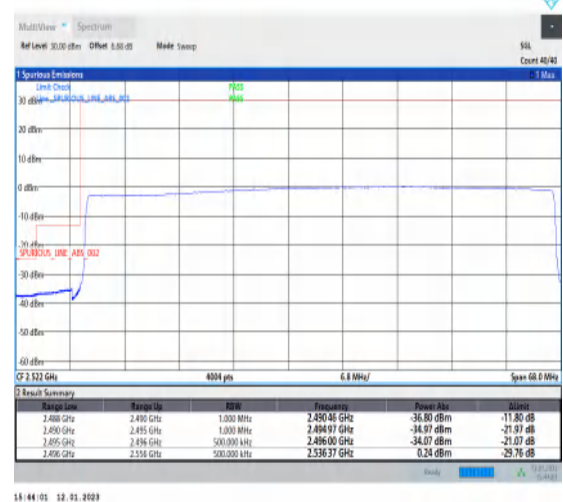
1-N41-PC3-30-60-L-6-CP-QPSK-Outer_Full-162@0-Ant1-1--PASS-see graph
