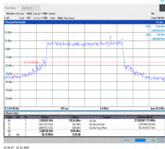
1-N41-PC3-30-30-H-7-CP-16QAM-Outer_Full-78@0- Ant1-27.93-30.180-≤30-PASS
