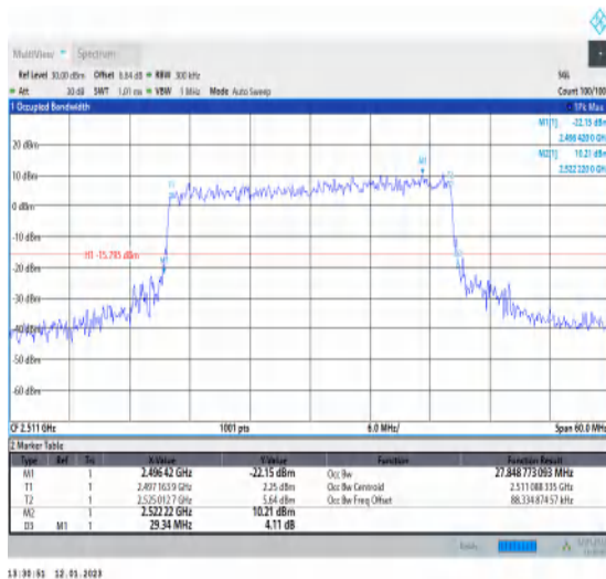
1-N41-PC3-30-30-L-8-CP-64QAM-Outer_Full-78@0- Ant1-27.849-29.340-≤30-PASS
