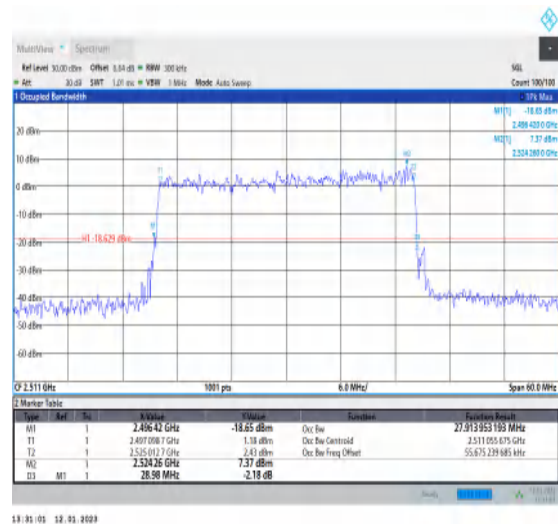
1-N41-PC3-30-30-L-9-CP-256QAM-Outer_Full-78@0- Ant1-27.914-28.980-≤30-PASS
