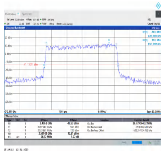
1-N41-PC3-30-30-L-1-DFT-QPSK-Outer_Full-75@0- Ant1-26.78-28.320-≤30-PASS
