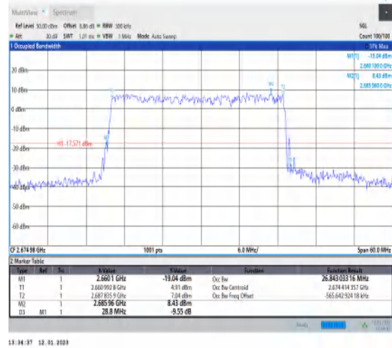
1-N41-PC3-30-30-H-5-DFT-256QAM-Outer_Full-75@ 0-Ant1-26.843-28.800-≤30-PASS
