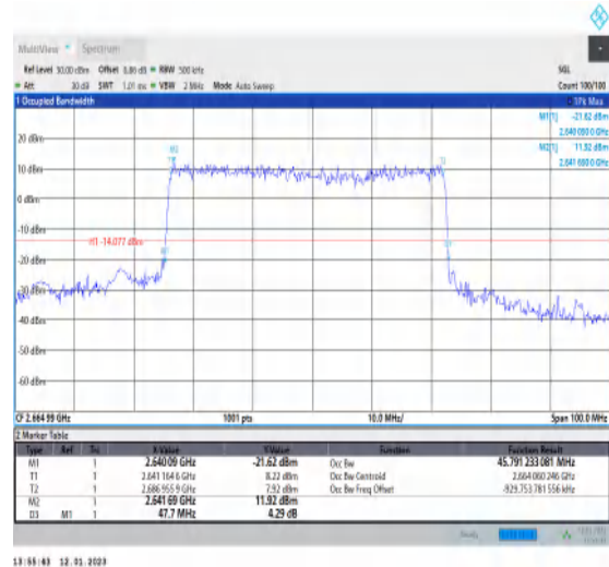
1-N41-PC3-30-50-H-1-DFT-QPSK-Outer_Full-128@ 0-Ant1-45.791-47.700-≤50-PASS
