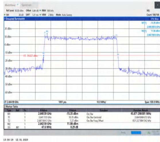
1-N41-PC3-30-50-H-3-DFT-16QAM-Outer_Full-128 @0-Ant1-45.871-47.600-≤50-PASS
