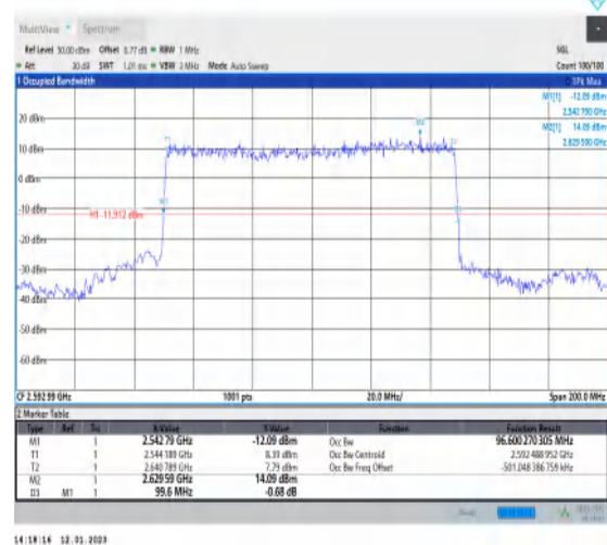
1-N41-PC3-30-100-M-2-DFT-PI2BPSK-Outer_Full-270 @0-Ant1-96.6-99.600-≤100-PASS
