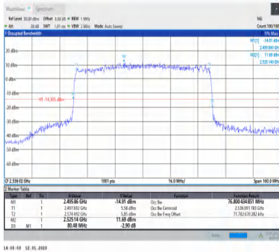
1-N41-PC3-30-80-L-6-CP-QPSK-Outer_Full-217@0-Ant1-76.8-80.480-≤80-PASS
