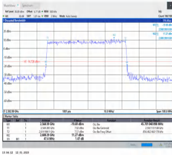
1-N41-PC3-30-50-M-3-DFT-16QAM-Outer_Full-128 @0-Ant1-45.701-47.400-≤50-PASS
