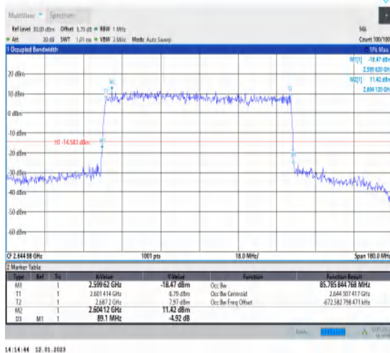
1-N41-PC3-30-90-H-3-DFT-16QAM-Outer_Full-240@0-Ant1-85.786-89.100-≤90-PASS
