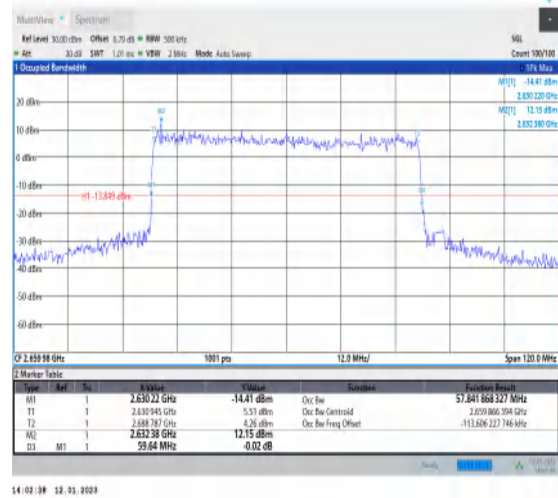
1-N41-PC3-30-60-H-4-DFT-64QAM-Outer_Full-162 @0-Ant1-57.842-59.640-≤60-PASS
