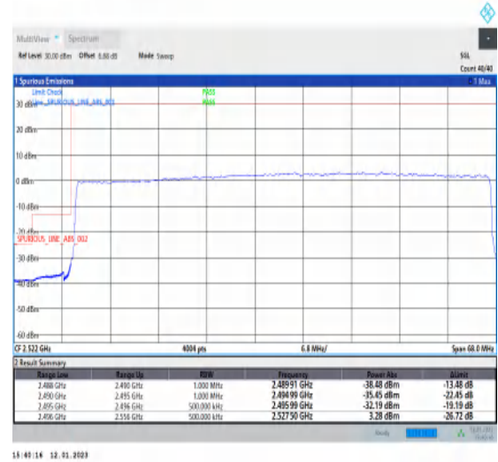
1-N41-PC3-30-60-L-3-DFT-PI2BPSK-Outer_Full-162@0-Ant1-1--PASS-see graph
