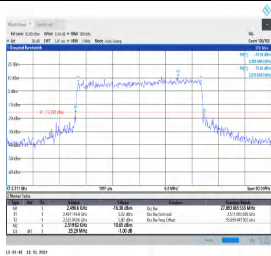
1-N41-PC3-30-30-L-7-CP-16QAM-Outer_Full-78@0- Ant1-27.894-29.280-≤30-PASS
