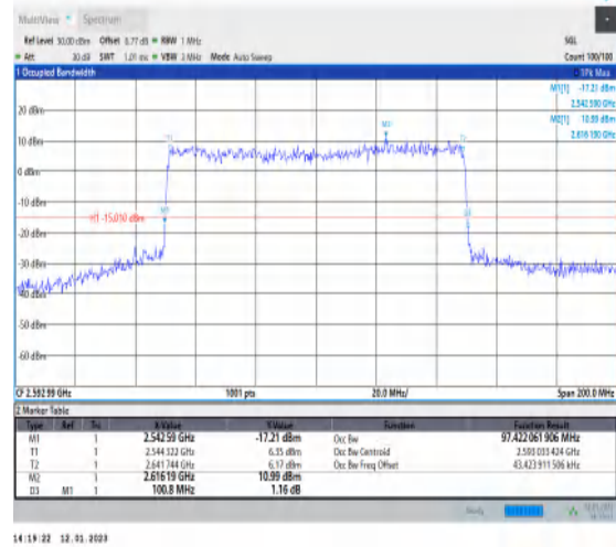
1-N41-PC3-30-100-M-8-CP-64QAM-Outer_Full-273 @0-Ant1-97.422-100.800-≤100-PASS
