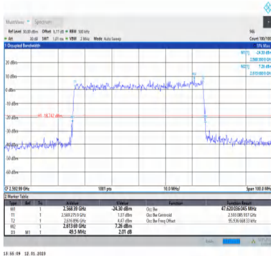
1-N41-PC3-30-50-M-9-CP-256QAM-Outer_Full-133 @0-Ant1-47.62-49.500-≤50-PASS
