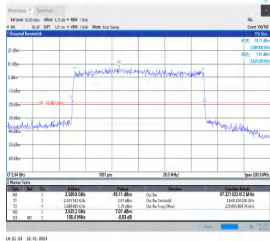
1-N41-PC3-30-100-H-9-CP-256QAM-Outer_Full-273 @0-Ant1-97.322-100.400≤100-PASS
