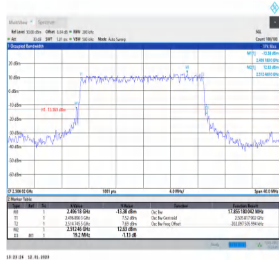
1-N41-PC3-30-20-L-2-DFT-PI2BPSK-Outer_Full-50@-Ant1-17.855-19.200-≤20-PASS
