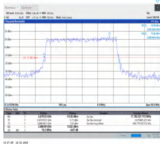
1-N41-PC3-30-20-H-2-DFT-PI2BPSK-Outer_Full-50 @0-Ant1-17.782-19.200-≤20-PASS
