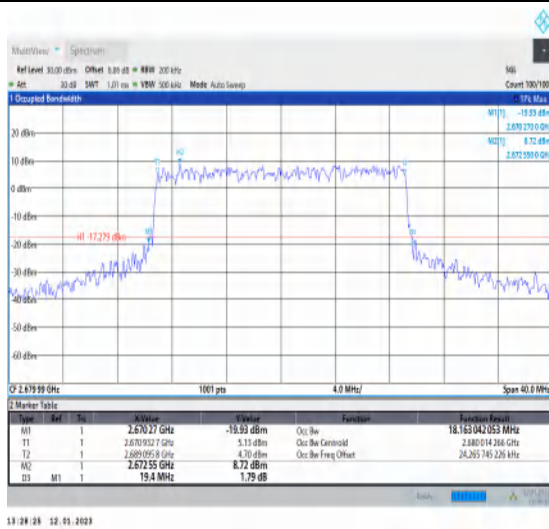
1-N41-PC3-30-20-H-7-CP-16QAM-Outer_Full-51@0 -Ant1-18.163-19.400-≤20-PASS
