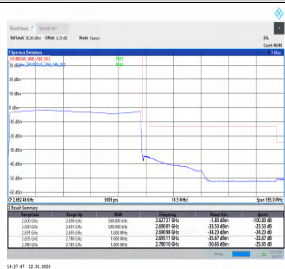
1-N41-PC3-30-90-H-6-CP-QPSK-Outer_Full-245 @0-Ant1-1--PASS-see graph
