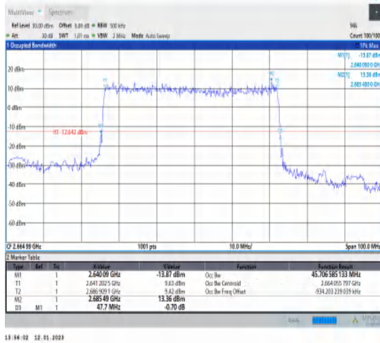
1-N41-PC3-30-50-H-2-DFT-PI2BPSK-Outer_Full-128 @0-Ant1-45.707-47.700-≤50-PASS
