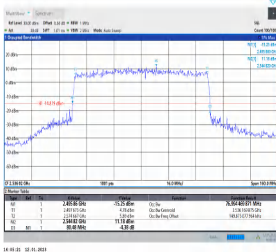
1-N41-PC3-30-80-L-8-CP-64QAM-Outer_Full-217@0-Ant1-76.994-80.480-≤80-PASS
