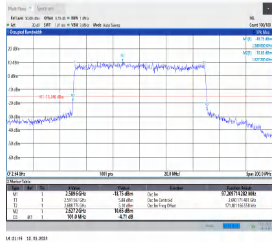
1-N41-PC3-30-100-H-7-CP-16QAM-Outer_Full-273 @0-Ant1-97.21-101.000≤100-PASS
