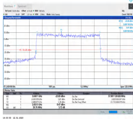
1-N41-PC3-30-60-H-6-CP-QPSK-Outer_Full-162@0 -Ant1-57.901-59.760-≤60-PASS
