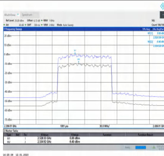
1-N41-PC3-30-100-L-2-CP-256QAM-Outer_Full-27 3@0-Ant1-9.40-100%-0.00-9.40-PASS-≤13
