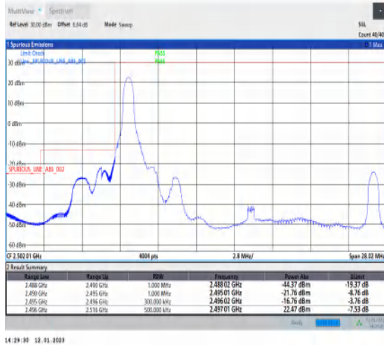
1-N41-PC3-30-20-L-1-DFT-PI2BPSK-Edge_1RB_Left-1@0-Ant1-1--PASS-see graph
