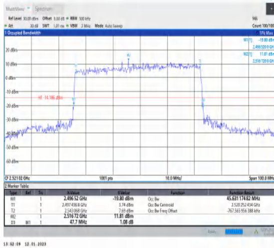
1-N41-PC3-30-50-L-4-DFT-64QAM-Outer_Full-128 @0-Ant1-45.631-47.700-≤50-PASS
