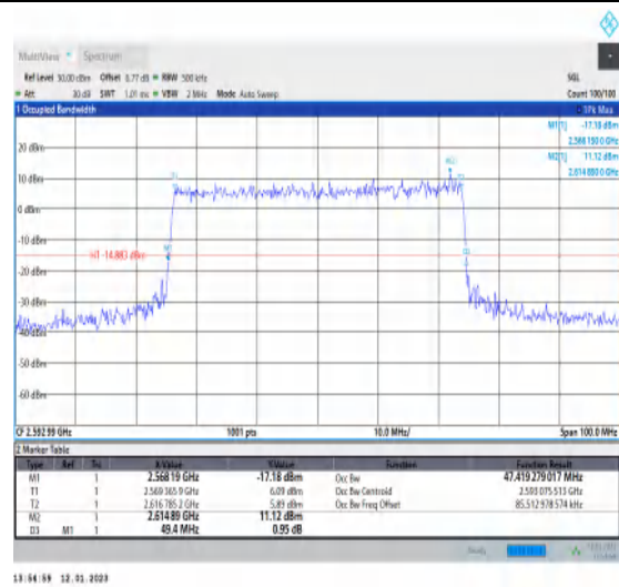
1-N41-PC3-30-50-M-8-CP-64QAM-Outer_Full-133@ 0-Ant1-47.419-49.400-≤50-PASS
