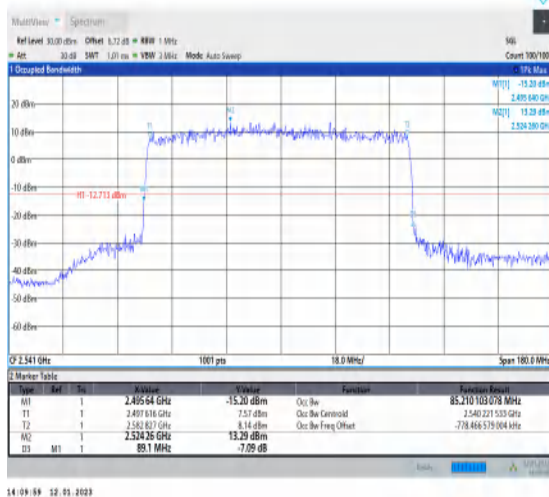
1-N41-PC3-30-90-L-1-DFT-QPSK-Outer_Full-240@0 -Ant1-85.21-89.100-≤90-PASS
