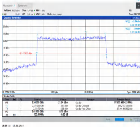
1-N41-PC3-30-100-M-9-CP-256QAM-Outer_Full-273 @0-Ant1-97.656-100.800-≤100-PASS
