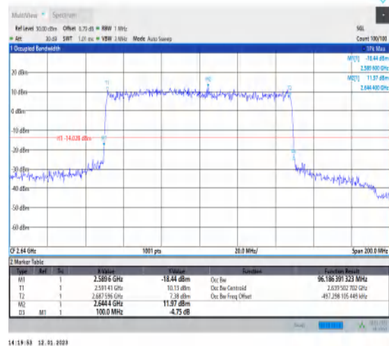
1-N41-PC3-30-100-H-1-DFT-QPSK-Outer_Full-270 @0-Ant1-96.186-100.000-≤100-PASS
