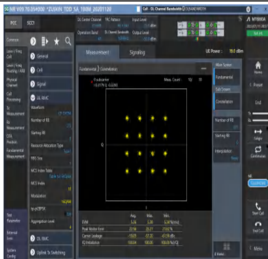
1-N41-PC3-30-100-M-7-CP-16QAM-Outer_Full-273 @0-Ant1-see graph-PASS
