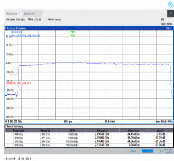
1-N41-PC3-30-100-L-3-DFT-PI2BPSK-Outer_Full-270@0-Ant1-1--PASS-see graph
