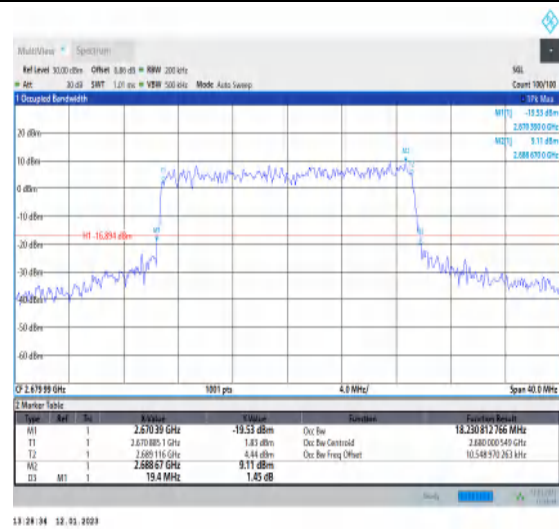
1-N41-PC3-30-20-H-8-CP-64QAM-Outer_Full-51@0 -Ant1-18.231-19.400-≤20-PASS
