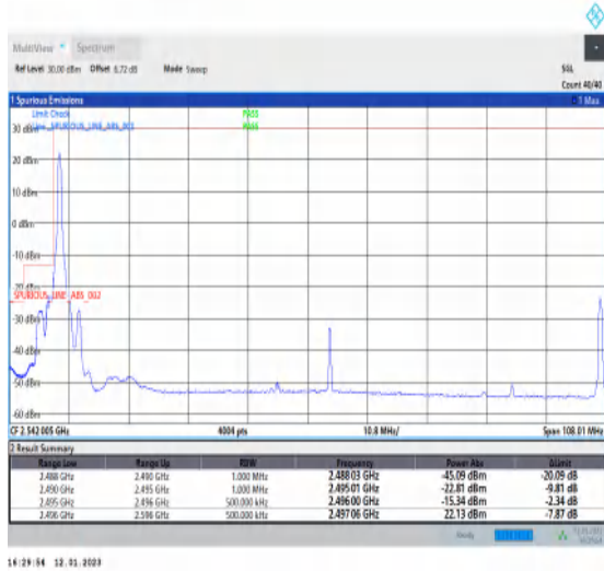
1-N41-PC3-30-100-L-1-DFT-PI2BPSK-Edge_1RB_Left-1@0-Ant1-1--PASS-see graph
