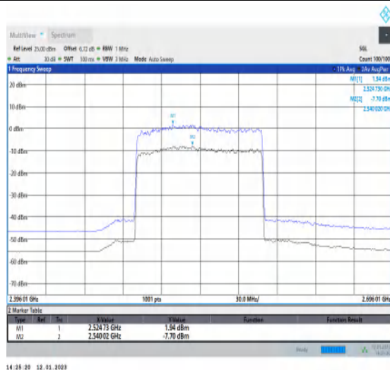
1-N41-PC3-30-100-L-1-DFT-256QAM-Outer_Full-270 @0-Ant1-9.64-100%-0.00-9.64-PASS-≤13
