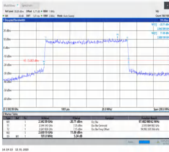
1-N41-PC3-30-100-M-7-CP-16QAM-Outer_Full-273 @0-Ant1-97.483-101.000-≤100-PASS
