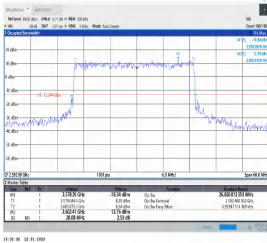
1-N41-PC3-30-30-M-1-DFT-QPSK-Outer_Full-75@0 -Ant1-26.831-28.080-≤30-PASS
