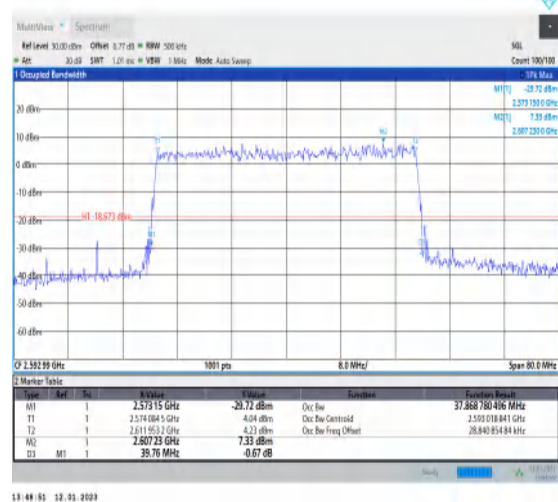
1-N41-PC3-30-40-M-9-CP-256QAM-Outer_Full-106@0-Ant1-37.869-39.760-≤40-PASS
