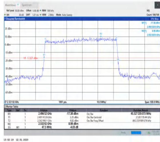
1-N41-PC3-30-50-L-5-DFT-256QAM-Outer_Full-128 @0-Ant1-45.527-47.500-≤50-PASS
