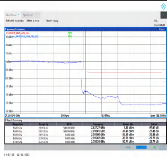
1-N41-PC3-30-90-H-3-DFT-PI2BPSK-Outer_Full-2 40@0-Ant1-1--PASS-see graph
