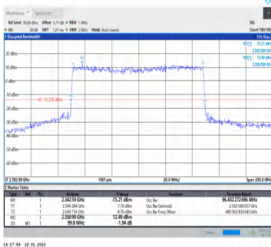
1-N41-PC3-30-100-M-1-DFT-QPSK-Outer_Full-270 @0-Ant1-96.432-99.800-≤100-PASS
