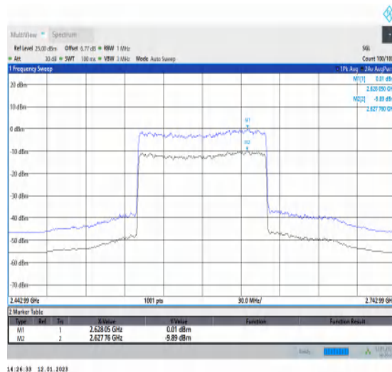
1-N41-PC3-30-100-M-2-CP-256QAM-Outer_Full-27 3@0-Ant1-9.90-100%-0.00-9.90-PASS-≤13
