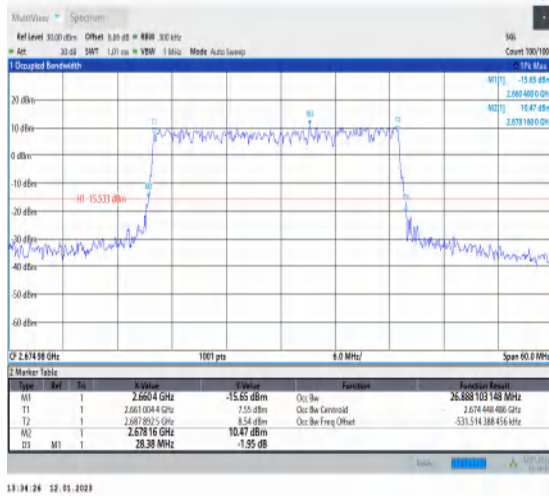
1-N41-PC3-30-30-H-4-DFT-64QAM-Outer_Full-75@ 0-Ant1-26.888-28.380-≤30-PASS
