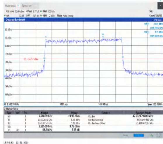
1-N41-PC3-30-50-M-6-CP-QPSK-Outer_Full-133@0-Ant1-47.532-49.200-≤50-PASS
