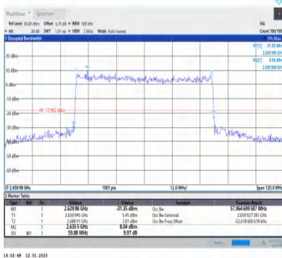
1-N41-PC3-30-60-H-5-DFT-256QAM-Outer_Full-162 @0-Ant1-57.965-59.880-≤60-PASS
