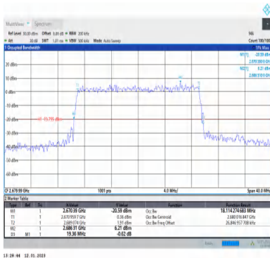
1-N41-PC3-30-20-H-9-CP-256QAM-Outer_Full-51@0 -Ant1-18.114-19.360-≤20-PASS
