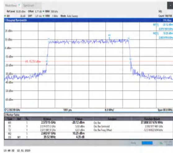
1-N41-PC3-30-40-M-7-CP-16QAM-Outer_Full-106@0-Ant1-37.809-39.520-≤40-PASS
