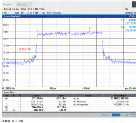
1-N41-PC3-30-40-M-6-CP-QPSK-Outer_Full-106@0 -Ant1-37.943-39.840-≤40-PASS
