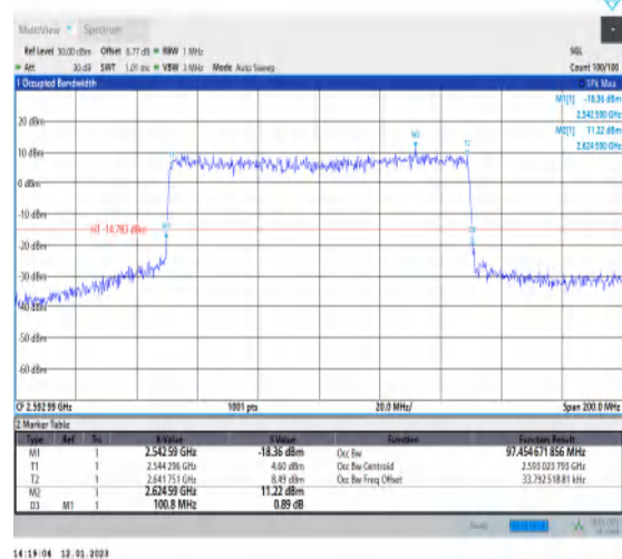
1-N41-PC3-30-100-M-6-CP-QPSK-Outet_Full-273@ 0-Ant1-97.455-100.800-≤100-PASS
