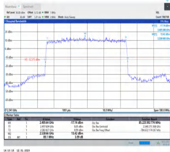
1-N41-PC3-30-90-L-2-DFT-PI2BPSK-Outer_Full-240 @0-Ant1-85.223-89.100-≤90-PASS
