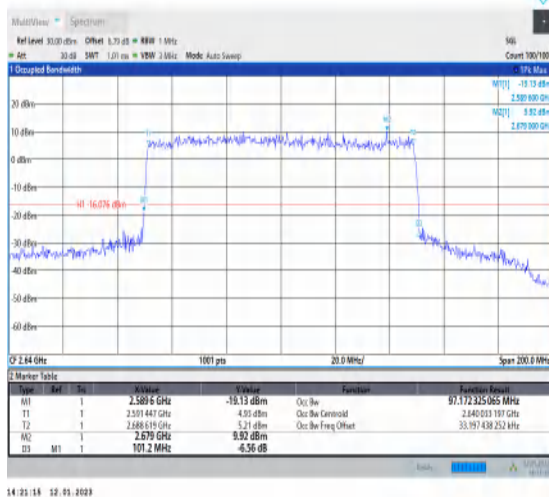
1-N41-PC3-30-100-H-8-CP-64QAM-Outer_Full-273 @0-Ant1-97.172-101.200≤100-PASS
