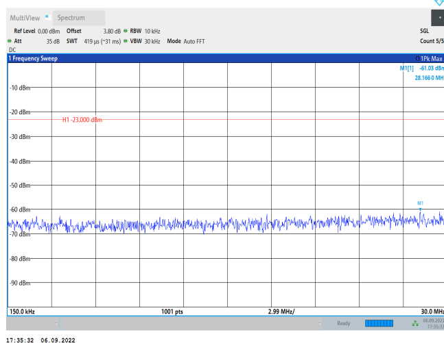
Band5-10MHz-QPSK-20450-1RB#0-Range2:0.15~30MHz
