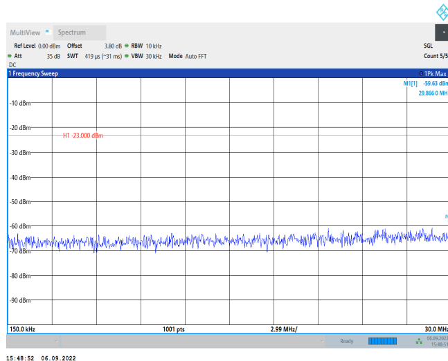
Band26-15MHz-QPSK-26865-1RB#0-Range2:0.15~30MHz
