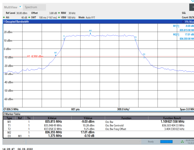
Band26-1.4MHz-QPSK-26915-6RB#0
