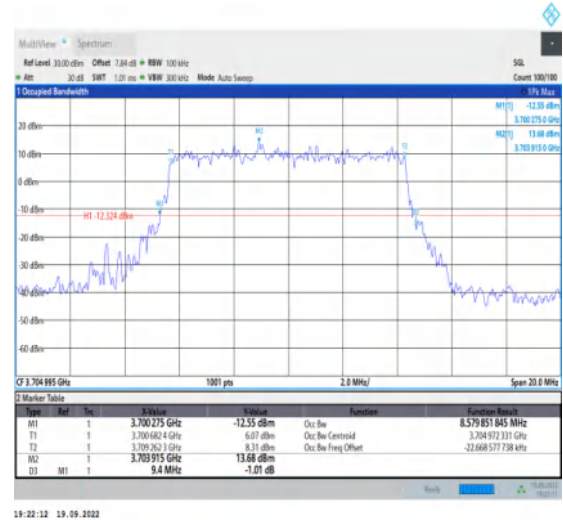
1-N77-3700-3980--30-10-L-4-DFT-64QAM-Outer_Full I-24@0-Ant1-8.58-9.400≤10-PASS
