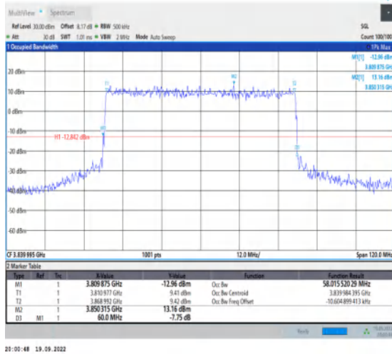
1-N77-3700-3980--30-60-M-1-DFT-QPSK-Outet_Ful I-162@0-Ant1-58.016-60.000-≤60-PASS
