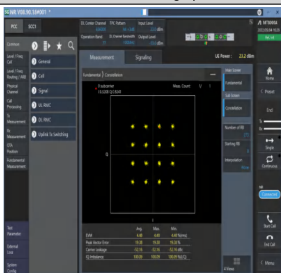
1-N77-3700-3980--30-100-M-7-CP-16QAM-Outer_Fu II-273@0-Ant1-see graph-PASS
