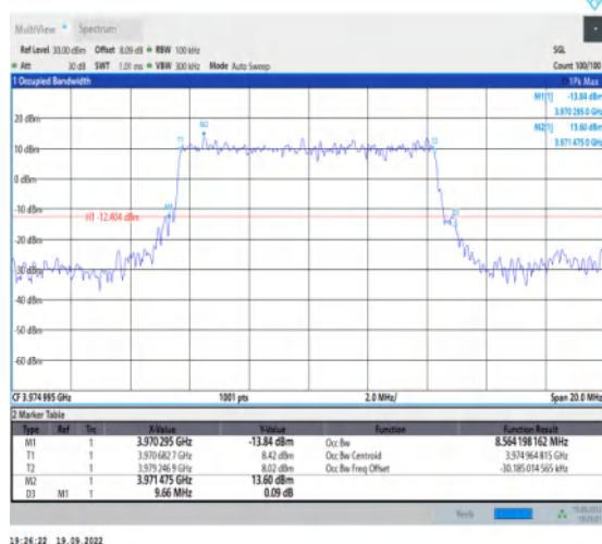
1-N77-3700-3980--30-10-H-2-DFT-PI2BPSK-Outer_F ull-24@0-Ant1-8.564-9.660-≤10-PASS
