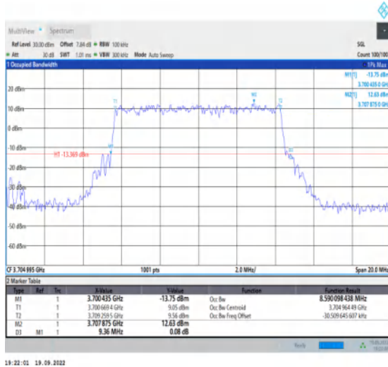
1-N77-3700-3980--30-10-L-3-DFT-16QAM-Outer_Full I-24@0-Ant1-8.59-9.360≤10-PASS
