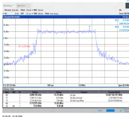
1-N77-3700-3980--30-15-L-7-CP-16QAM-Outet_Full-38@0-Ant1-13.567-15.000-≤15-PASS
