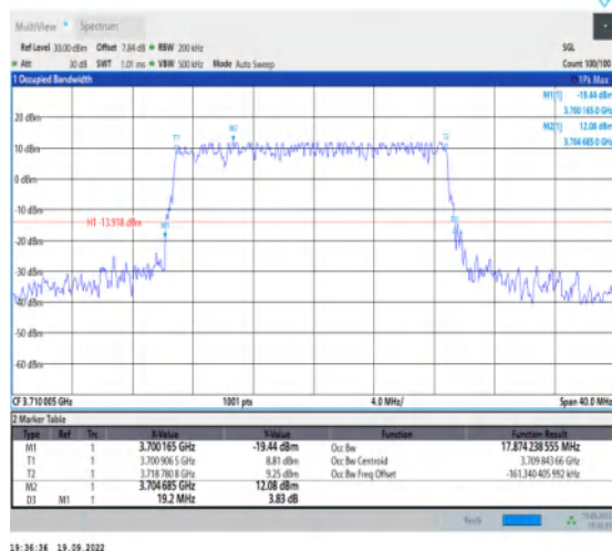
1-N77-3700-3980--30-20-L-4-DFT-64QAM-Outer_Ful I-50@0-Ant1-17.874-19.200-≤20-PASS
