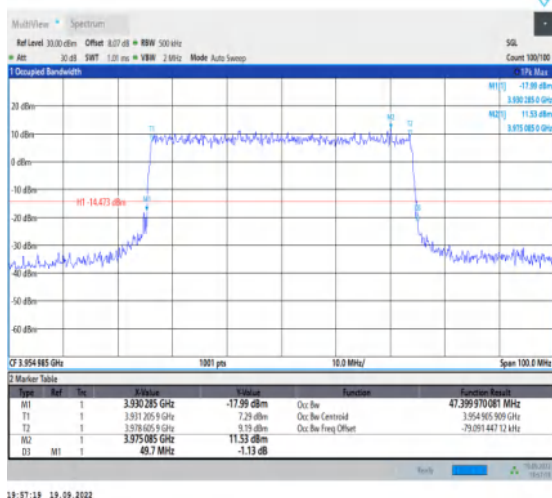
1-N77-3700-3980--30-50-H-7-CP-16QAM-Outer_Full I-133@0-Ant1-47.4-49.700-≤50-PASS
