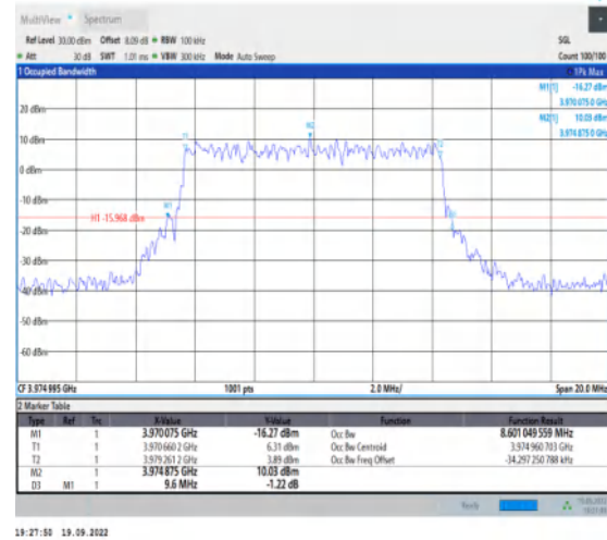
1-N77-3700-3980--30-10-H-8-CP-64QAM-Outer_Full -24@0-Ant1-8.601-9.600-≤10-PASS
