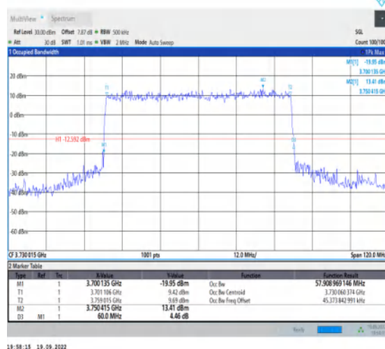
1-N77-3700-3980--30-60-L-1-DFT-QPSK-Outer_Full 162@0-Ant1-57.909-60.000-≤60-PASS
