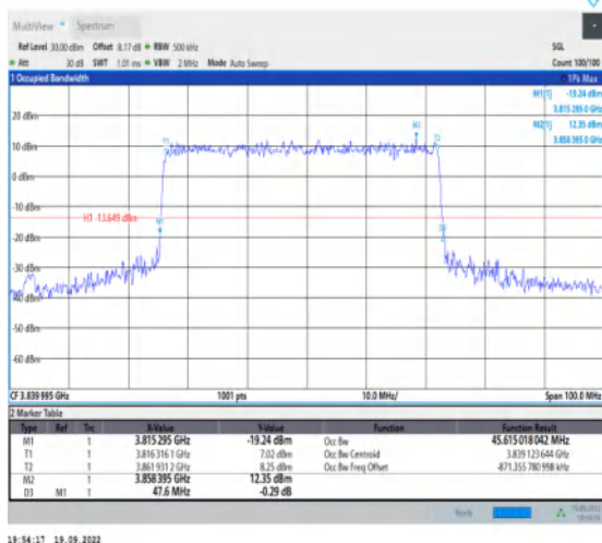
1-N77-3700-3980--30-50-M-4-DFT-64QAM-Outer_Full-128@0-Ant1-45.615-47.600-≤50-PASS
