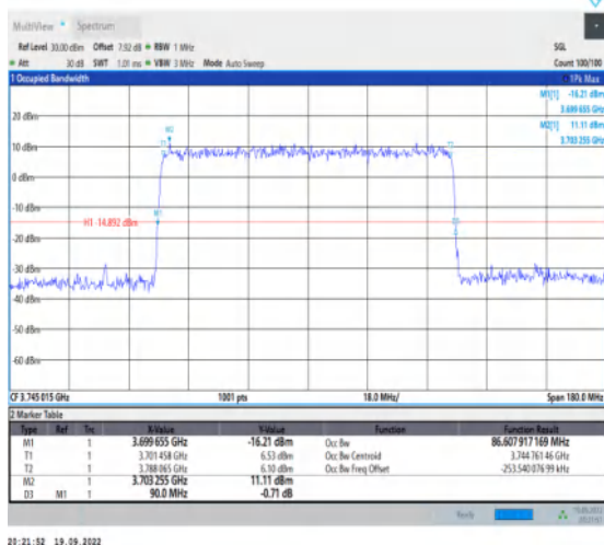
1-N77-3700-3980--30-90-L-5-DFT-256QAM-Outer_Full-243@0-Ant1-86.608-90.000-≤90-PASS
