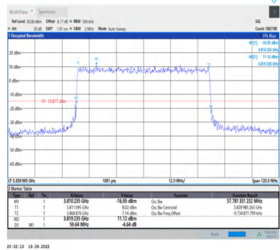
1-N77-3700-3980--30-60-M-6-CP-QPSK-Outer_Full-162@0-Ant1-57.781-59.640-≤60-PASS
