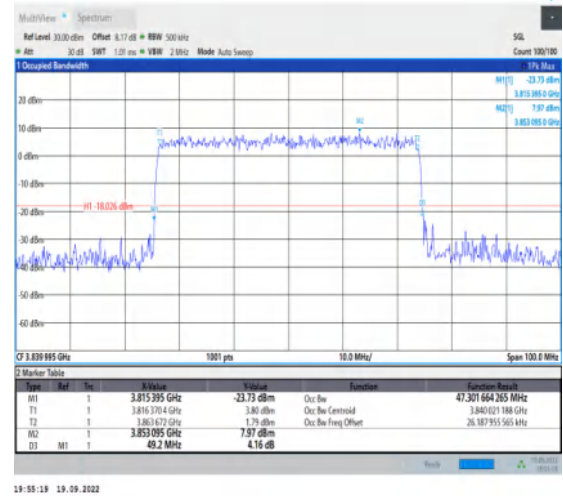
1-N77-3700-3980--30-50-M-9-CP-256QAM-Outer_Fu II-133@0-Ant1-47.302-49.200-≤50-PASS
