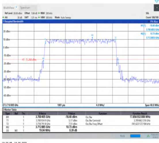
1-N77-3700-3980--30-20-L-5-DFT-256QAM-Outer_F ull-50@0-Ant1-17.857-19.040-≤20-PASS
