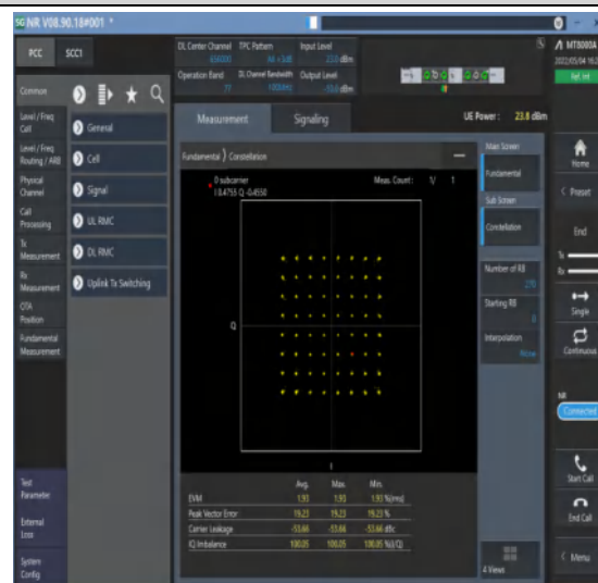
1-N77-3700-3980--30-100-M-4-DFT-64QAM-Outer_Full-270@0-Ant1-see graph-PASS
