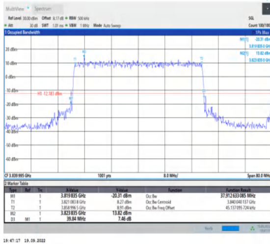
1-N77-3700-3980--30-40-M-7-CP-16QAM-Outer_Ful I-106@0-Ant1-37.913-39.840-≤40-PASS
