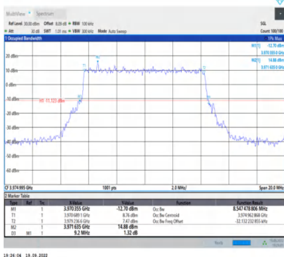
1-N77-3700-3980--30-10-H-1-DFT-QPSK-Outer_Full -24@0-Ant1-8.547-9.200-≤10-PASS
