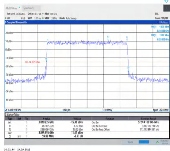
1-N77-3700-3980--30-60-M-4-DFT-64QAM-Outet_Full-162@0-Ant1-57.914-59.880-≤60-PASS
