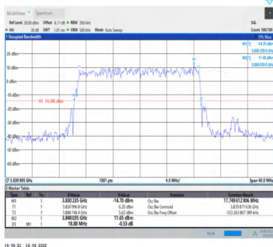
1-N77-3700-3980--30-20-M-5-DFT-256QAM-Outer_Full-50@0-Ant1-17.75-18.880-≤20-PASS
