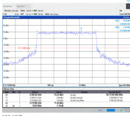
1-N77-3700-3980--30-20-L-6-CP-QPSK-Outer_Full-5 1@0-Ant1-18.175-18.920-≤20-PASS
