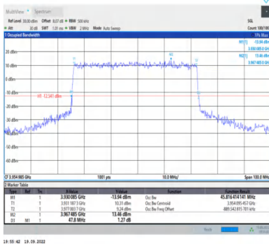
1-N77-3700-3980--30-50-H-1-DFT-QPSK-Outer_Full -128@0-Ant1-45.816-47.800-≤50-PASS
