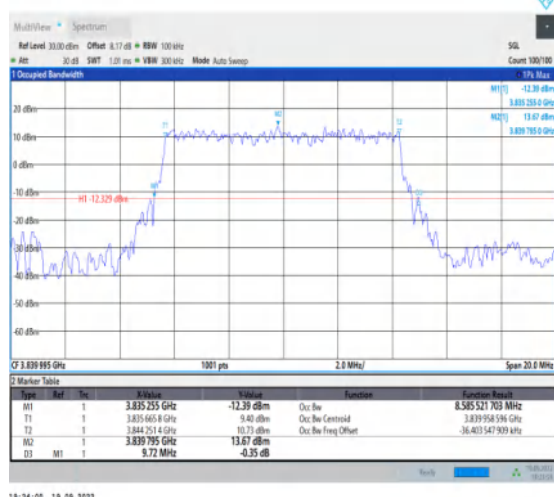
1-N77-3700-3980--30-10-M-2-DFT-PI2BPSK-Outer_Full-24@0-Ant1-8.586-9.720-≤10-PASS
