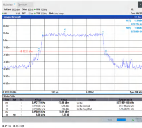
1-N77-3700-3980--30-10-H-7-CP-16QAM-Outer_Full I-24@0-Ant1-8.576-9.580-≤10-PASS
