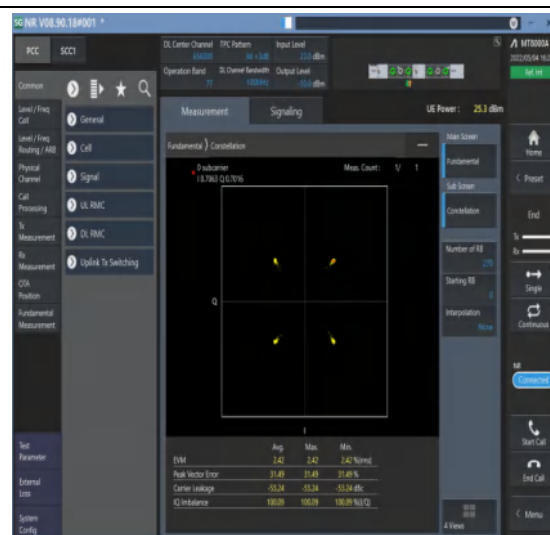
1-N77-3700-3980--30-100-M-2-DFT-QPSK-Outer_Full-270@0-Ant1-see graph-PASS
