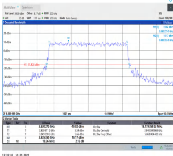
1-N77-3700-3980--30-20-M-6-CP-QPSK-Outet_Full-51@0-Ant1-18.179-19.360-≤20-PASS
