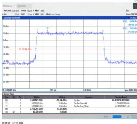
1-N77-3700-3980--30-80-L-6-CP-QPSK-Outer_Full-217@0-Ant1-77.42-80.640-≤80-PASS
