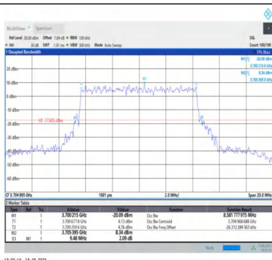
1-N77-3700-3980--30-10-L-9-CP-256QAM-Outer_Full-24@0-Ant1-8.582-9.480-≤10-PASS
