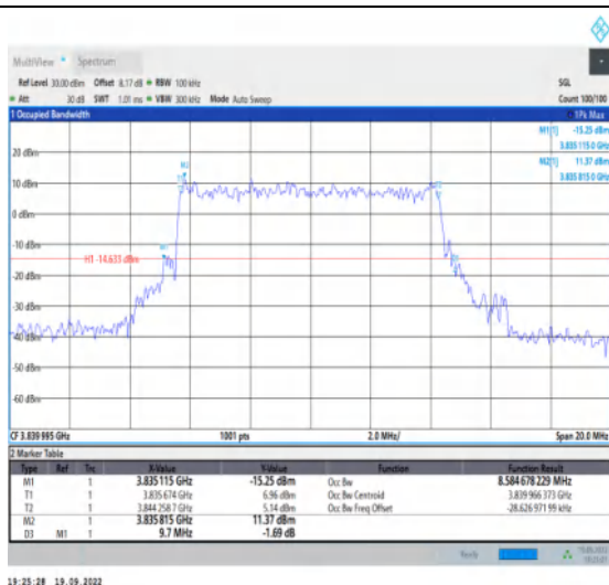
1-N77-3700-3980--30-10-M-8-CP-64QAM-Outer_Ful I-24@0-Ant1-8.585-9.700-≤10-PASS
