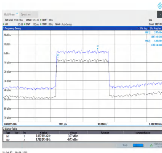
1-N77-3700-3980--30-100-M-1-DFT-256QAM-Outer_Full-270@0-Ant1-9.92-100%-0.00-9.92-PASS-≤13
