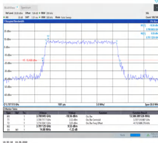
1-N77-3700-3980--30-15-L-9-CP-256QAM-Outet_Full-38@0-Ant1-13.586-14.880-≤15-PASS
