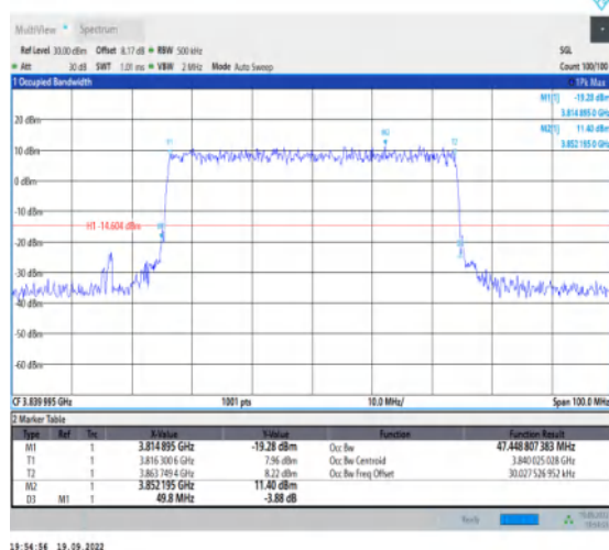
1-N77-3700-3980--30-50-M-7-CP-16QAM-Outer_Full-133@0-Ant1-47.449-49.800-≤50-PASS
