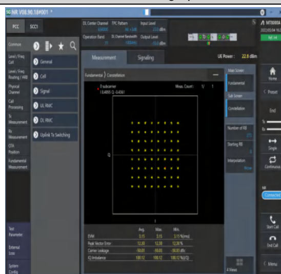
1-N77-3700-3980--30-100-M-8-CP-64QAM-Outer_F ull-273@0-Ant1-see graph-PASS
