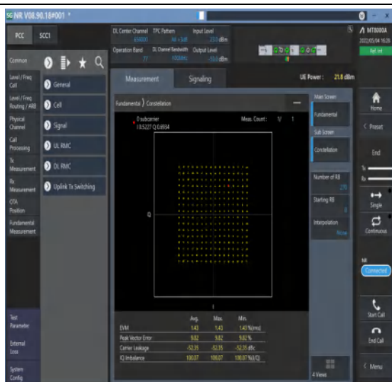
1-N77-3700-3980--30-100-M-5-DFT-256QAM-Outer_Fu Full-270@0-Ant1-see graph-PASS
