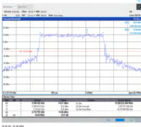
1-N77-3700-3980--30-15-L-8-CP-64QAM-Outet_Full-38@0-Ant1-13.584-14.640-≤15-PASS
