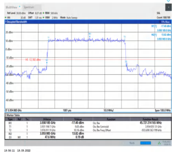
1-N77-3700-3980--30-50-H-2-DFT-PI2BPSK-Outer_F ull-128@0-Ant1-45.721-47.600-≤50-PASS
