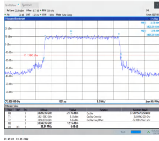
1-N77-3700-3980--30-40-M-8-CP-64QAM-Outer_Full -106@0-Ant1-37.788-39.840-≤40-PASS
