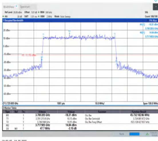
1-N77-3700-3980--30-50-L-1-DFT-QPSK-Outer_Full -128@0-Ant1-45.732-47.700-≤50-PASS
