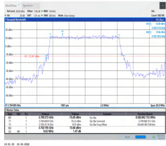
1-N77-3700-3980--30-10-L-2-DFT-PI2BPSK-Outer_Full -24@0-Ant1-8.583-9.620≤10-PASS
